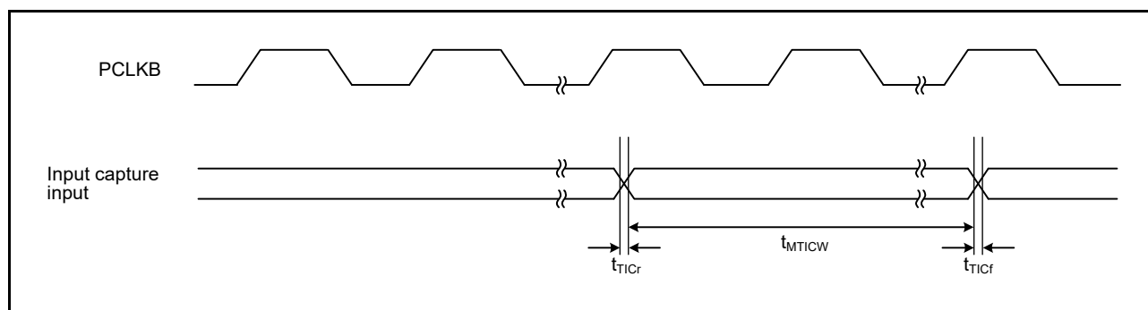
Figure 2.20 MTU Input/Output Timing
