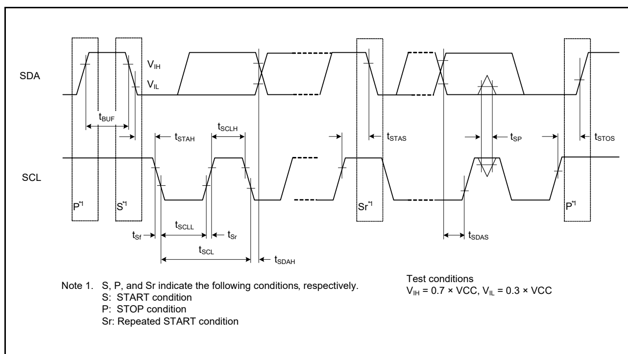
Figure 2.48 IIC Bus Interface Input/Output Timing
