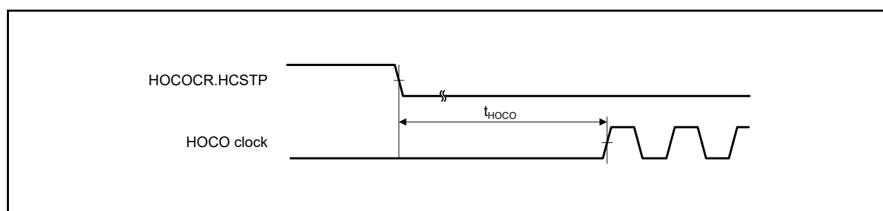
Figure 2.11 HOCO Clock Oscillation Start Timing (Oscillation is Started by Setting HOCOCR.HCSTP Bit)
