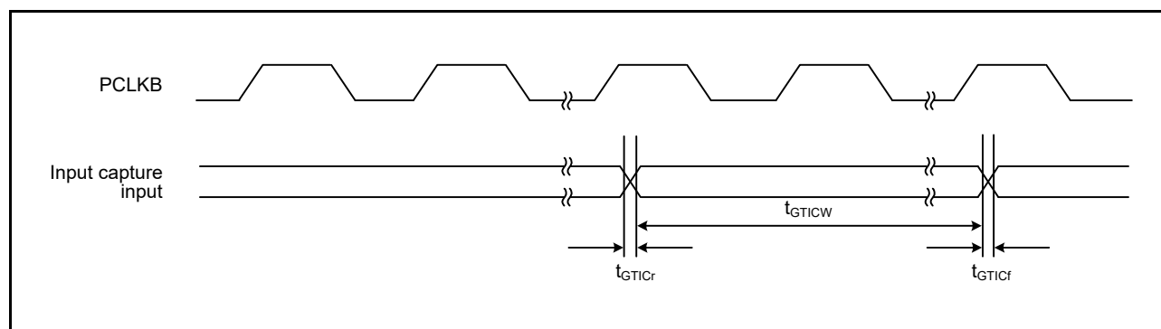
Figure 2.36 GPTW Input Capture Input Timing
