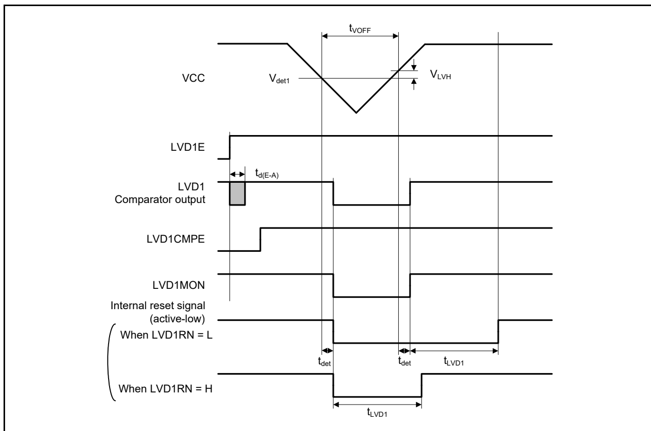
Figure 2.57 Voltage Detection Circuit Timing ( V_{det1} )
