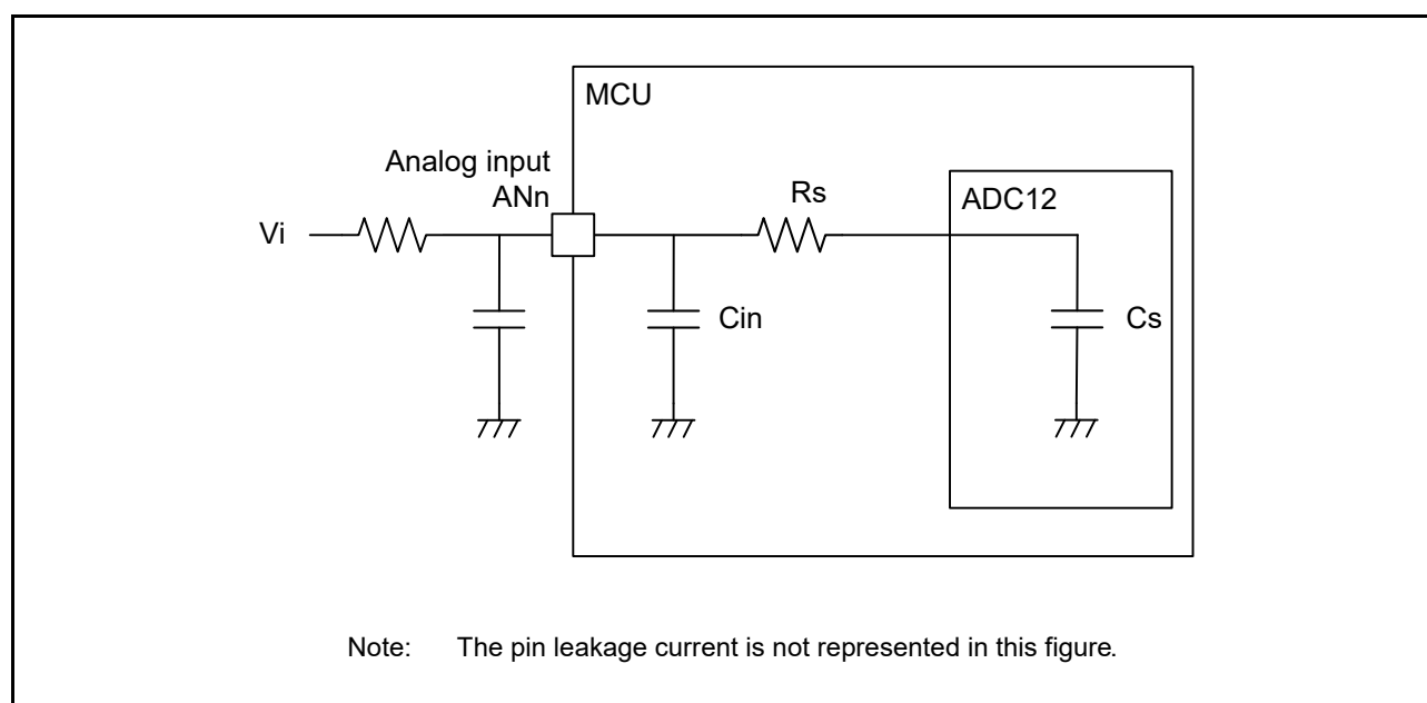
Figure 2.51 Equivalent Circuit of an Analog Input
