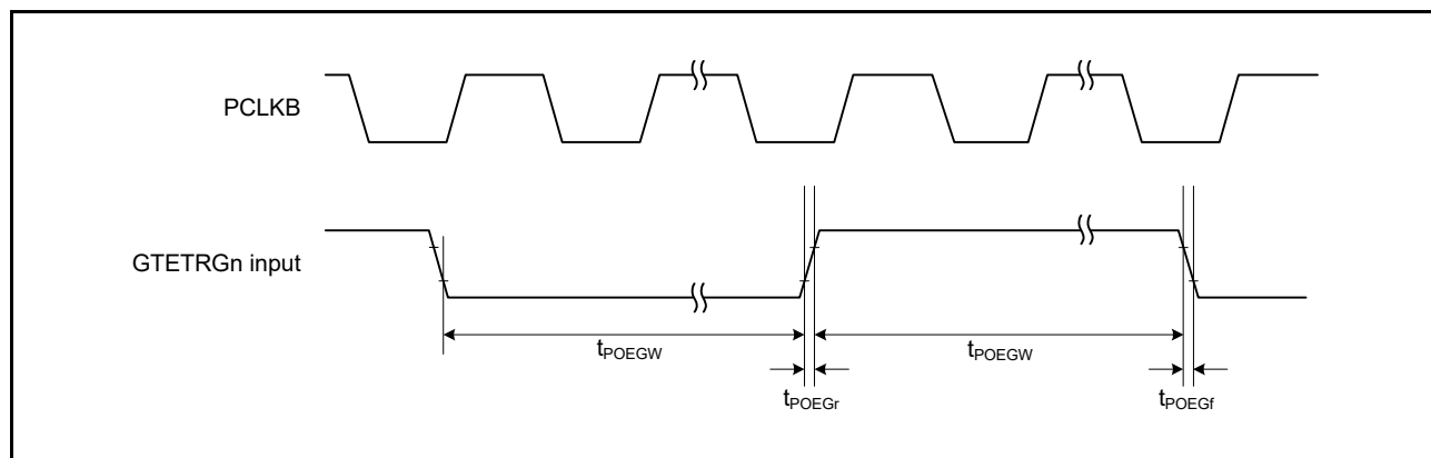
Figure 2.28 POEG Input Timing (n = A)
