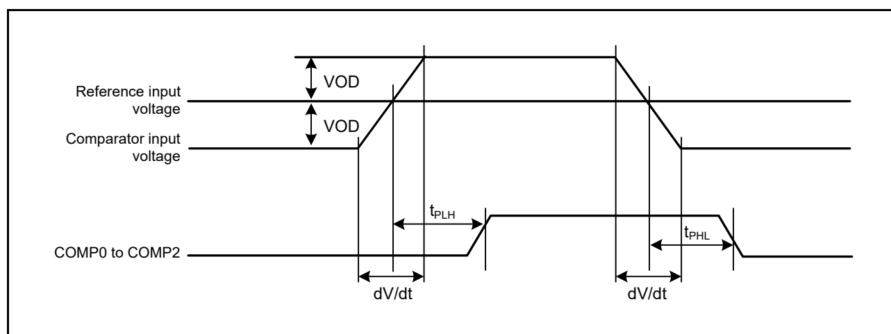
Figure 2.53 Comparator Response Time
