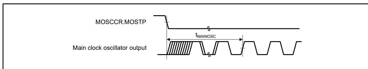
Figure 2.7 Main Clock Oscillation Start Timing
