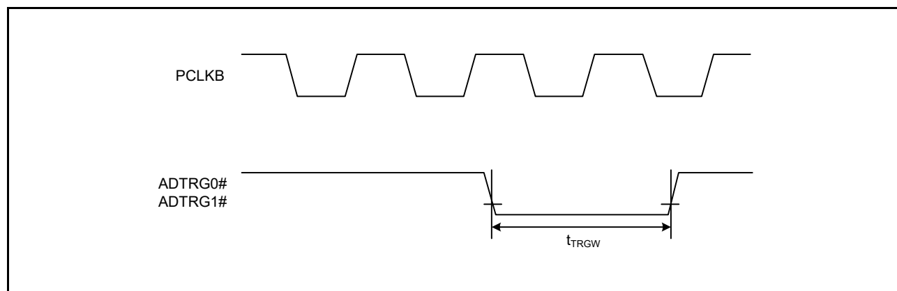
Figure 2.49 A/D Converter External Trigger Input Timing
