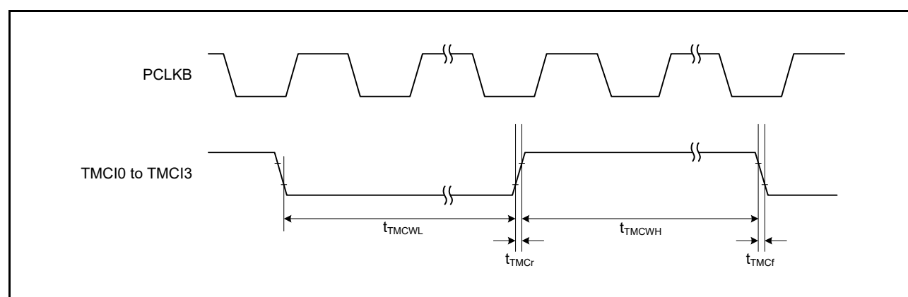
Figure 2.39 TMR Clock Input Timing
