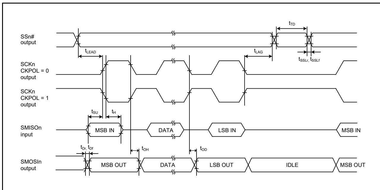
Figure 2.44 Simple SPI Timing (Master, CKPH = 1) ( n = 1, 5, 6, 12 )
