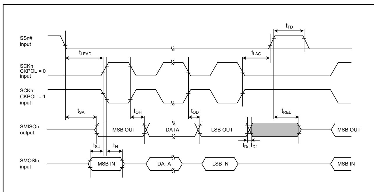
Figure 2.46 Simple SPI Clock Timing (Slave, CKPH = 1) (n = 1, 5, 6, 12)
