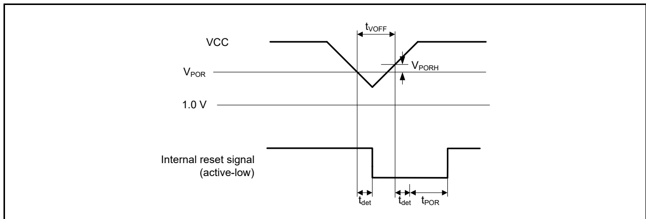
Figure 2.54 Voltage Detection Reset Timing
