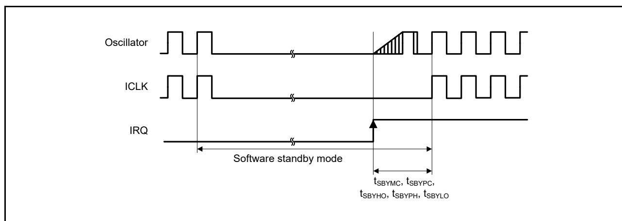
Figure 2.15 Software Standby Mode Recovery Timing
