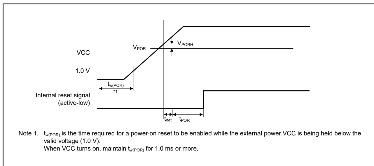
Figure 2.55 Power-On Reset Timing
