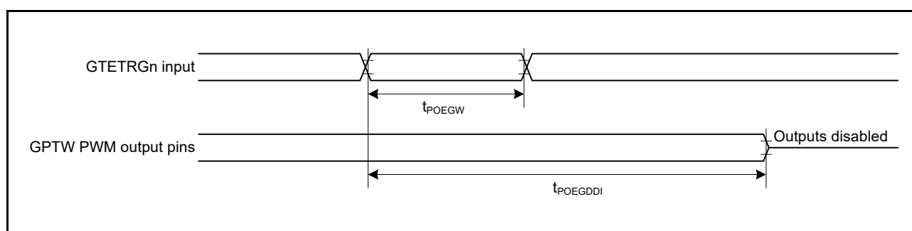
Figure 2.34 Output Disable Time for POEG in Direct Response to the Input Level Detection of the GTETRn pin ( n = A )
