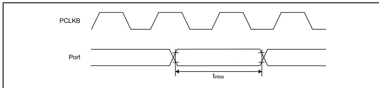
Figure 2.19 I/O Port Input Timing
