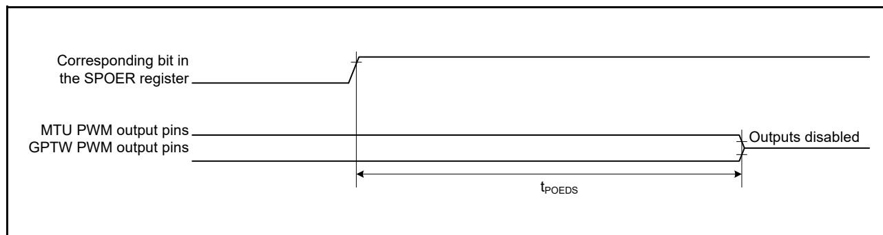
Figure 2.26 Output Disable Time for POE in Response to the Register Setting
