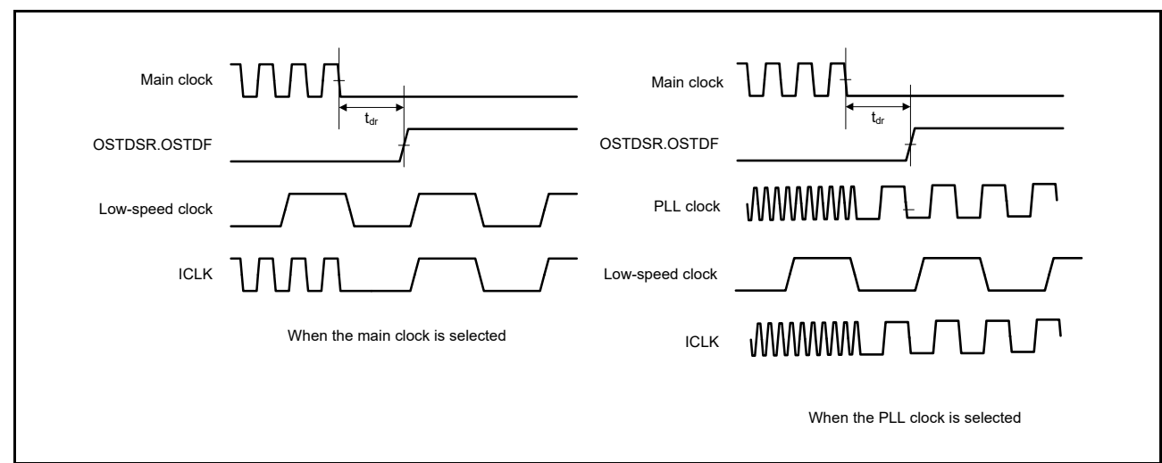
Figure 2.59 Oscillation Stop Detection Timing
