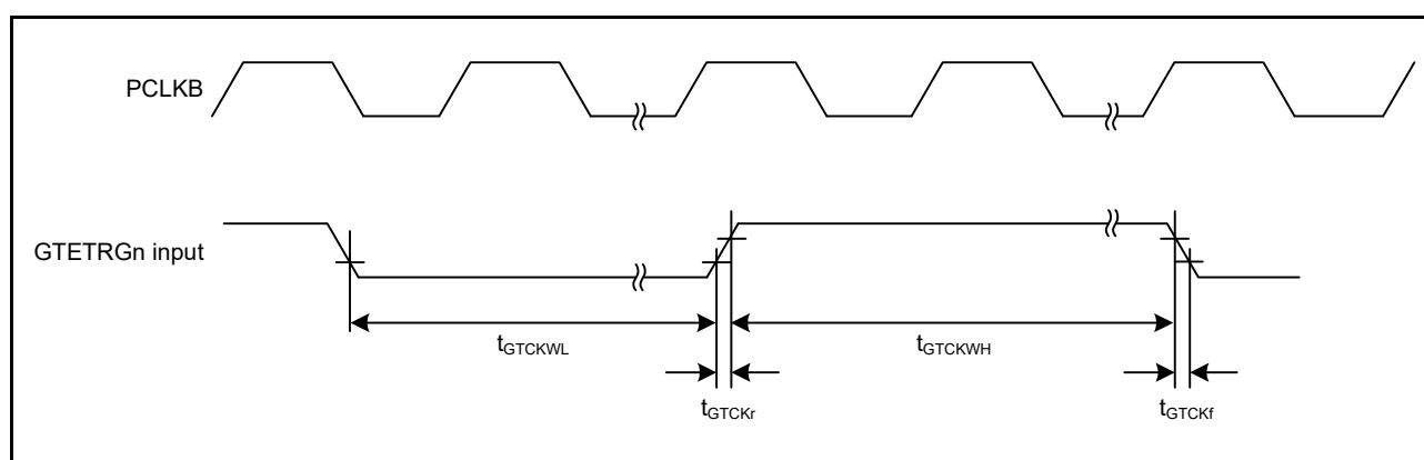
Figure 2.38 GPTW Clock Input Timing (n = A)
