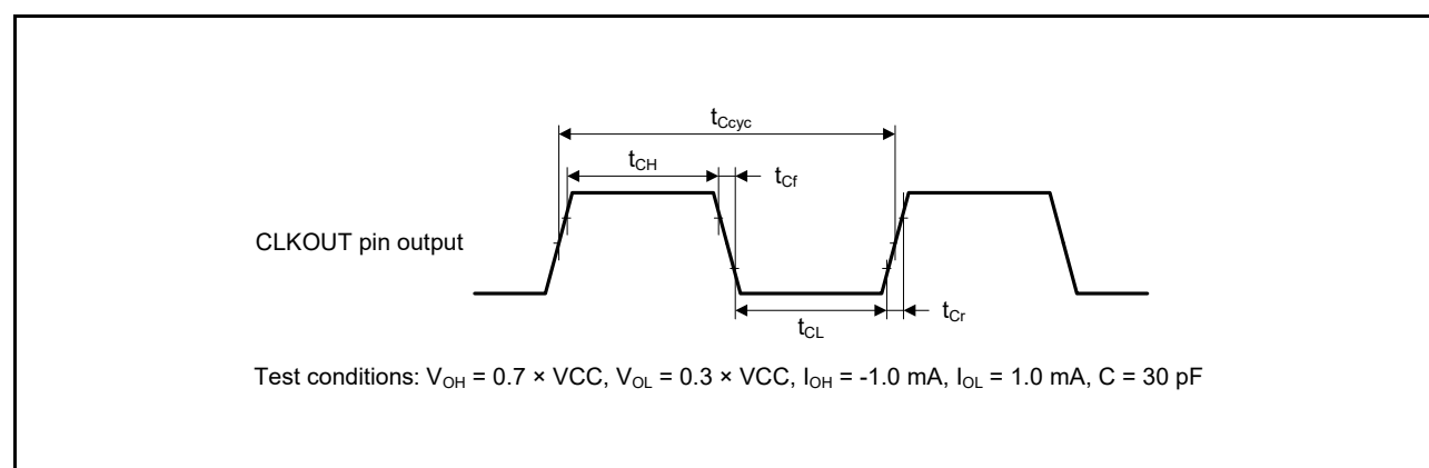
Figure 2.50 CLKOUT Output Timing
