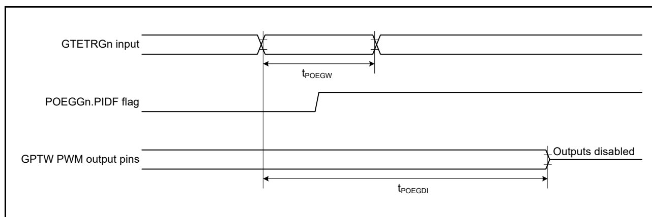
Figure 2.29 Output Disable Time for POEG via Detection Flag in Response to the Input Level Detection of the GTETRn pin ( n = A )
