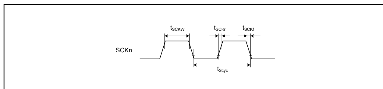
Figure 2.40 SCK Clock Input Timing (n = 1, 5, 6, 12)
