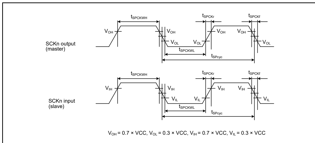
Figure 2.43 Simple SPI Clock Timing (n = 1, 5, 6, 12)
