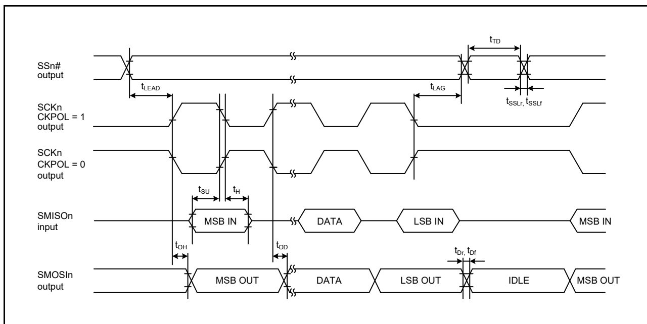
Figure 2.45 Simple SPI Timing (Master, CKPH = 0) ( n = 1, 5, 6, 12 )
