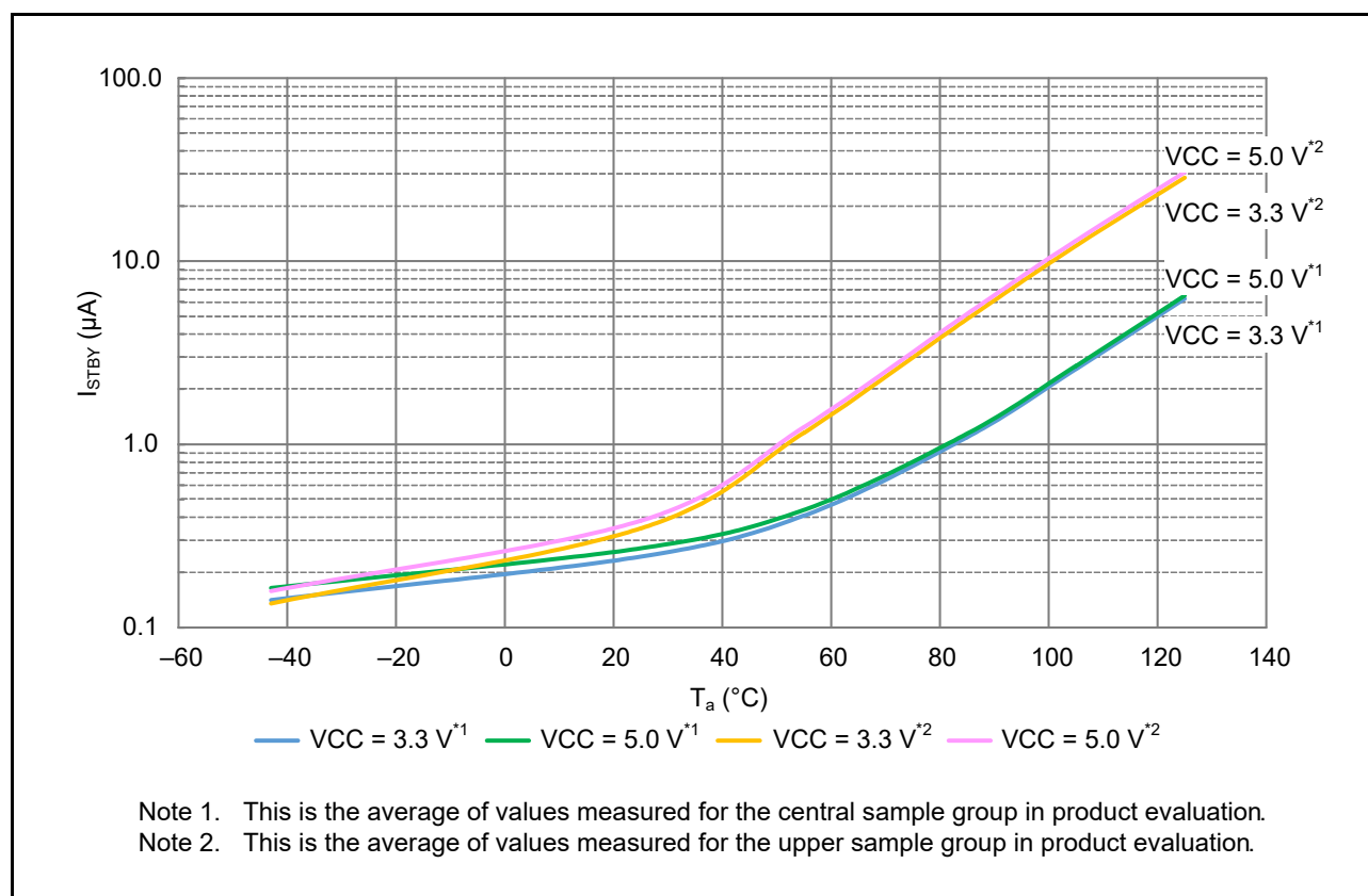
Figure 2.3 Temperature Dependency in Software Standby Mode
