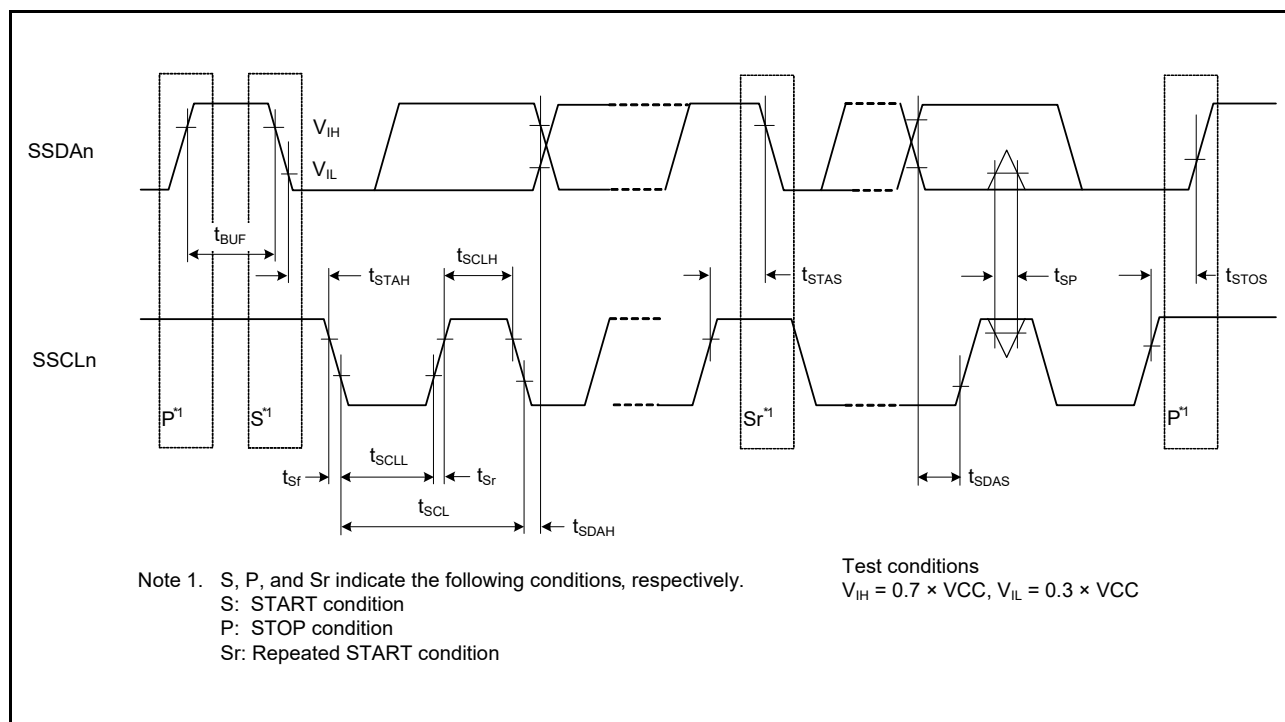
Figure 2.42 Output Timing and Simple I 2 C Bus Interface Input/Output Timing (n = 1, 5, 6, 12)
