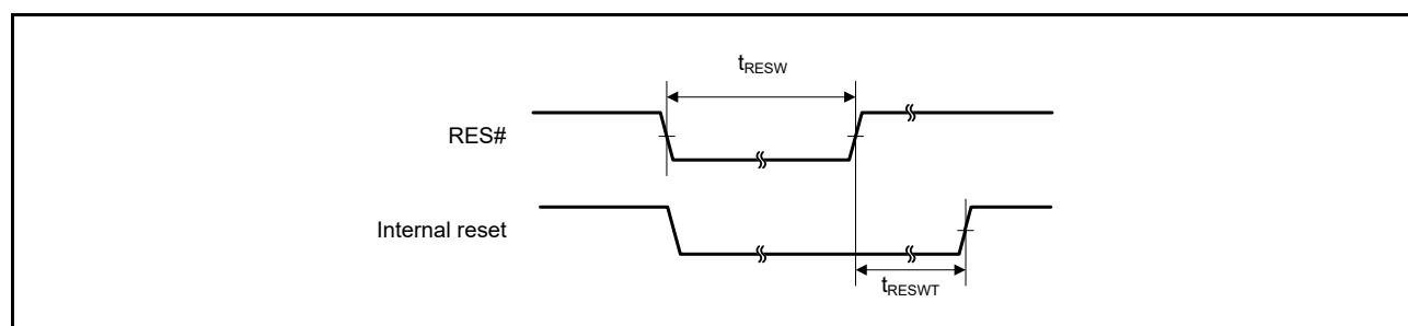
Figure 2.14 Reset Input Timing
