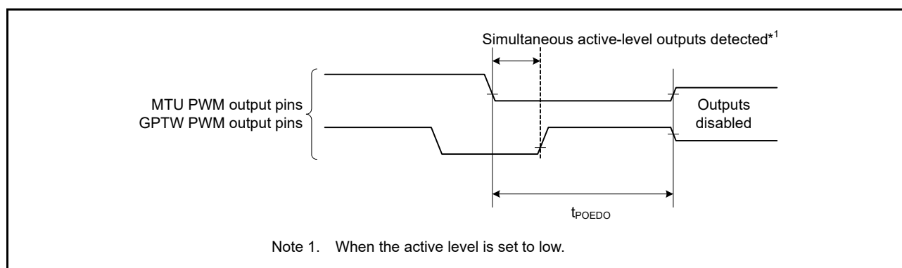
Figure 2.24 Output Disable Time for POE in Response to the Simultaneous Conduction of Output Pins
