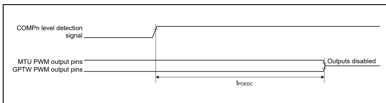
Figure 2.25 Output Disable Time for POE in Response to Detection of the Comparator Outputs (n = 0 to 2)
