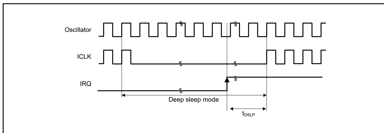
Figure 2.16 Deep Sleep Mode Recovery Timing
