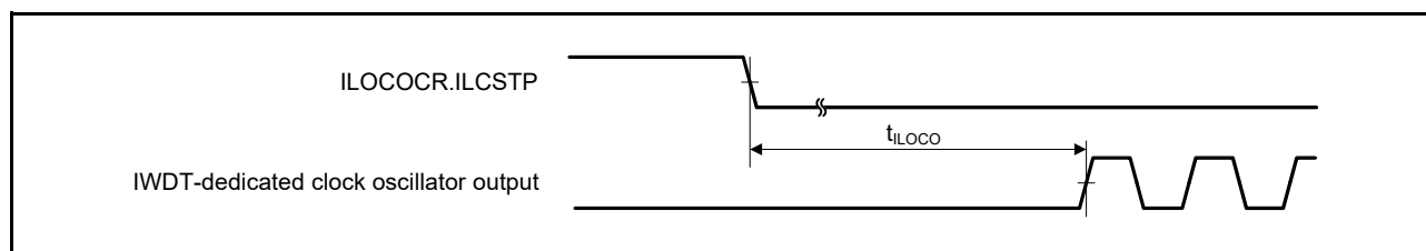
Figure 2.9 IWDT-Dedicated Clock Oscillation Start Timing
