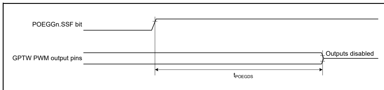
Figure 2.32 Output Disable Time for POEG in Response to the Register Setting ( n = A )
