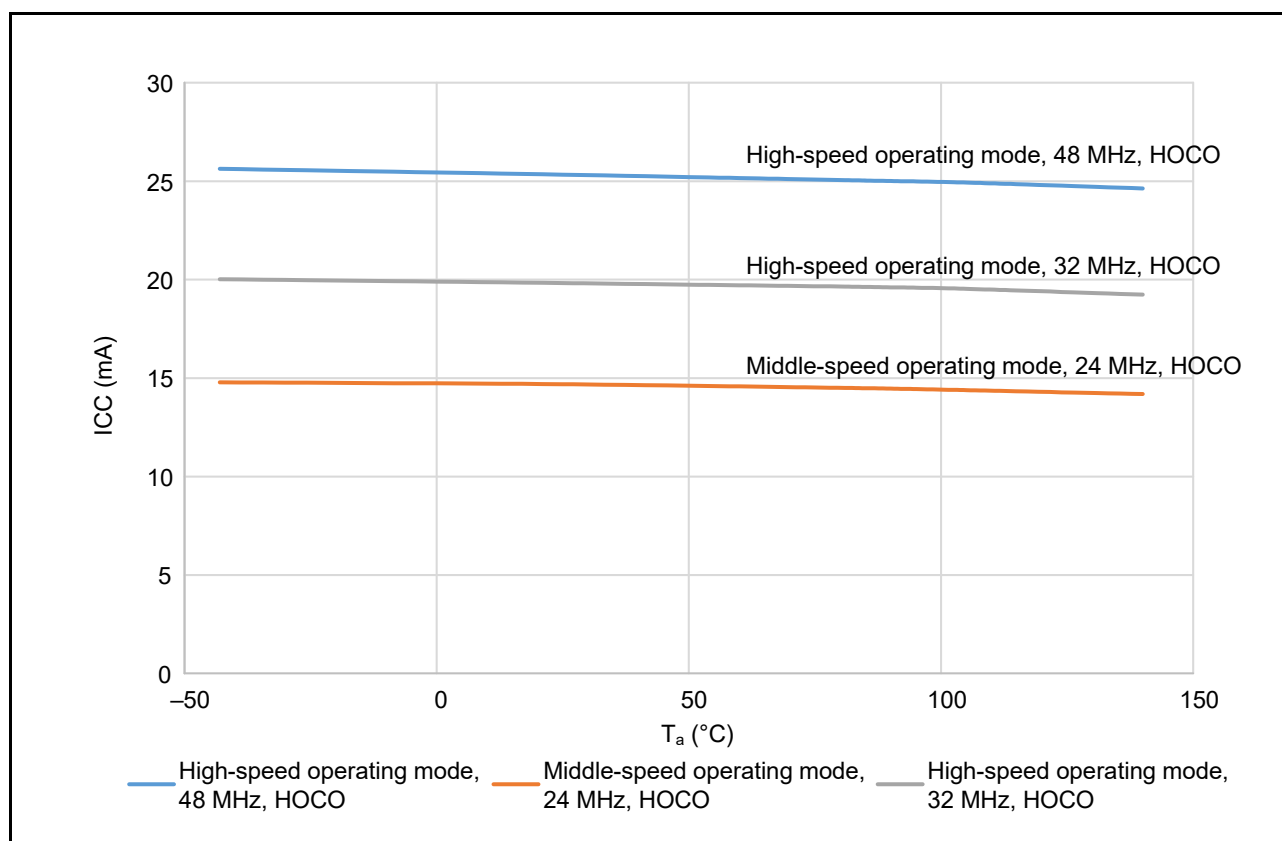
Figure 2.2 Temperature Dependence in the Normal Operating Mode
