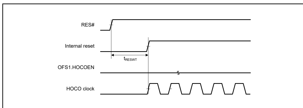
Figure 2.10 HOCO Clock Oscillation Start Timing (After Reset is Canceled by Setting OFS1.HOCOEN Bit to 0)
