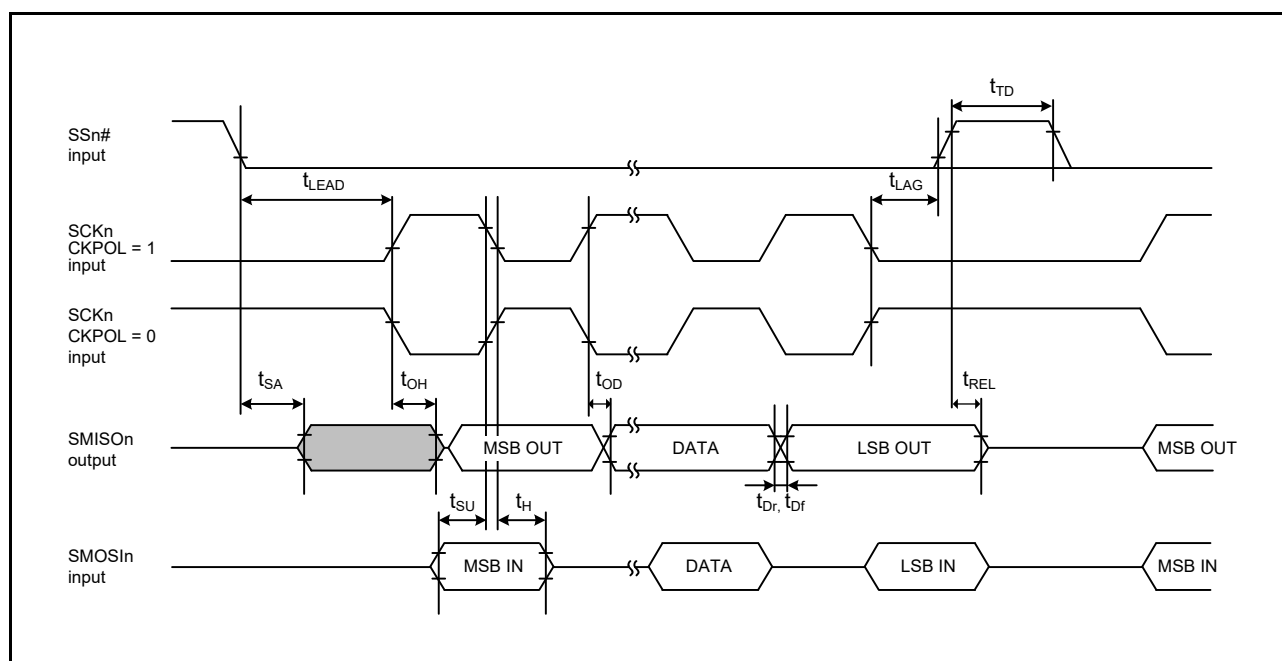
Figure 2.47 Simple SPI Timing (Slave, CKPH = 0) (n = 1, 5, 6, 12)
