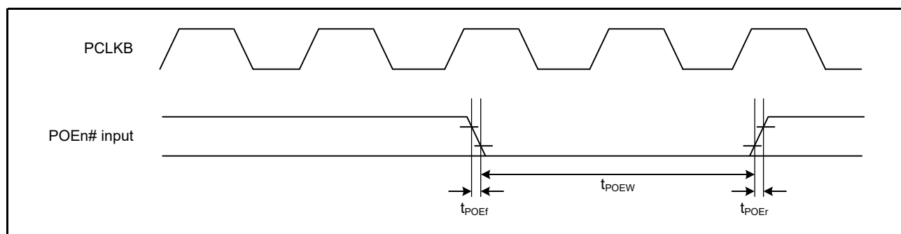
Figure 2.22 POE# Input Timing (n = 0, 8, 10 to 12)
