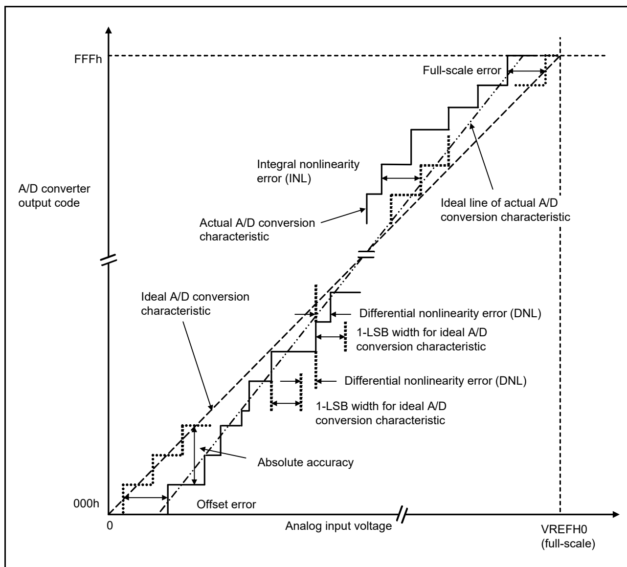
Figure 2.52 Illustration of A/D Converter Characteristic Terms
