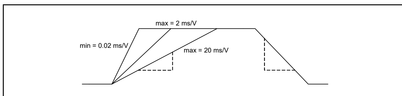
Figure 2.4 VCC Ramp Rate at Power-On
