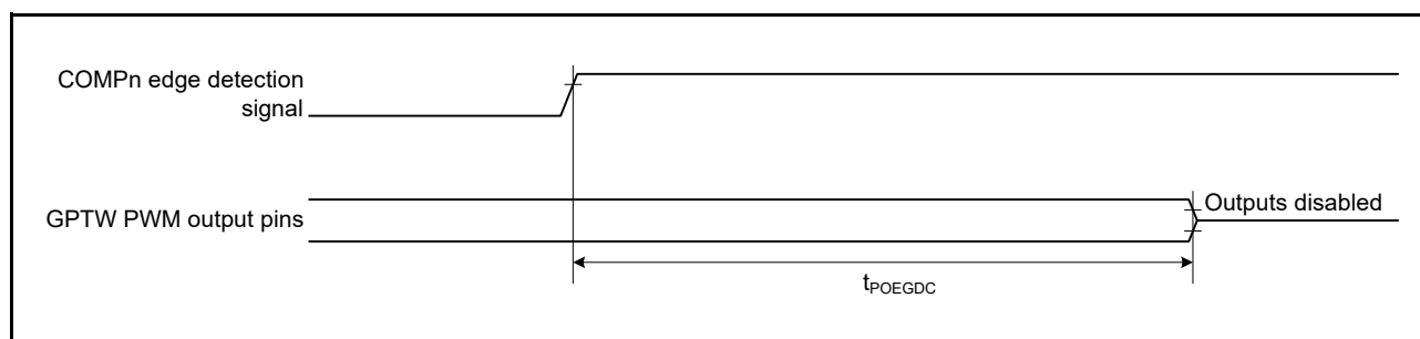
Figure 2.31 Output Disable Time for POEG in Response to Edge Detection Signal from a Comparator ( n = 0 to 2)
