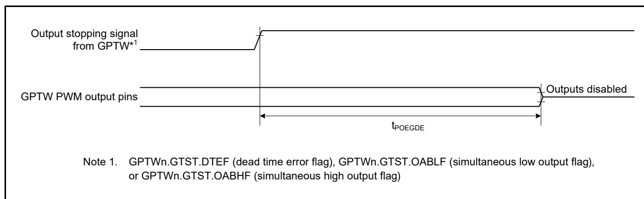
Figure 2.30 Output Disable Time for POEG in Response to Detection of the Output Stopping Signal from GPTW ( n = 0 to 2)
