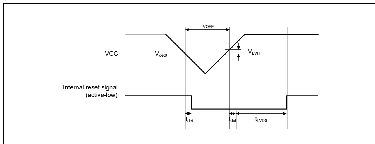
Figure 2.56 Voltage Detection Circuit Timing ( V_{det0} )
