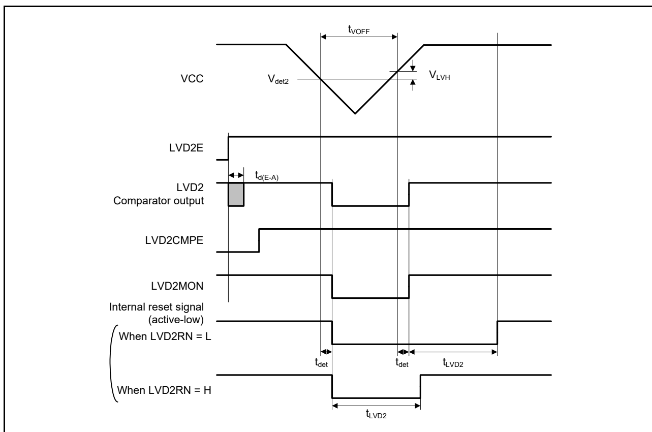
Figure 2.58 Voltage Detection Circuit Timing ( V_{det2} )
