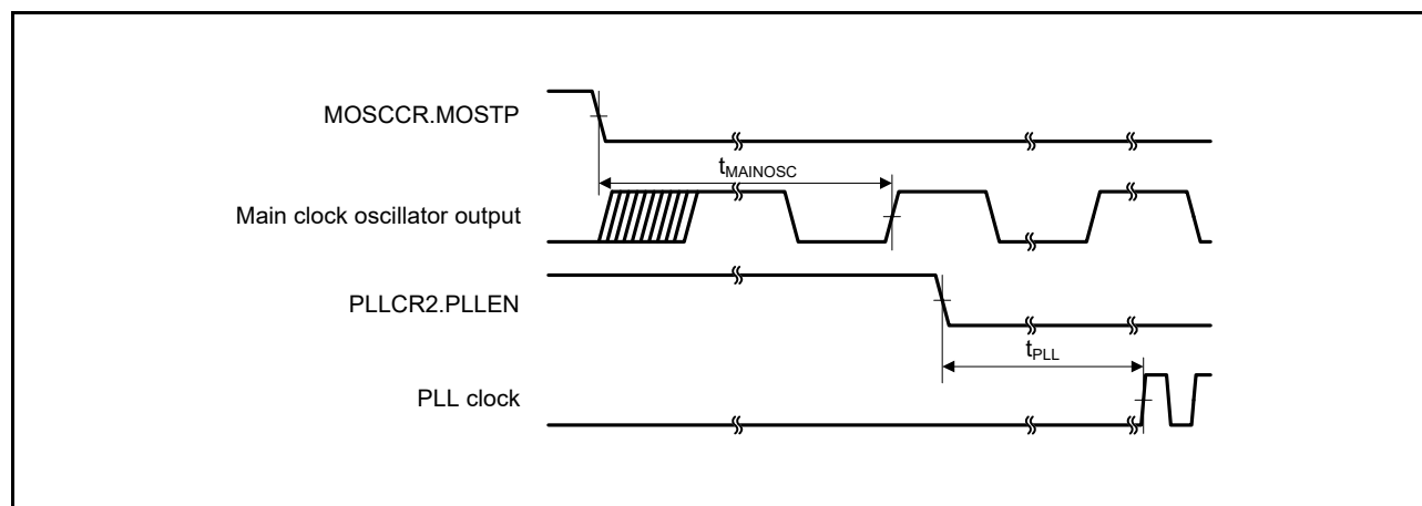
Figure 2.12 PLL Clock Oscillation Start Timing (PLL is Operated after Main Clock Oscillation Has Settled)
