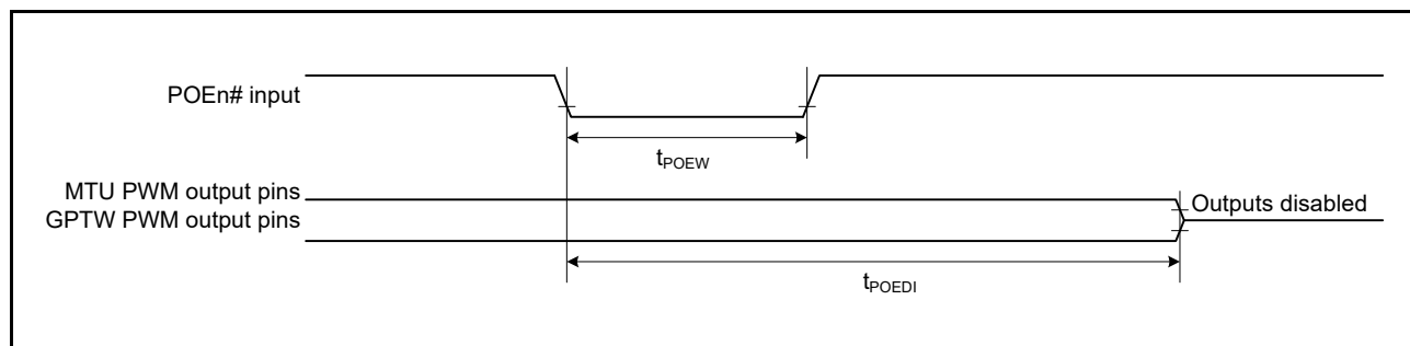
Figure 2.23 Output Disable Time for POE in Response to Transition of the POEn# Signal Level (n = 0, 8, 10 to 12)
