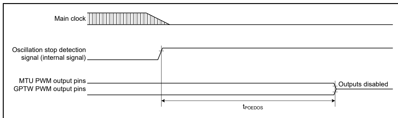
Figure 2.27 Output Disable Time for POE in Response to the Oscillation Stop Detection
