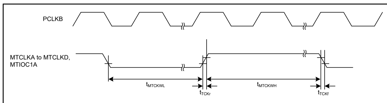
Figure 2.21 MTU Clock Input Timing
