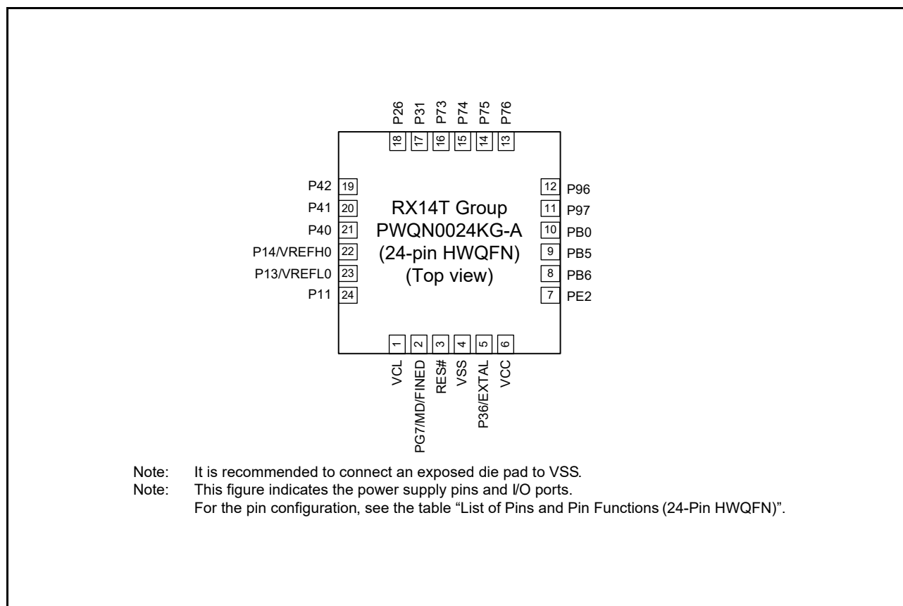
Figure 1.10 Pin Assignments of the 24-Pin HWQFN
