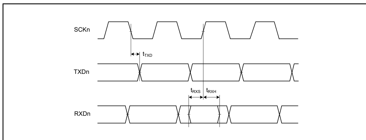
Figure 2.41 SCI Input/Output Timing: Clock Synchronous Mode (n = 1, 5, 6, 12)
