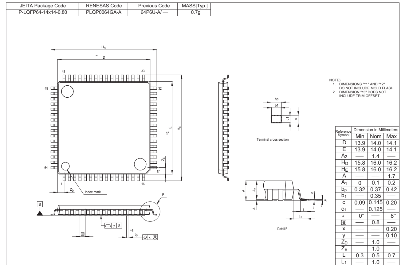
Figure A 64-Pin LQFP (PLQP0064GA-A)
