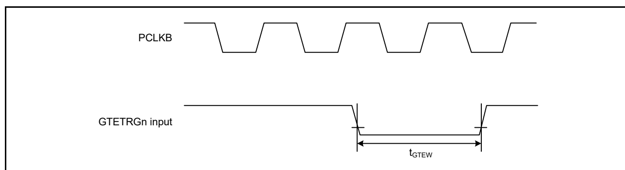
Figure 2.37 GPTW External Trigger Input Timing (n = A)
