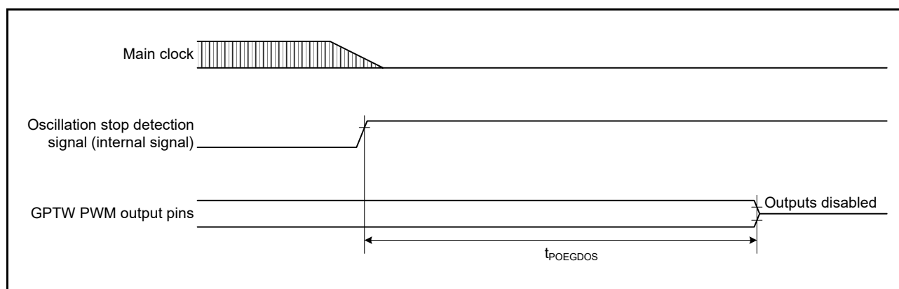
Figure 2.33 Output Disable Time of POEG in Response to the Oscillation Stop Detection
