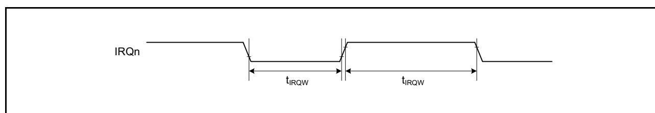
Figure 2.18 IRQ Interrupt Input Timing
