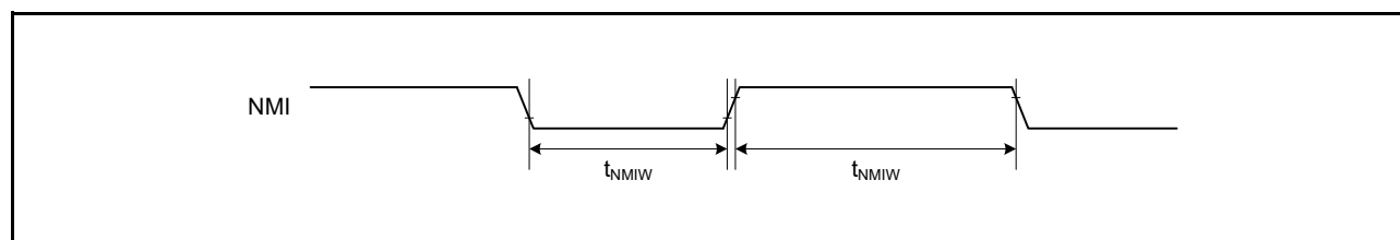
Figure 2.17 NMI Interrupt Input Timing
