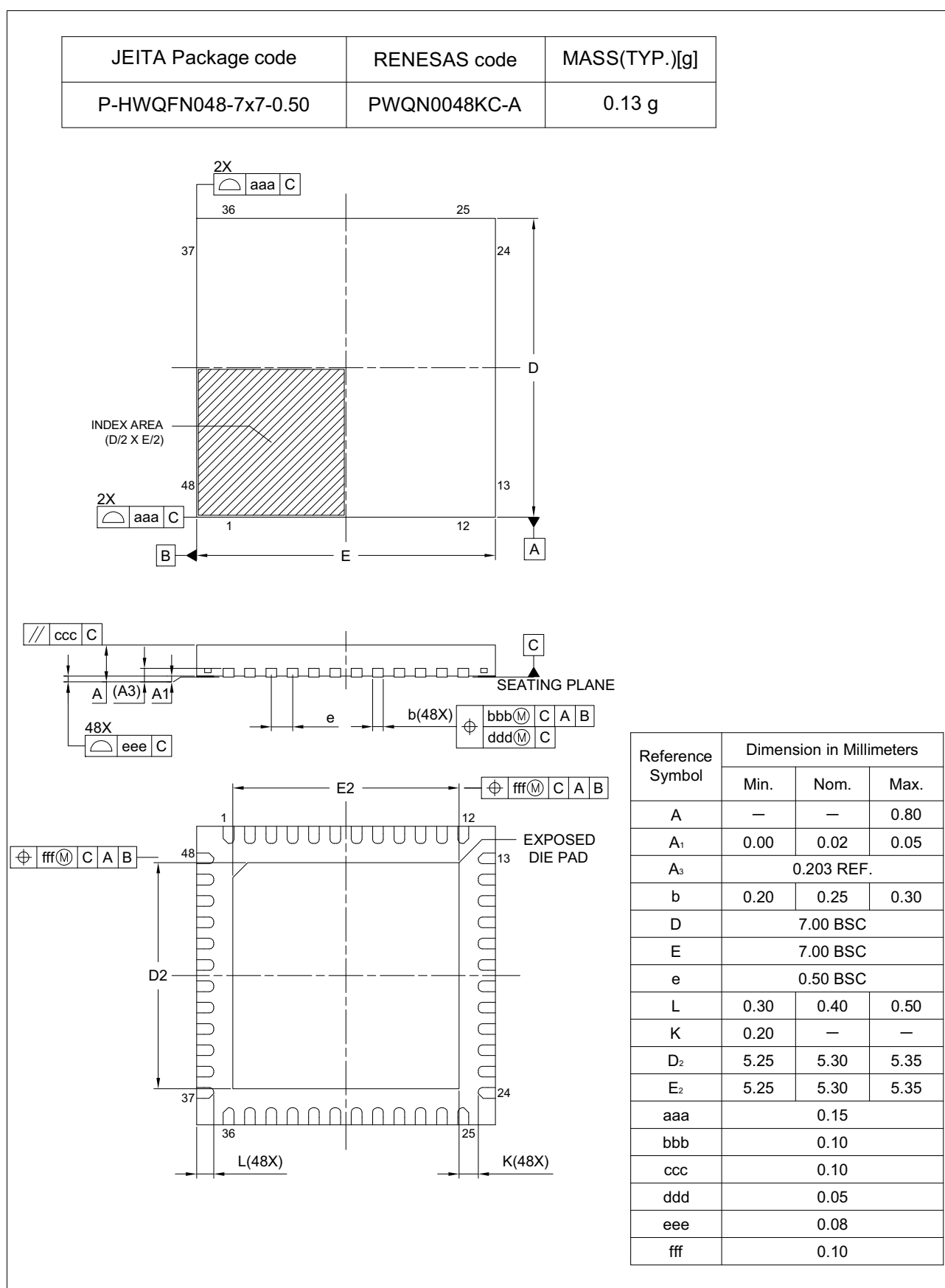
Figure E 48-Pin HWQFN (PWQN0048KC-A)
