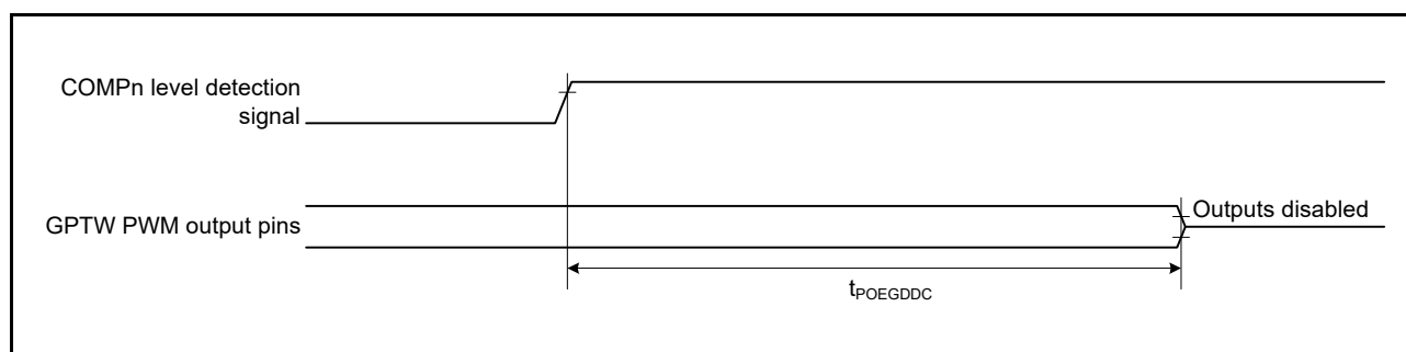
Figure 2.35 Output Disable Time for POEG in Response to Level Detection Signal from a Comparator ( n = 0 to 2)
