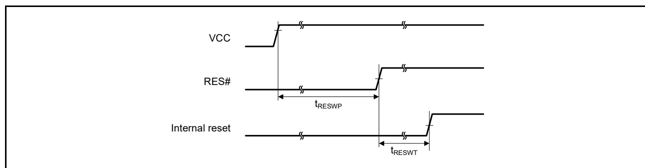
Figure 2.13 Reset Input Timing at Power-On
