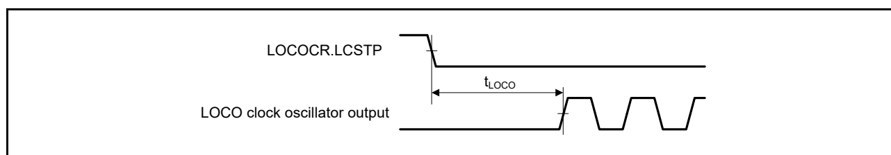
Figure 2.8 LOCO Clock Oscillation Start Timing
