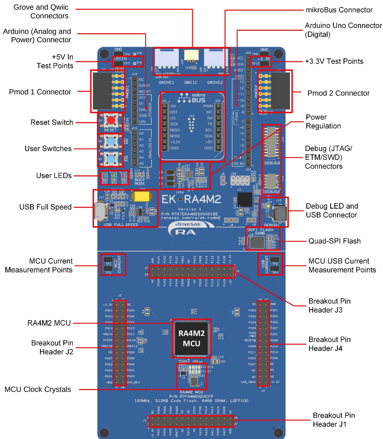
Figure 1. EK-RA4M2 Board Top Side
