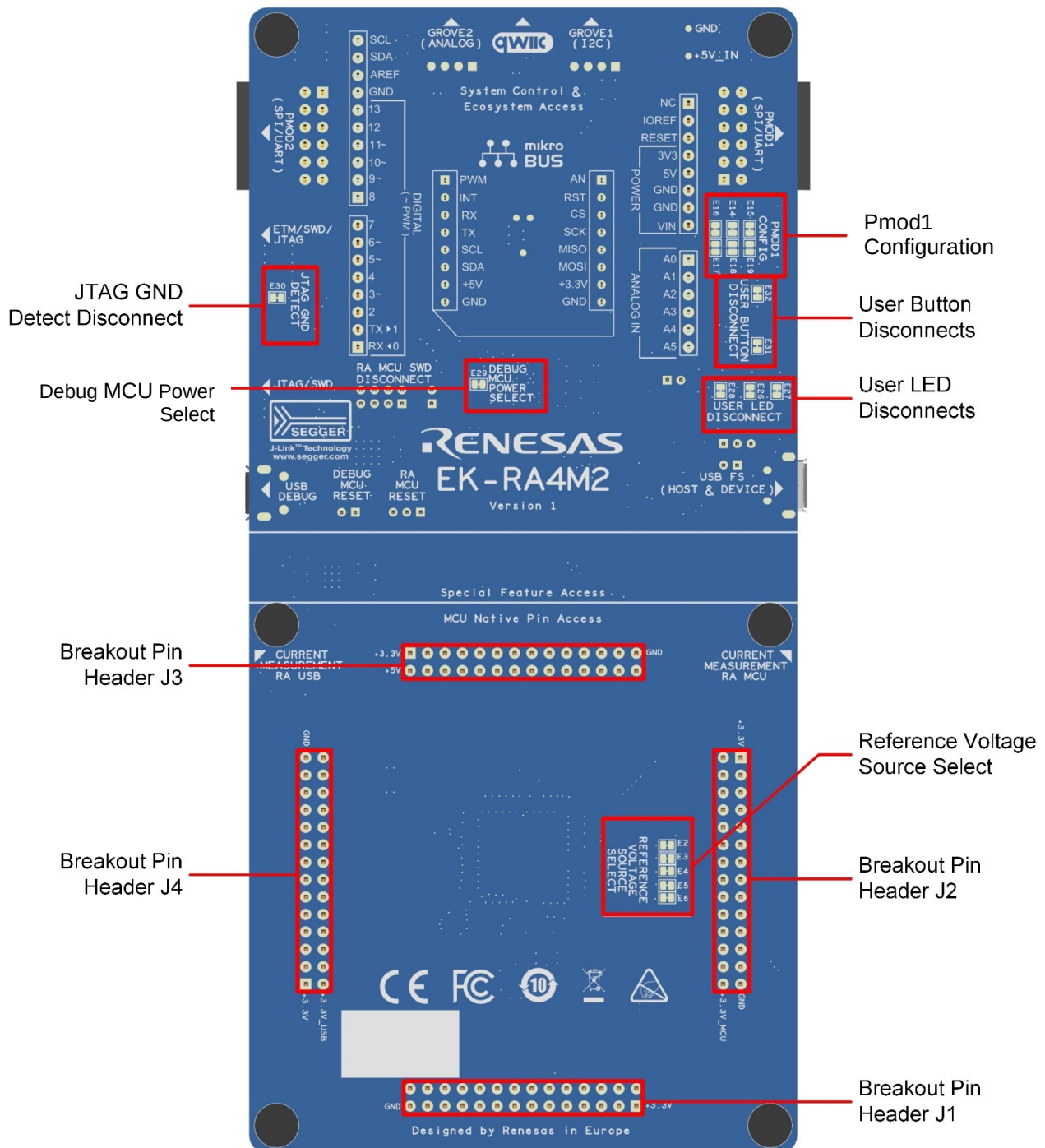
Figure 2. EK-RA4M2 Board Bottom Side
