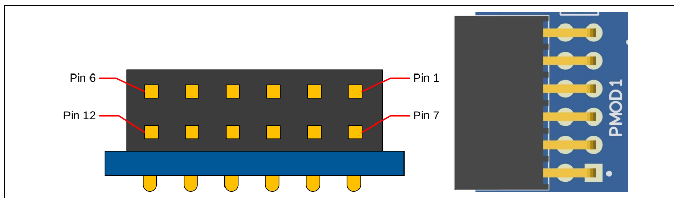
Figure 11. Pmod 1
