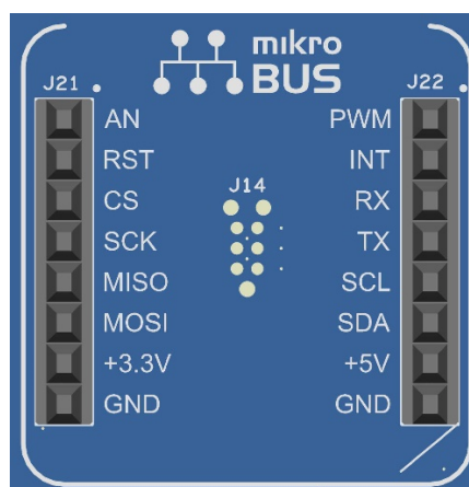
Figure 15. mikroBUS Connection
