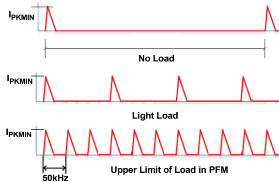
Figure 21. PFM Operation in Light Load
