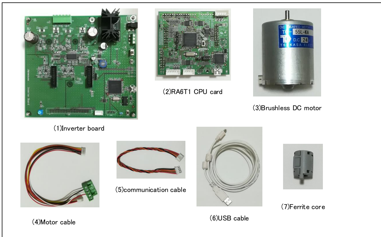
Figure 2-1 Product contents
