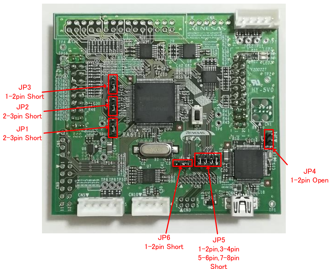
Figure 4-2 Jumper pin setting
