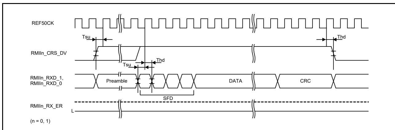
Figure 2.77 RMI Reception Timing (Normal Operation)
