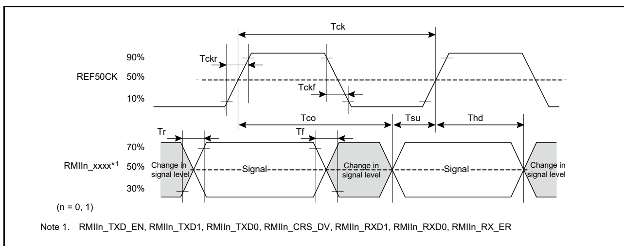
Figure 2.75 Timing with the REF50CK and RMI Signals
