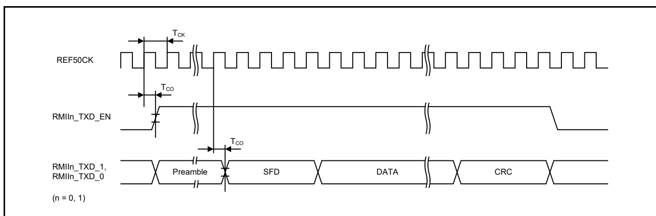
Figure 2.76 RMI Transmission Timing
