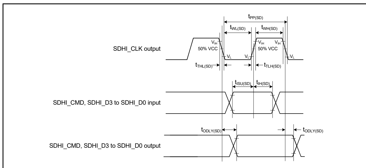
Figure 2.91 SD Host Interface Input/Output Signal Timing
