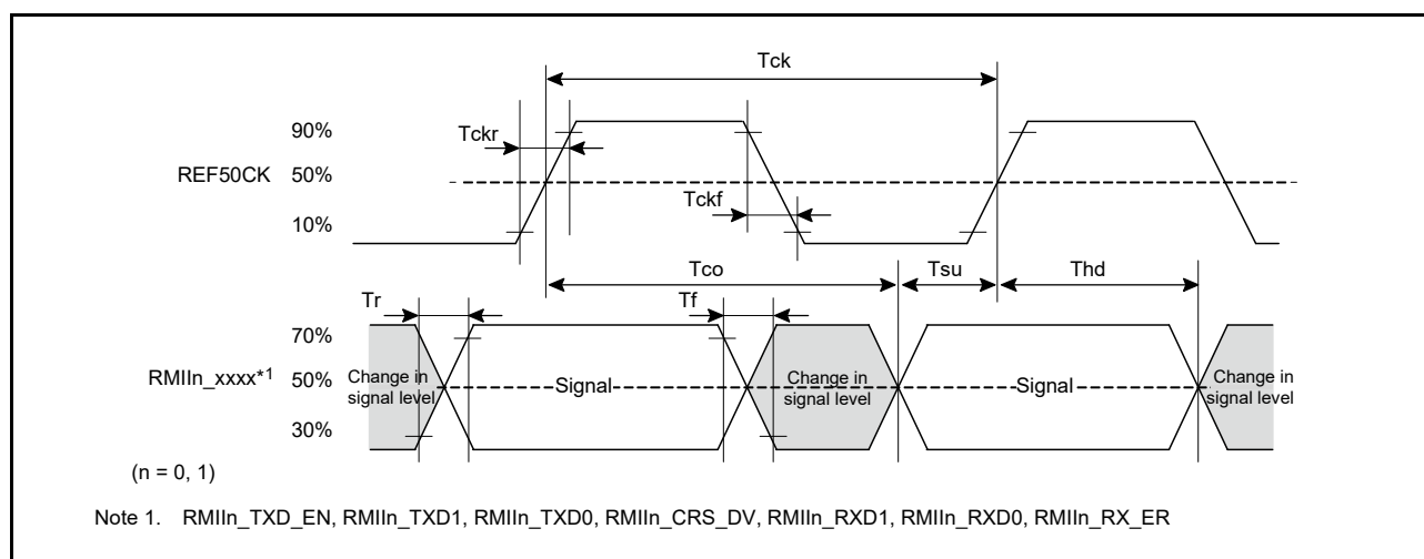
Figure 2.79 Timing with the REF50CK and RMII Signals
