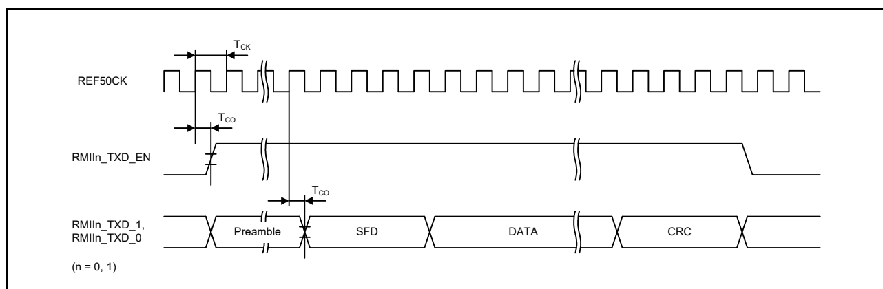
Figure 2.80 RMII Transmission Timing
