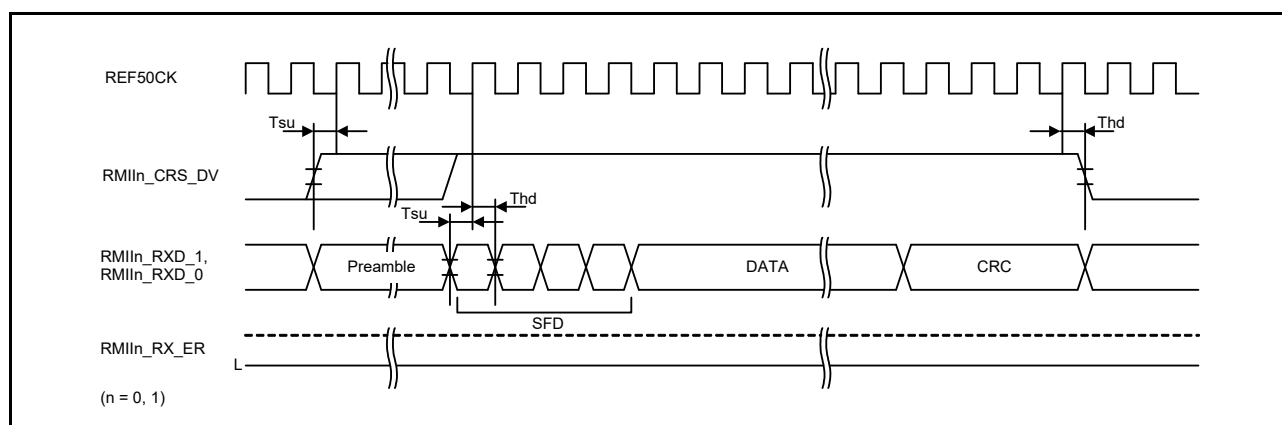
Figure 2.81 RMII Reception Timing (Normal Operation)
