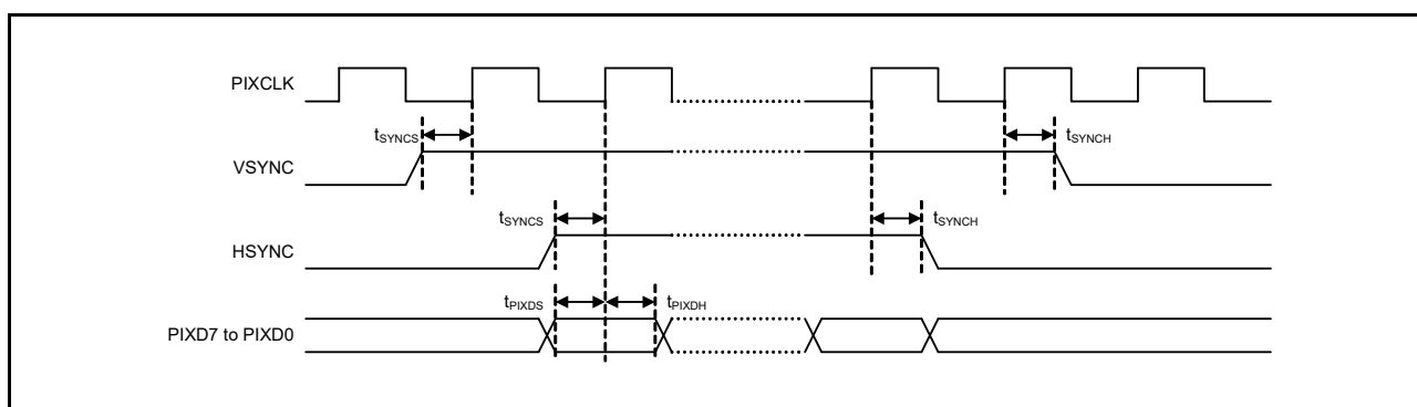
Figure 2.87 PDC AC Timing
