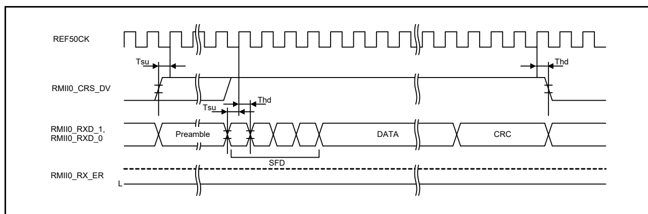
Figure 2.77 RMII Reception Timing (Normal Operation)
