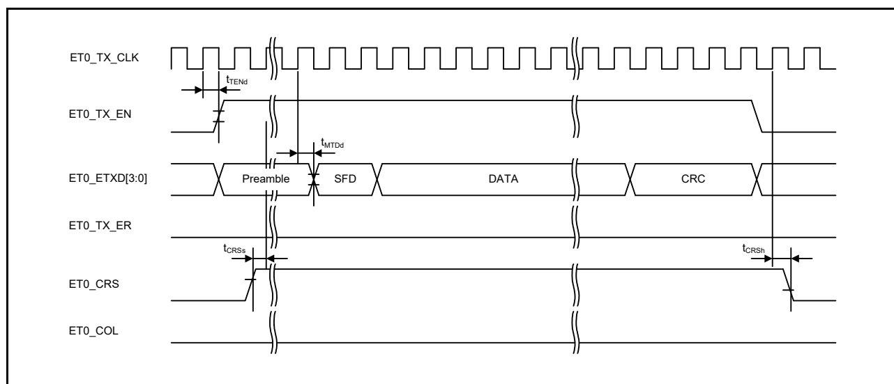
Figure 2.80 MII Transmission Timing (Normal Operation)
