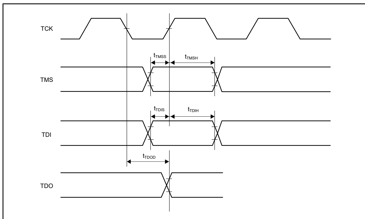
Figure 2.105 Boundary Scan Input/Output Timing
