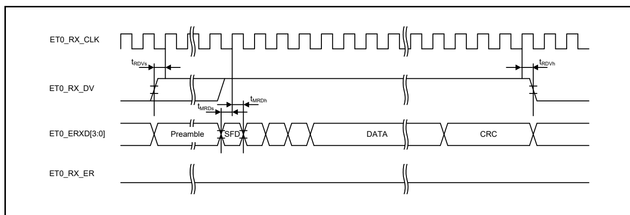
Figure 2.82 MII Reception Timing (Normal Operation)
