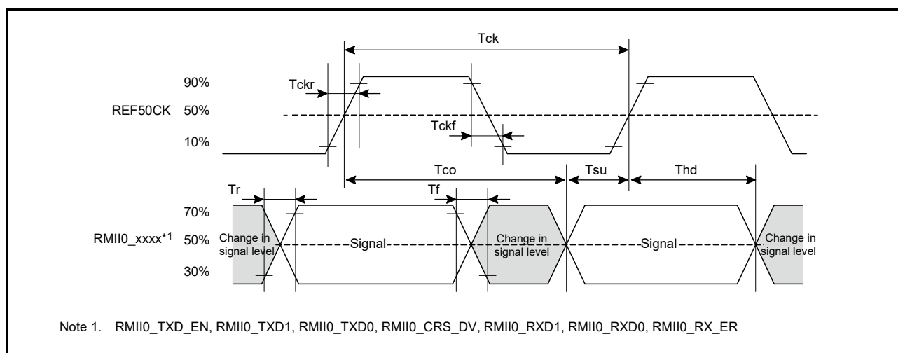
Figure 2.75 Timing with the REF50CK and RMII Signals
