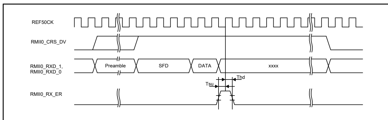
Figure 2.78 RMII Reception Timing (Error Occurrence)
