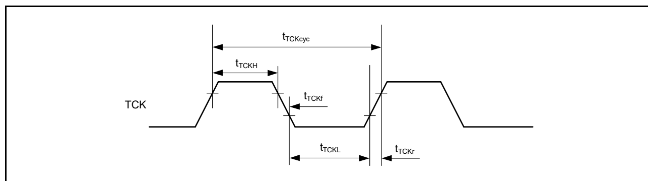
Figure 2.103 Boundary Scan TCK Timing
