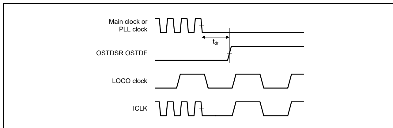
Figure 2.100 Oscillation Stop Detection Timing
