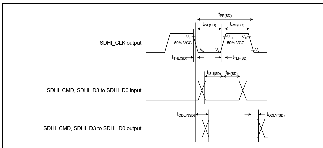
Figure 2.91 SD Host Interface Input/Output Signal Timing
