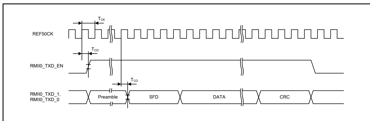
Figure 2.76 RMII Transmission Timing
