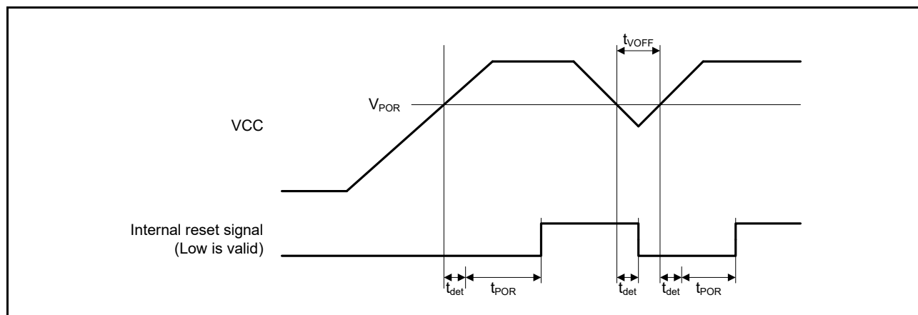
Figure 2.96 Power-on Reset Timing
