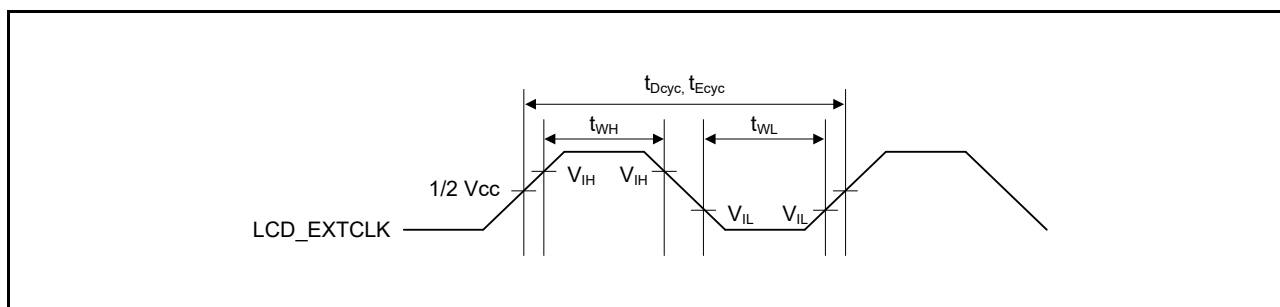
Figure 2.88 LCD_EXTCLK Clock Input Timing
