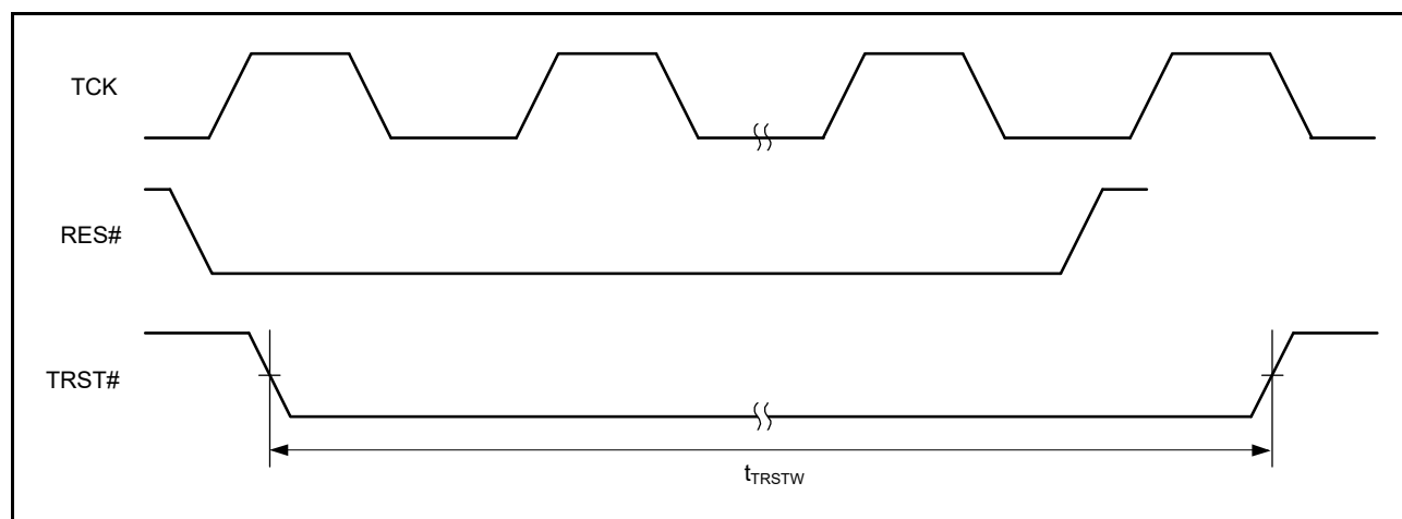
Figure 2.104 Boundary Scan TRST# Timing
