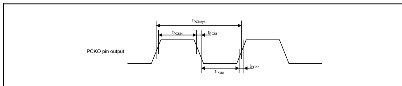
Figure 2.86 PDC Output Clock Timing
