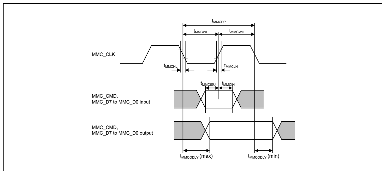
Figure 2.74 MMC Interface
