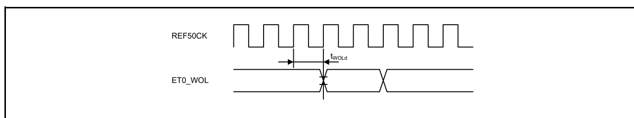
Figure 2.79 WOL Output Timing (RMII)
