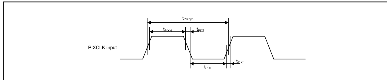
Figure 2.85 PDC Input Clock Timing
