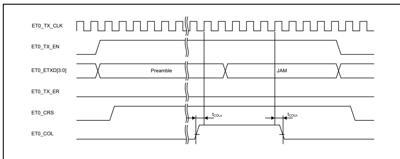
Figure 2.81 MII Transmission Timing (Conflict Occurrence)
