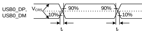
Figure 5.49 USB0_DP and USB0_DM Output Timing
