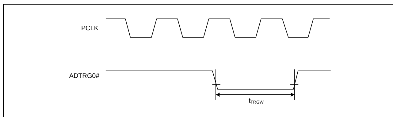
Figure 5.39 A/D Converter External Trigger Input Timing
