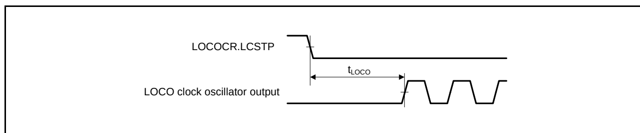
Figure 5.21 LOCO Clock Oscillation Start Timing
