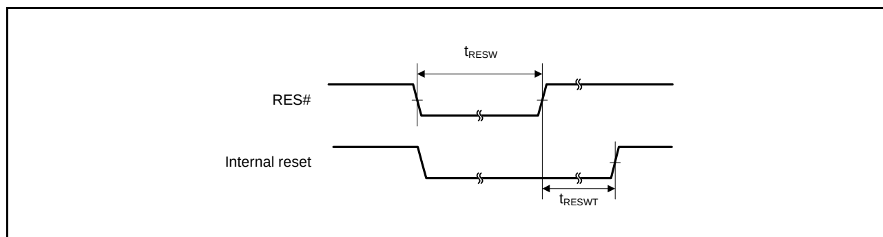
Figure 5.27 Reset Input Timing (1)
