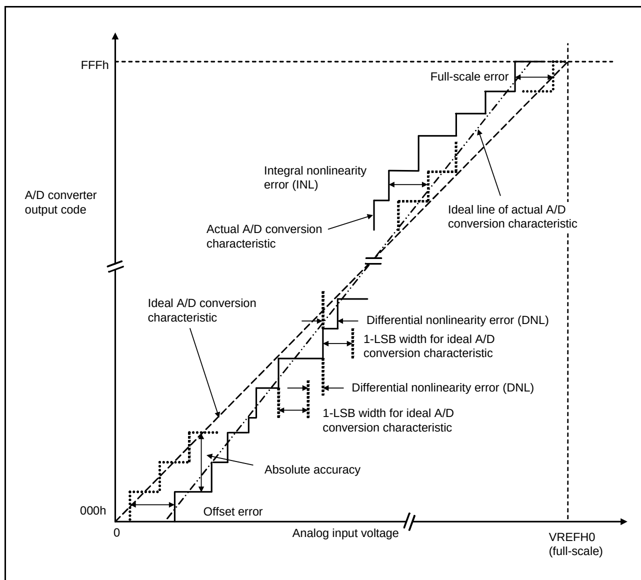
Figure 5.52 Illustration of A/D Converter Characteristic Terms
