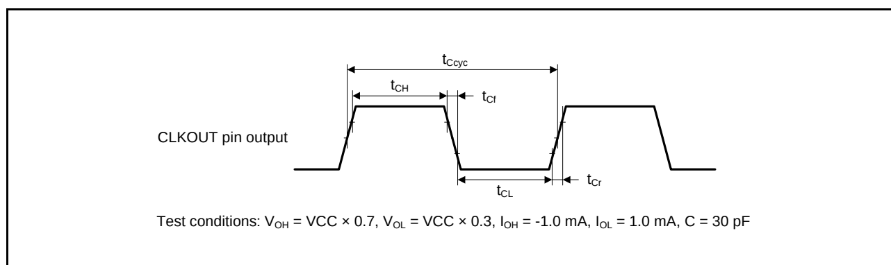
Figure 5.40 CLKOUT Output Timing
