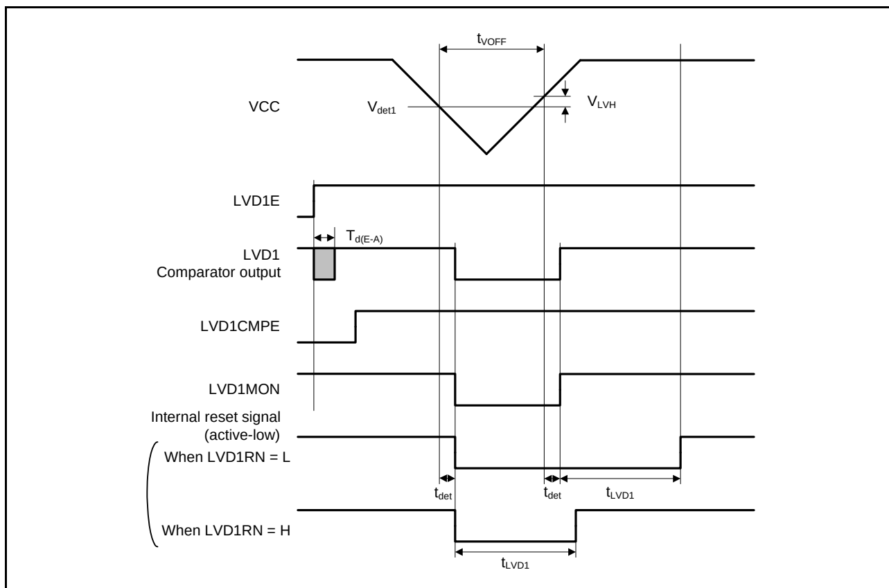
Figure 5.55 Voltage Detection Circuit Timing ( V_{det1} )
