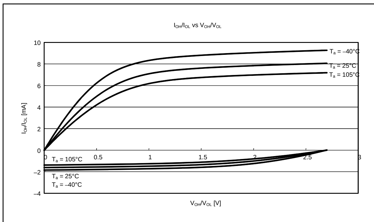
Figure 5.16 V_{OH}/V_{OL} and I_{OH}/I_{OL} Temperature Characteristics of Port 4 and Port J at V_{CC} = 2.7 V (Reference Data)
