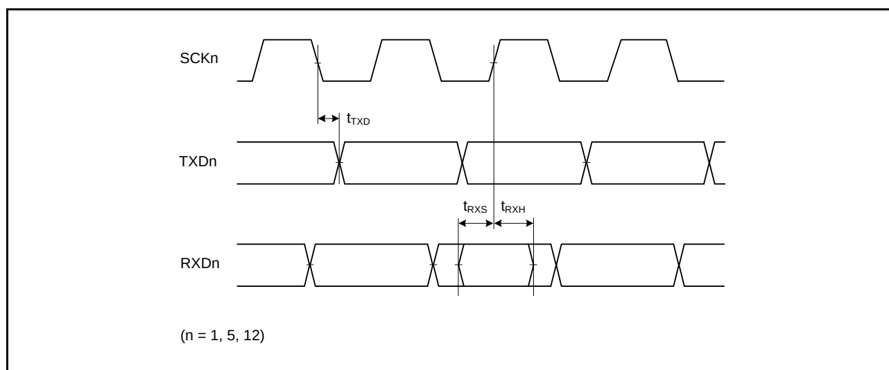
Figure 5.38 SCI Input/Output Timing: Clock Synchronous Mode
