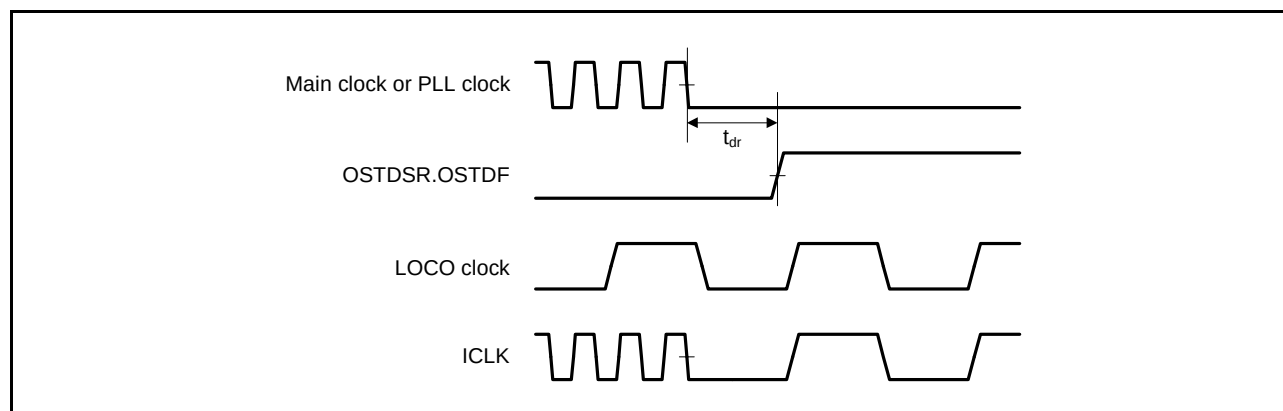
Figure 5.57 Oscillation Stop Detection Timing
