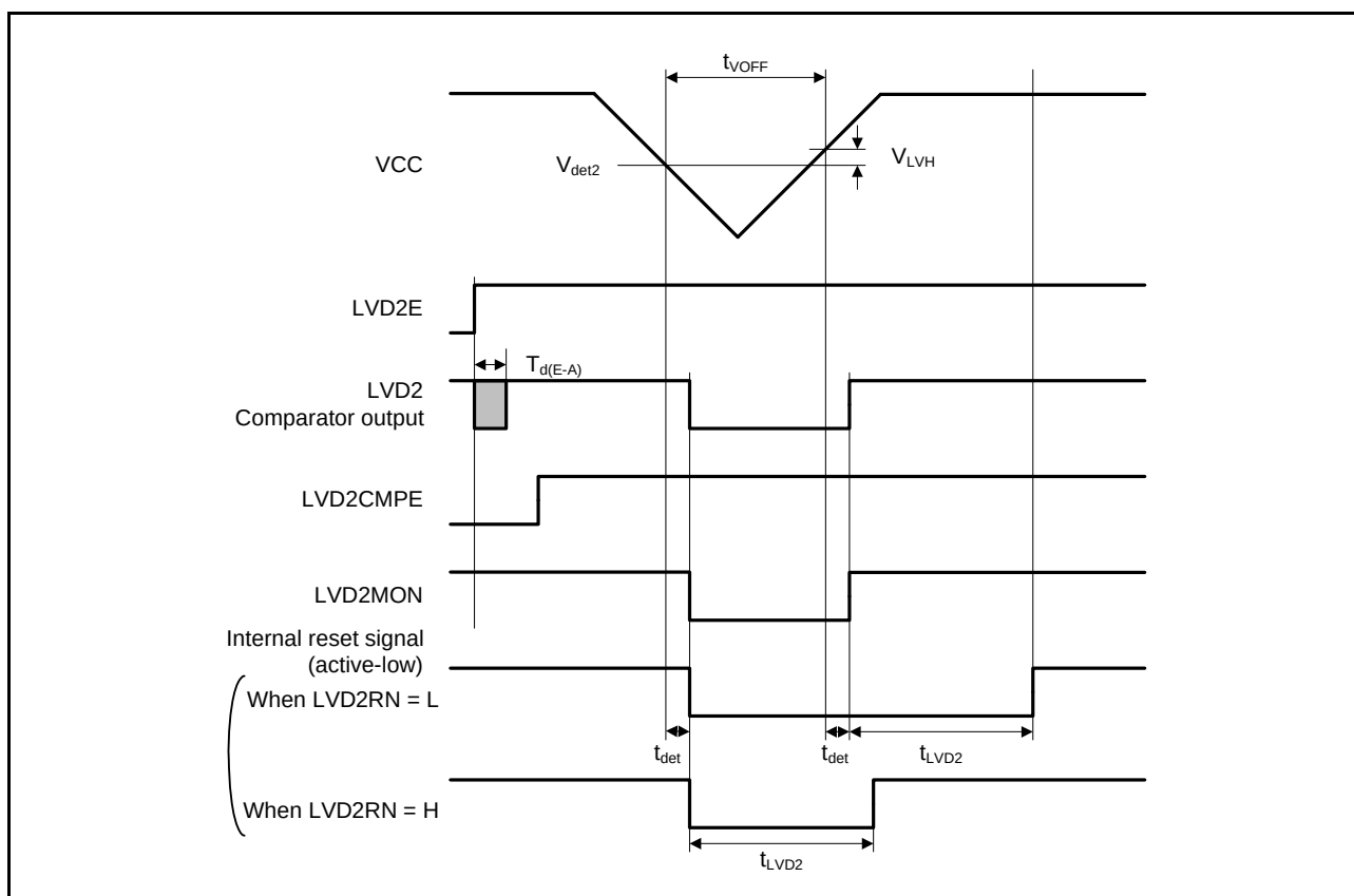
Figure 5.56 Voltage Detection Circuit Timing ( V_{det2} )
