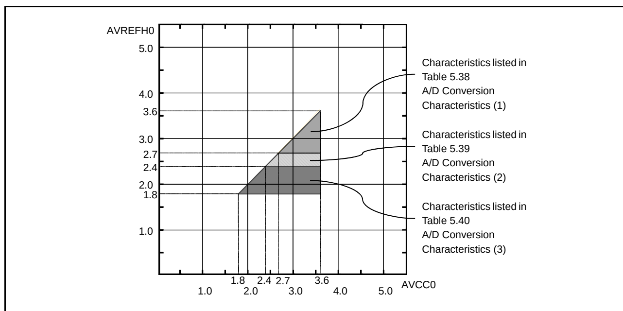
Figure 5.51 AVCC0 to AVREFH0 Voltage Range
