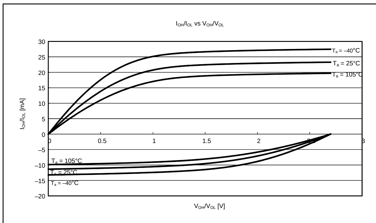
Figure 5.9 V_{OH}/V_{OL} and I_{OH}/I_{OL} Temperature Characteristics of General Ports (Except for RIIC Output Pin, Port 4, and Port J) at V_{CC} = 2.7 V (Reference Data)
