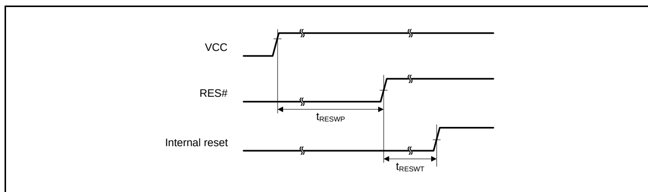
Figure 5.26 Reset Input Timing at Power-On
