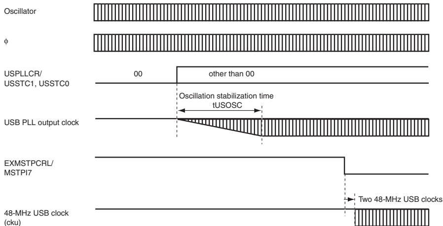
Figure 26.38 Timing of Oscillation Stabilization Time of USB PLL
