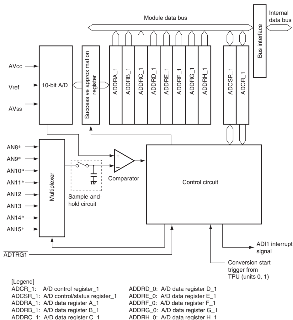
Figure 18.2 Block Diagram of A/D Converter Unit 1 (AD_1)
