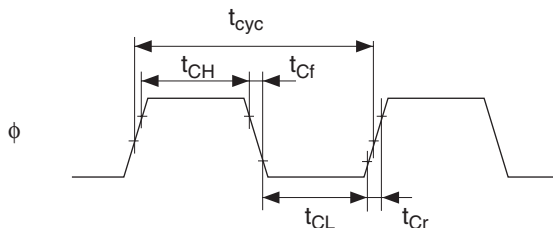
Figure 26.3 System Clock Timing
