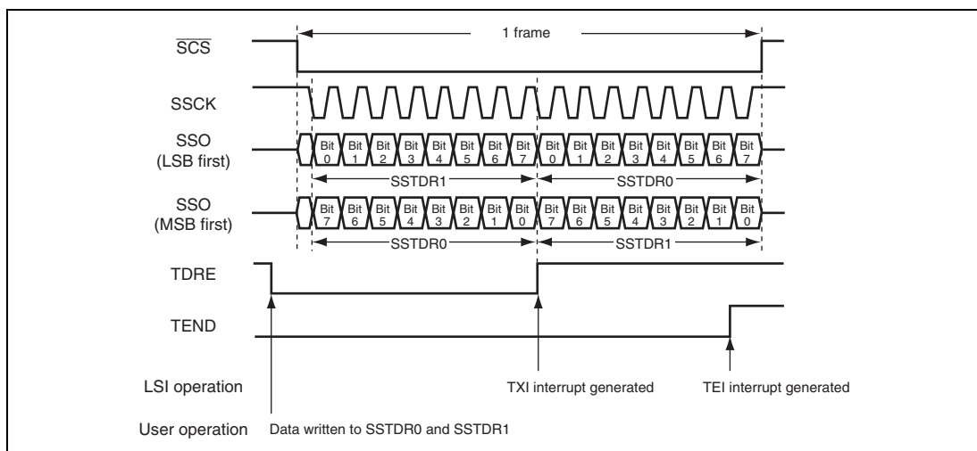
Figure 20.5 (2) Example of Transmission Operation (SSU Mode) When 16-bit data length is selected (SSTD0 and SSTDR1 are valid) with CPOS = 0 and CPHS = 0
