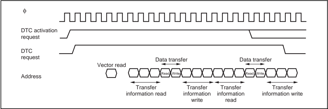
Figure 9.12 DTC Operation Timing (Example of Chain Transfer)
