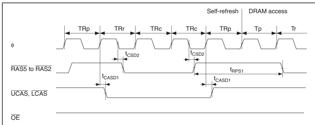
Figure 26.23 Self-Refresh Timing (Return from Software Standby Mode: RAST = 1)
