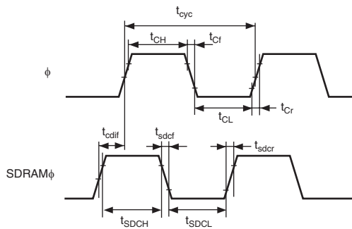
Figure 26.4 SDRAM \phi Timing
