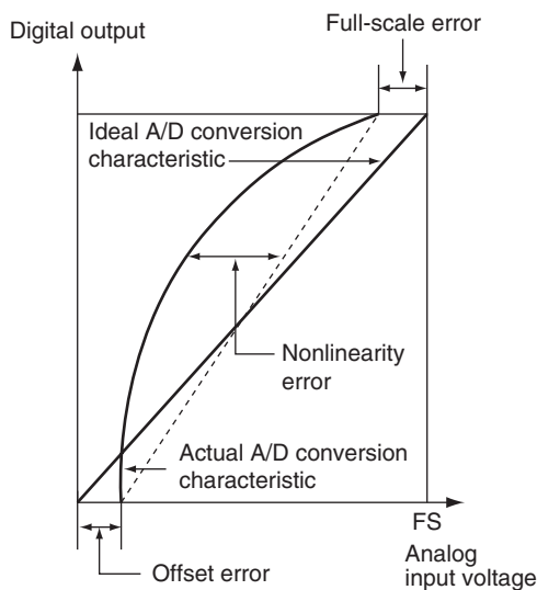
Figure 18.10 A/D Conversion Accuracy Definitions
