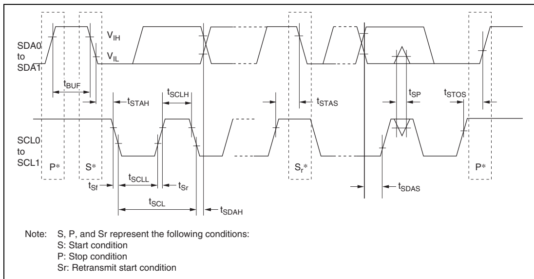
Figure 26.50 I²C Bus Interface 2 Input/Output Timing
