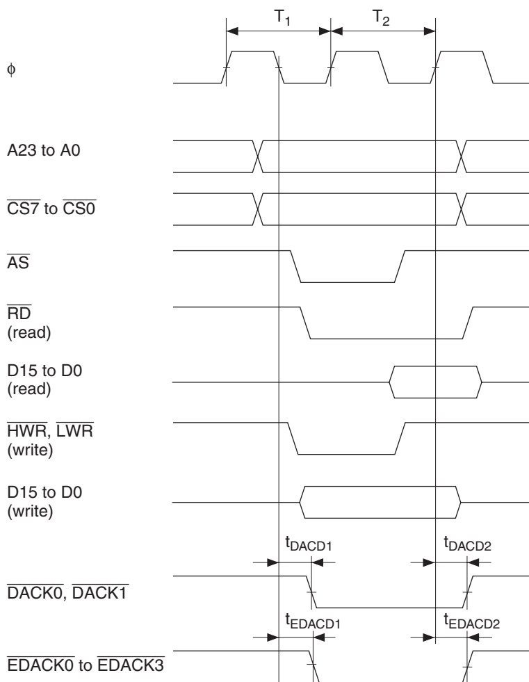
Figure 26.31 DMAC and EXDMAC Single Address Transfer Timing: Two-State Access
