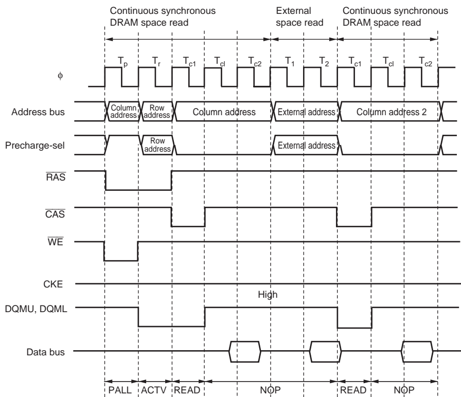
Figure 6.65 Example of Operation Timing in RAS Down Mode (BE = 1, CAS Latency 2)
