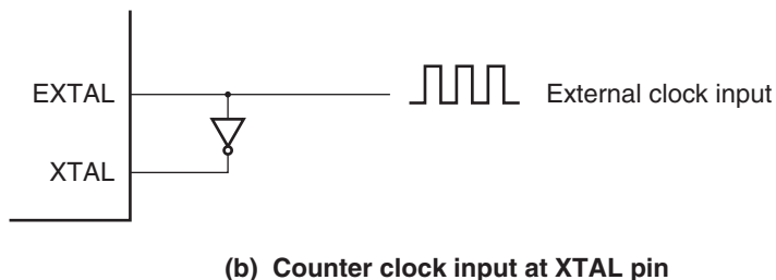
Figure 23.4 Connection of External Clock Input (Examples)
