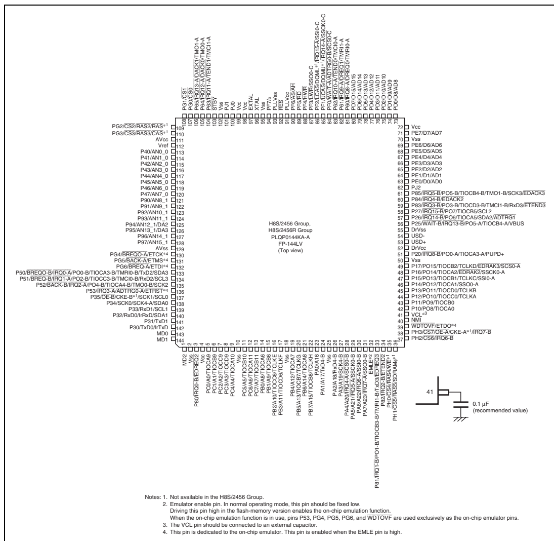
Figure 1.4 Pin Assignments for H8S/2456 Group and H8S/2456R Group (1)
