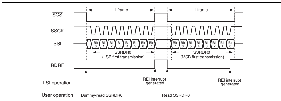
Figure 20.7 (1) Example of Reception Operation (SSU Mode)
