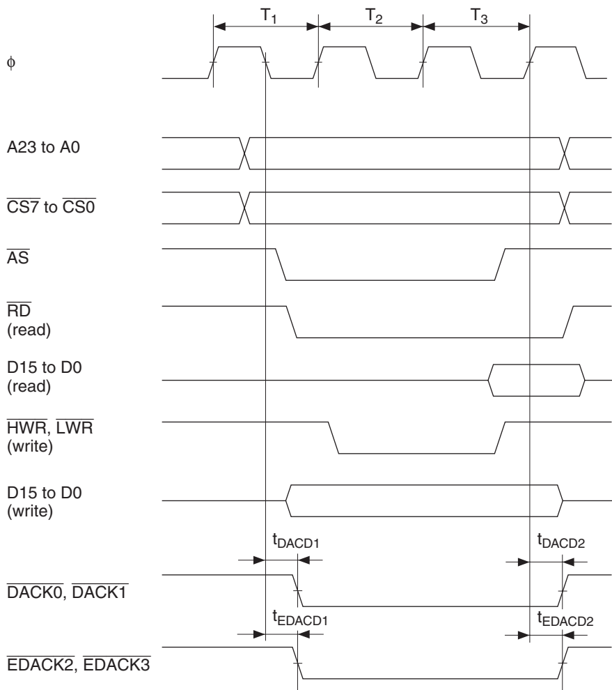
Figure 26.32 DMAC and EXDMAC Single Address Transfer Timing: Three-State Access
