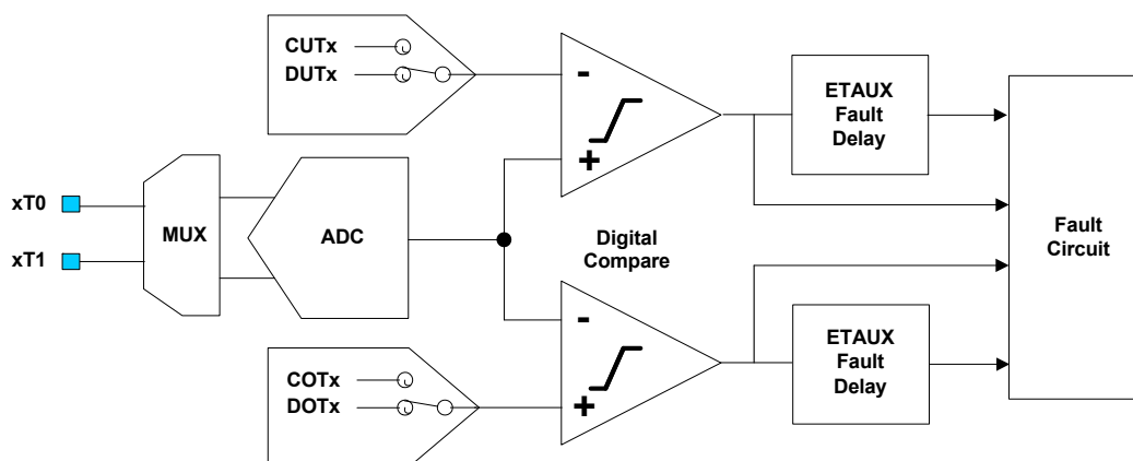
Figure 89. ETAUX Fault Detector Block Diagram
