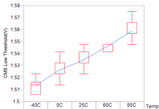
Figure 75. CMS Pins VIL
