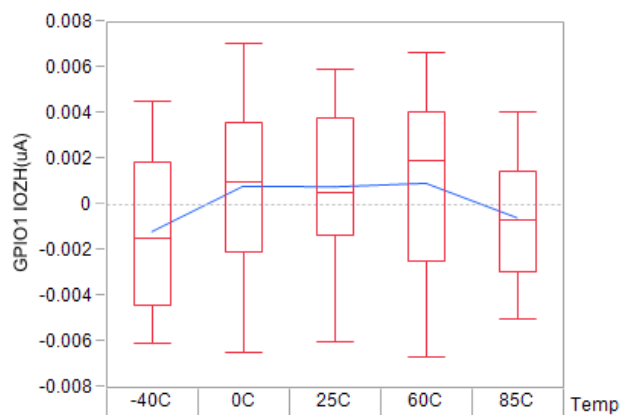
Figure 70. GPIO1 Leakage Current (3.3V)
