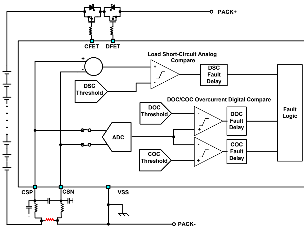
Figure 82. Current Sense Block Diagram
