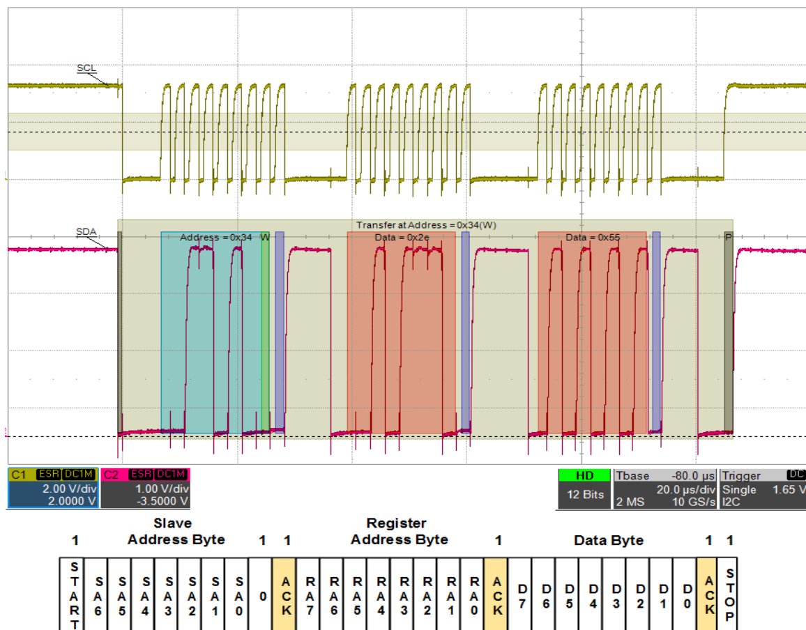
I2C 1-BYTE WRITE
