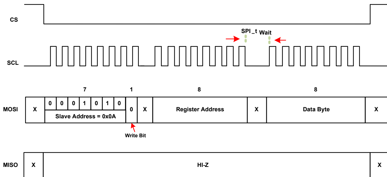
Figure 117. SPI Write
