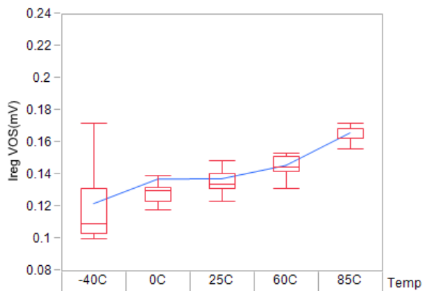
Figure 28. I_{REG} Measurement Offset
