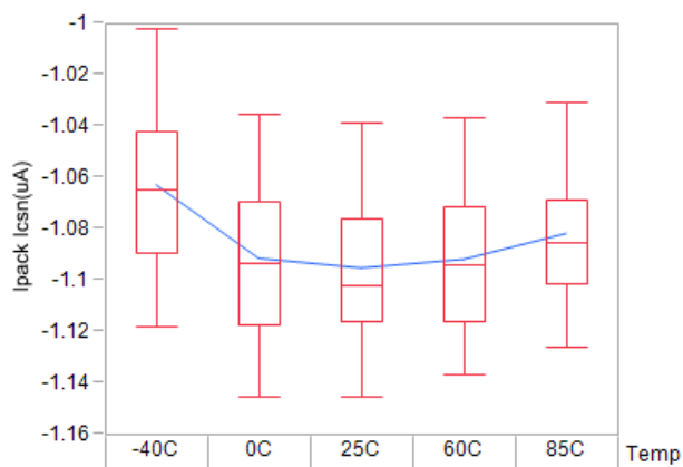
Figure 13. I_{CSN} Pin Measurement Input Current
