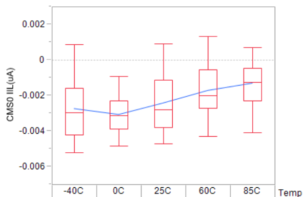
Figure 76. CMS0 Leakage Current (3.3V)
