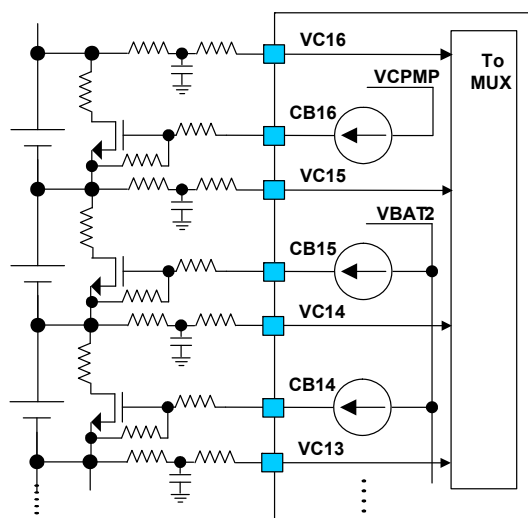
Figure 95. External Cell Balancing Configuration
