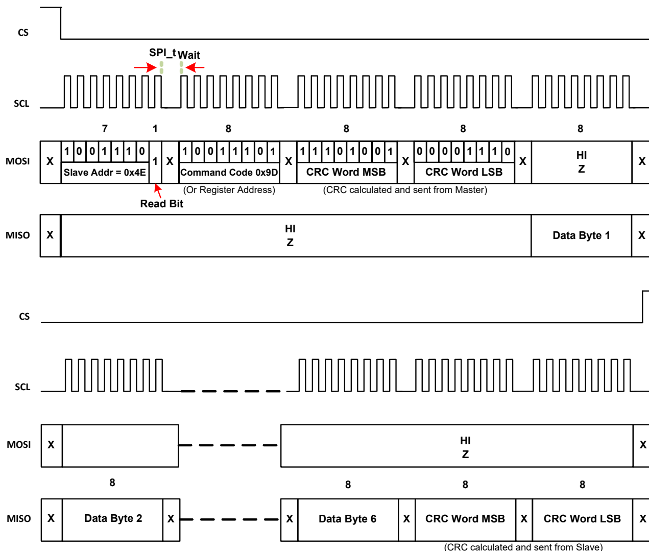
Figure 120. SPI I 2 C Read w/CRC
