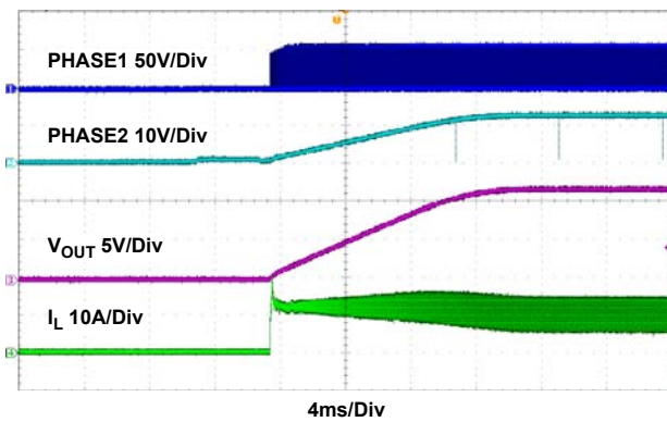
Figure 38. Start-Up Waveform, V_{IN} = 60V I_O = 10A , CCM
