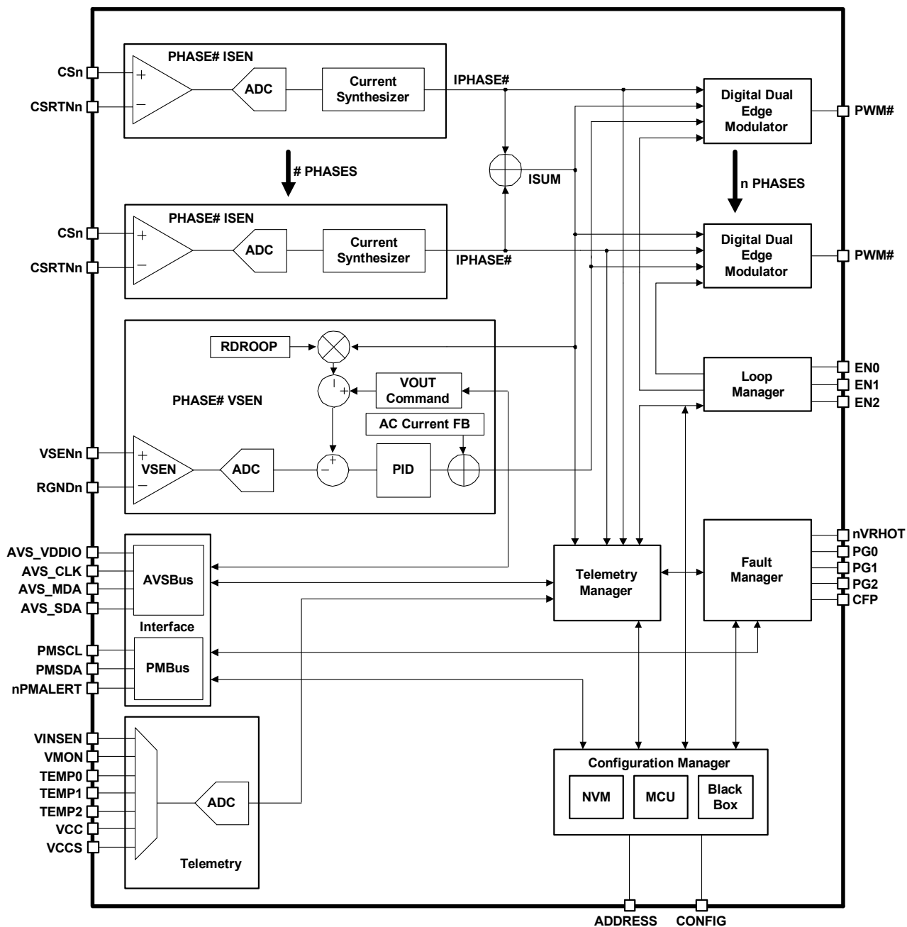
Figure 4. ISL68239 Internal Block Diagram
