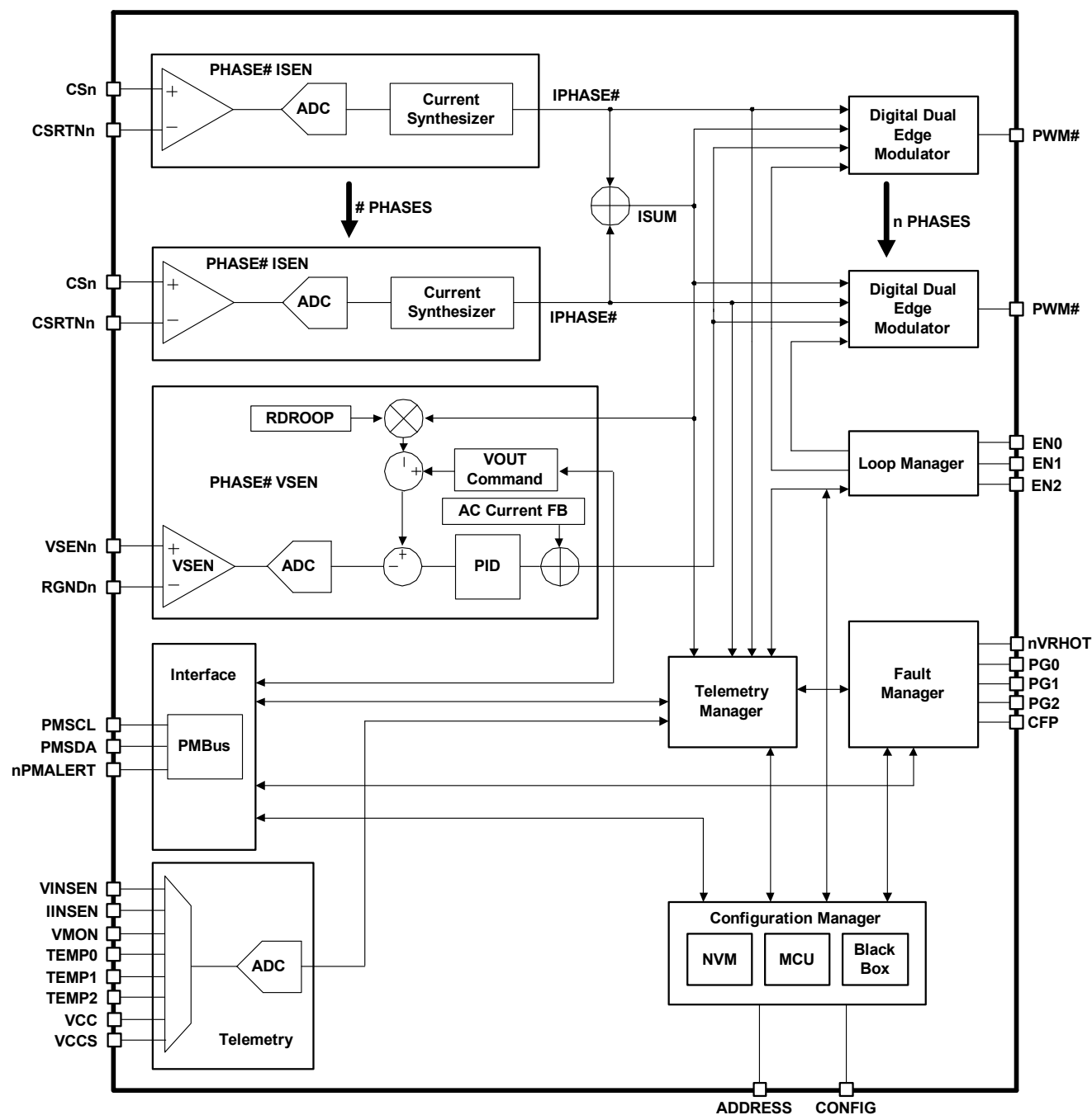
Figure 3. ISL68229 Internal Block Diagram
