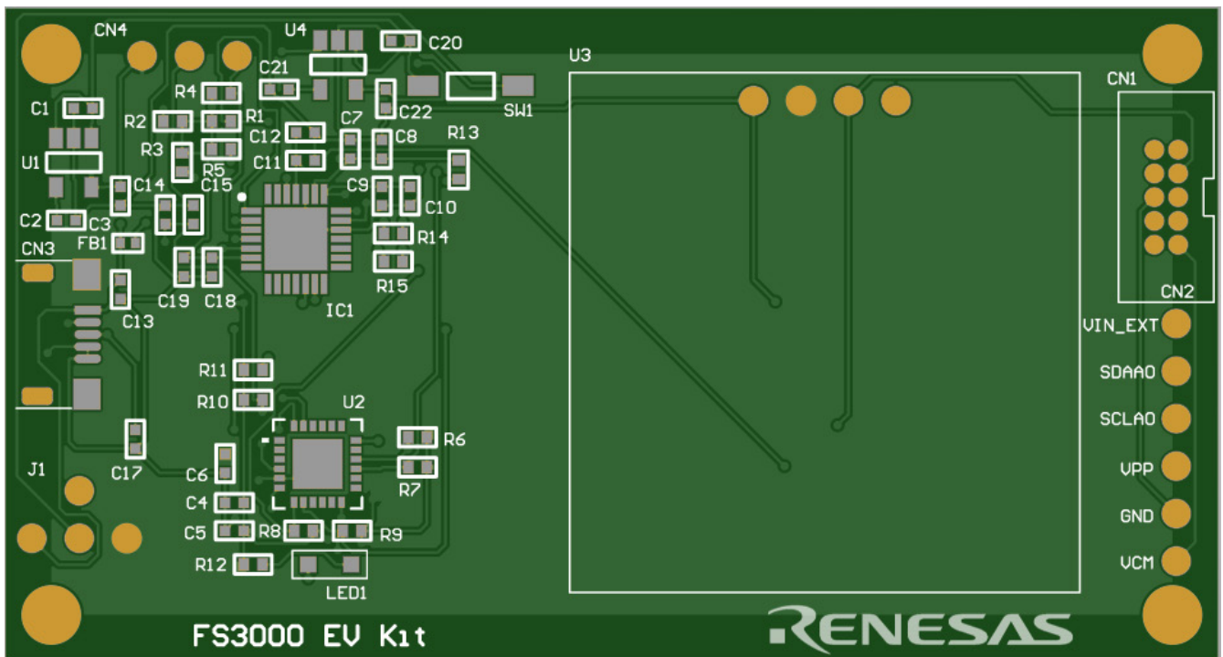
Figure 5. Top Layer
