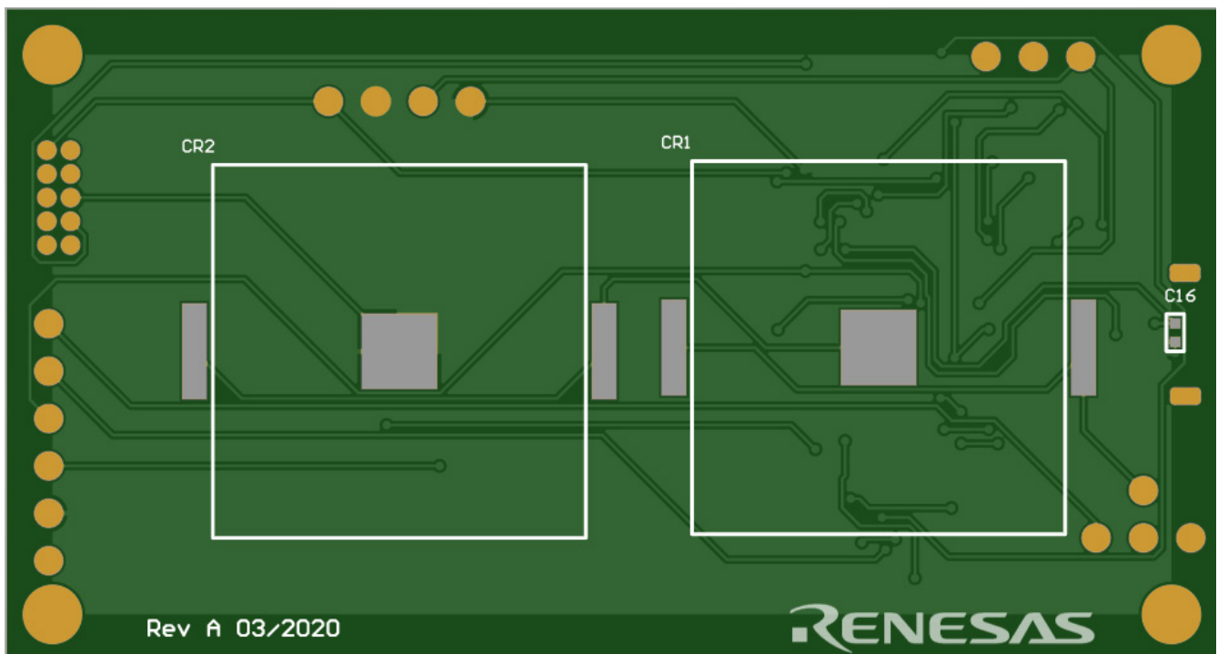
Figure 6. Bottom Layer
