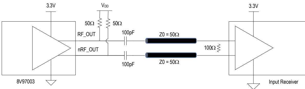
Figure 14. Resistive Matching Termination
