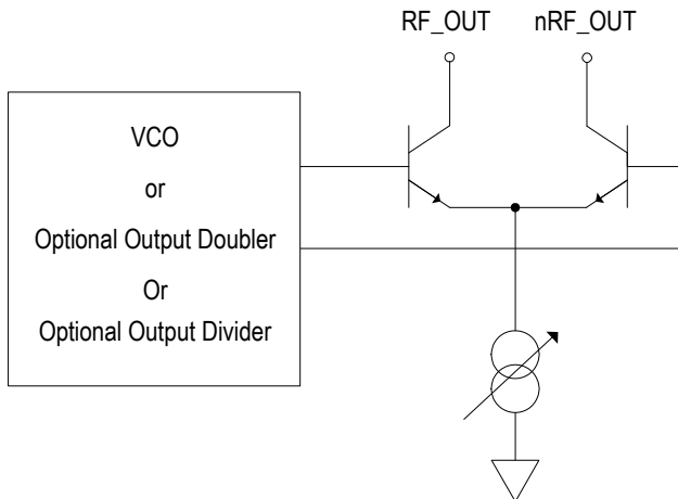
Figure 13. Output Stage
