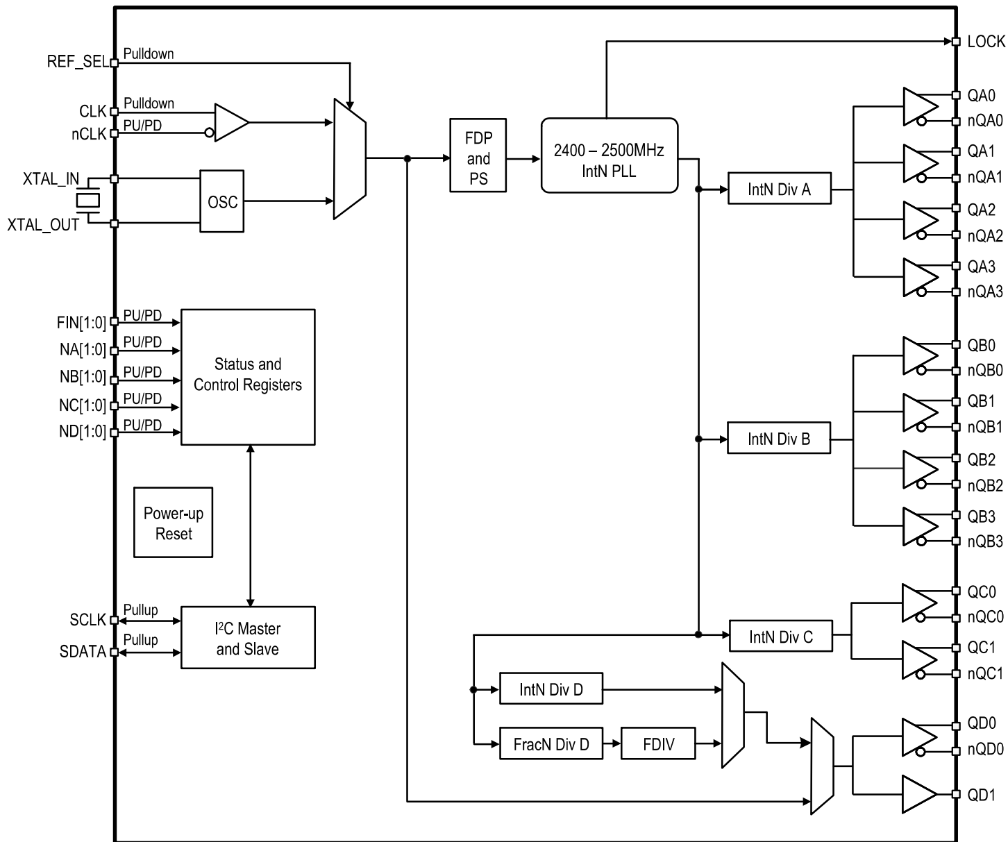
Figure 1. 8V49NS1412 Block Diagram
