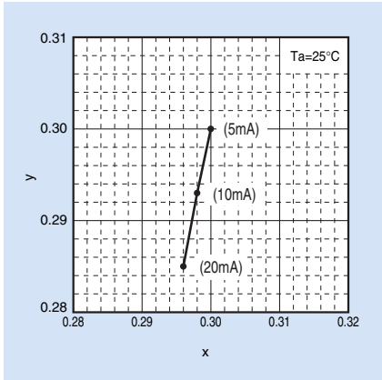
Forward Current - Chromaticity Diagram
