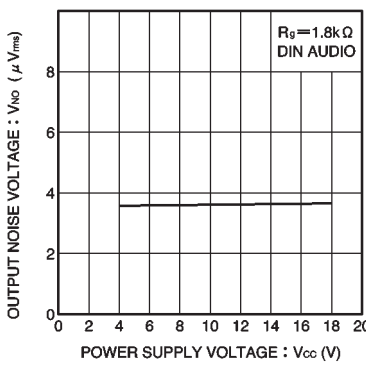
Fig. 9 Output noise voltage vs. power supply voltage
