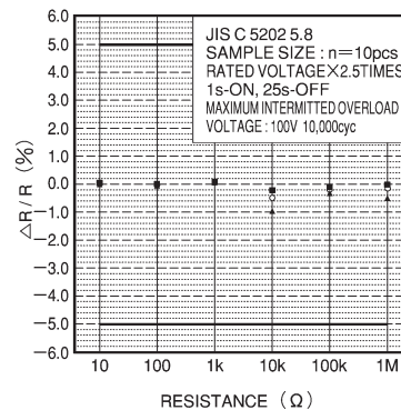
Fig.8 Intermittent overload
