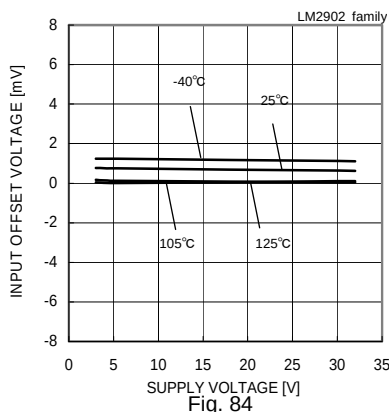
Fig. 84 Input Offset Voltage – Supply Voltage ( V_{icm}=0[V] , V_{OUT}=1.4[V] )
