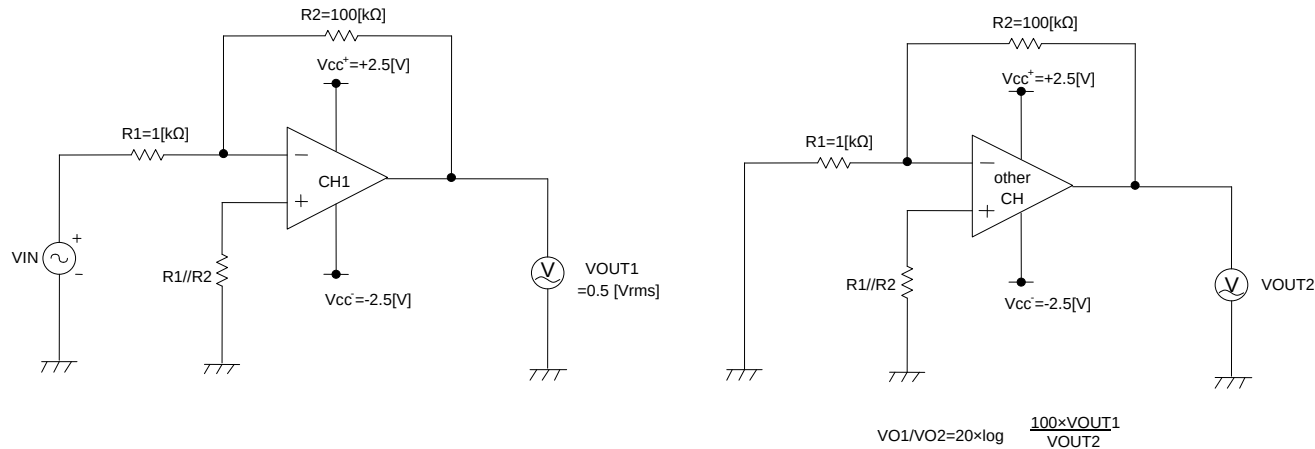
Fig.101 Measurement Circuit3
