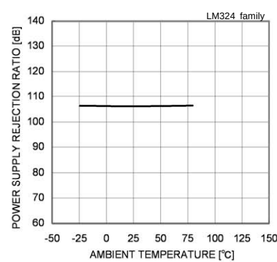
Fig. 48 Power Supply Rejection Ratio – Ambient Temperature
