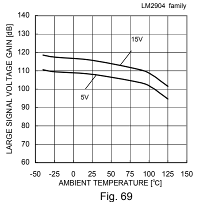
Fig. 69 Large Signal Voltage Gain – Ambient Temperature (RL=2[kΩ])
