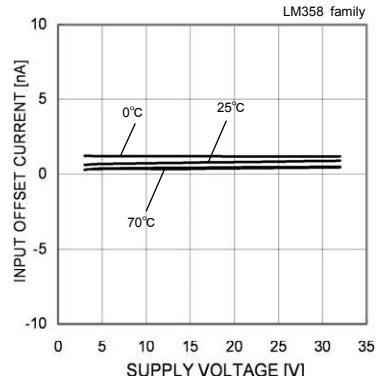
Fig. 18 Input Offset Current – Supply Voltage (Vicm=0[V], VOUT=1.4[V])
