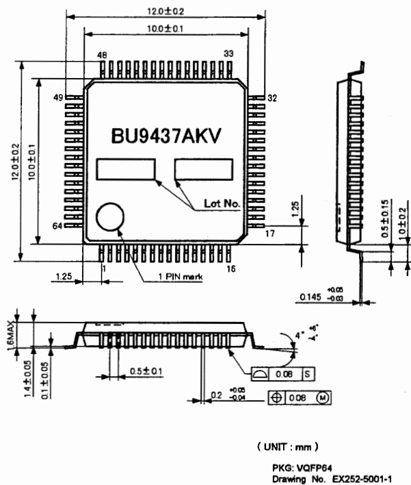
Figure 1. External dimension
