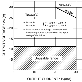
Fig.2 Derating curve
