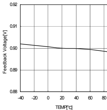
Fig.7 Feedback voltage
