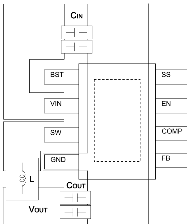
Fig.26 The example of PCB layout pattern
