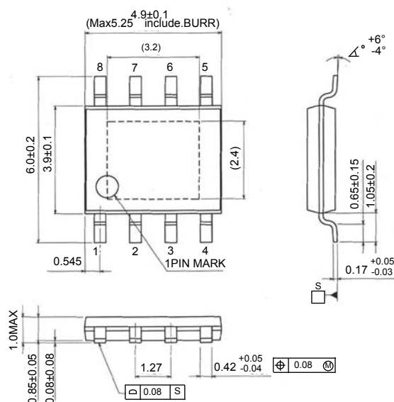
Fig.3 HTSOP-J8 Package (Unit:mm)
