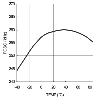
Fig.9 Operating Frequency
