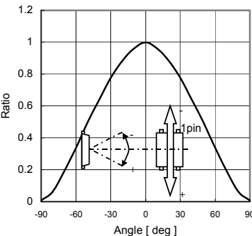
Fig.5 Directional Characteristics 2
