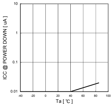
Fig.10 VCC - ICC@0 Lx (POWER DOWN)
