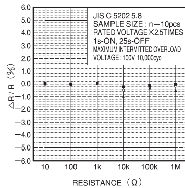
Fig.8 Intermittent overload
