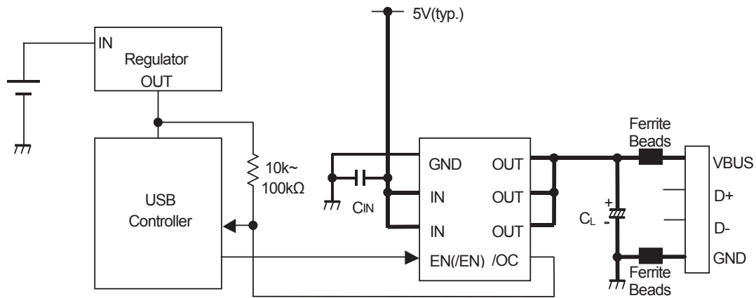
Fig.43 Typical application circuit
