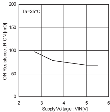
Fig.9 On-resistance
