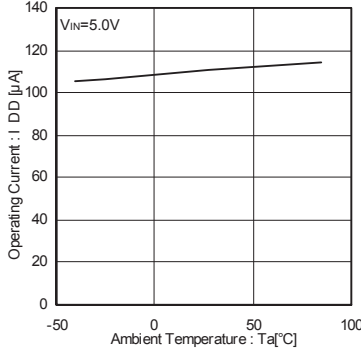
Fig.4 Operating current EN,/EN enable
