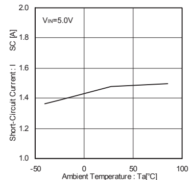
Fig.14 Short circuit current
