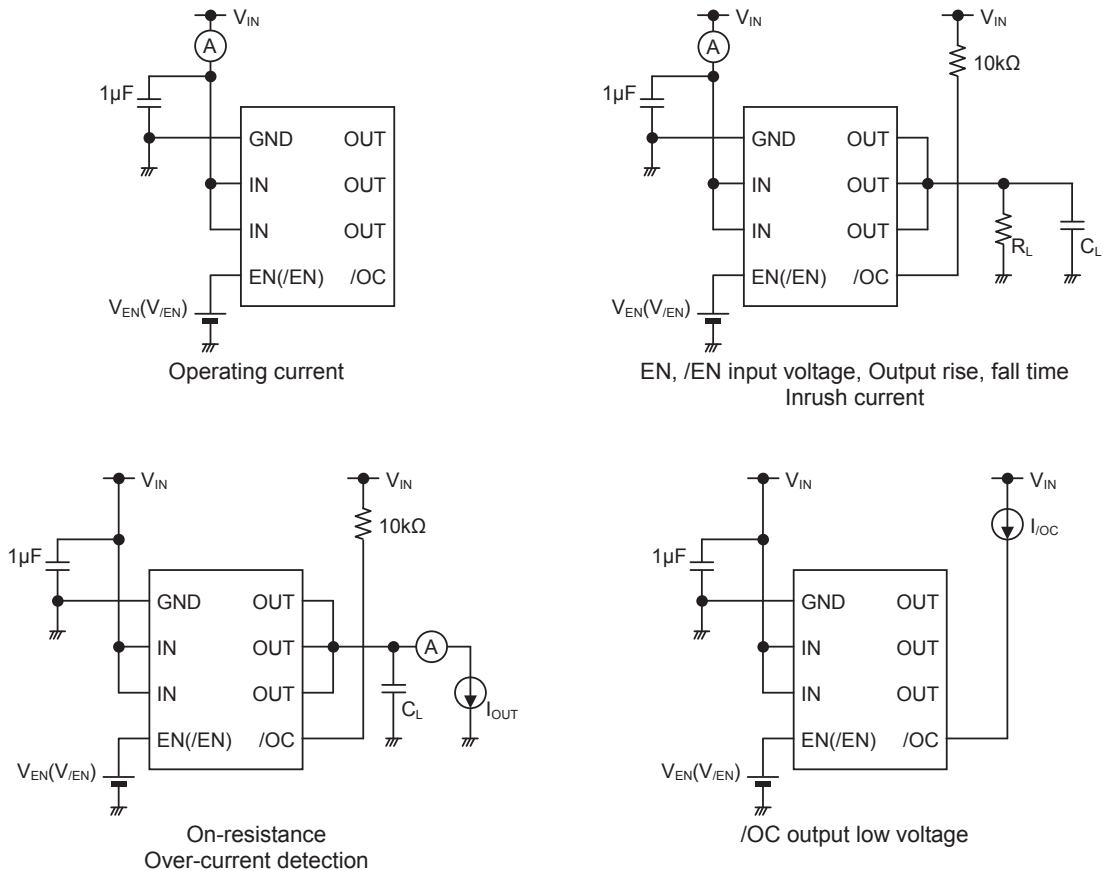
Fig.1 Measurement circuit
