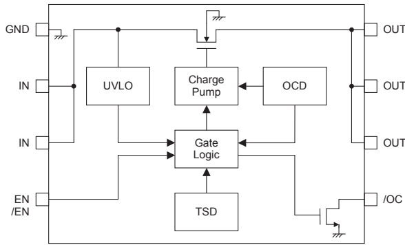
Fig.39 Block diagram
