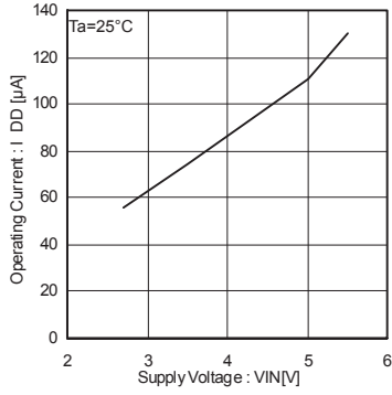
Fig.3 Operating current EN,/EN enable
