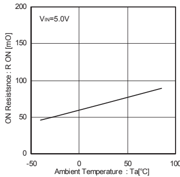
Fig.10 On-resistance
