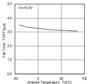
Fig.24 Output fall time
