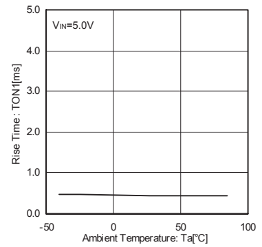
Fig.20 Output rise time
