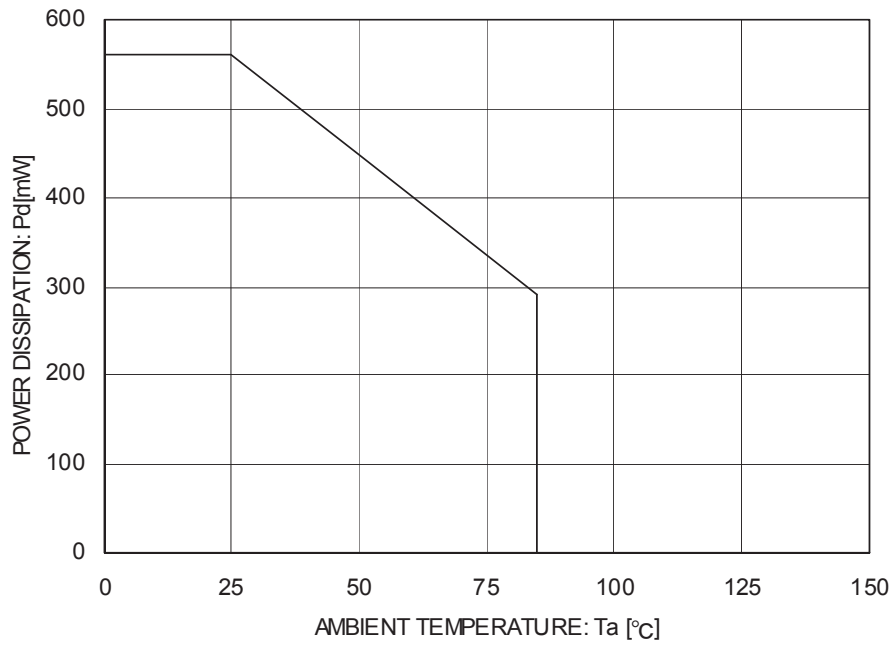
Fig.44 Power dissipation curve (Pd-Ta Curve)
