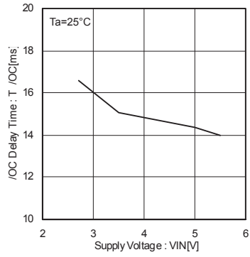
Fig.27 /OC delay time
