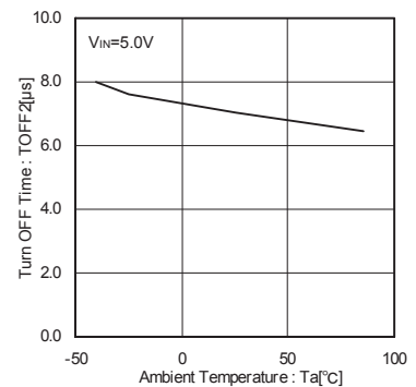
Fig.26 Output turn-off time
