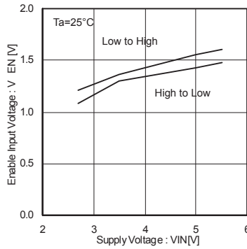
Fig.7 EN,/EN input voltage
