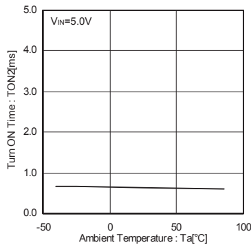
Fig.22 Output turn-on time
