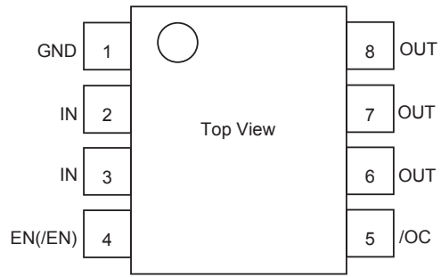
Fig.40 Pin configuration
