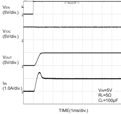
Fig.29 Output rise characteristic
