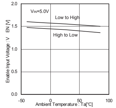
Fig.8 EN,/EN input voltage
