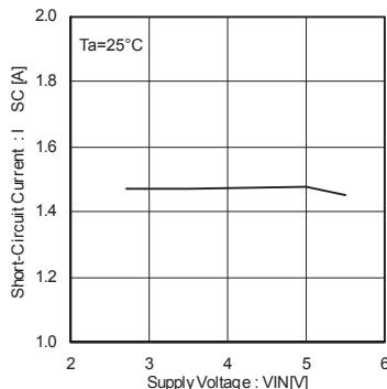
Fig.13 Short circuit current
