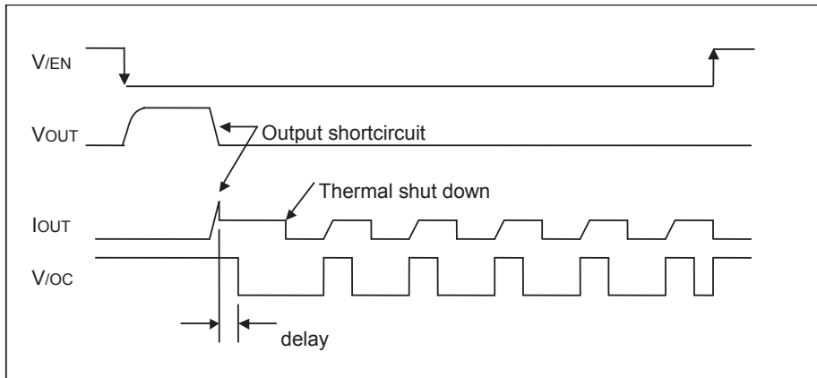
Fig.41 Over-current detection, thermal shutdown timing (BD82061FVJ)
