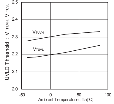
Fig.17 UVLO threshold voltage
