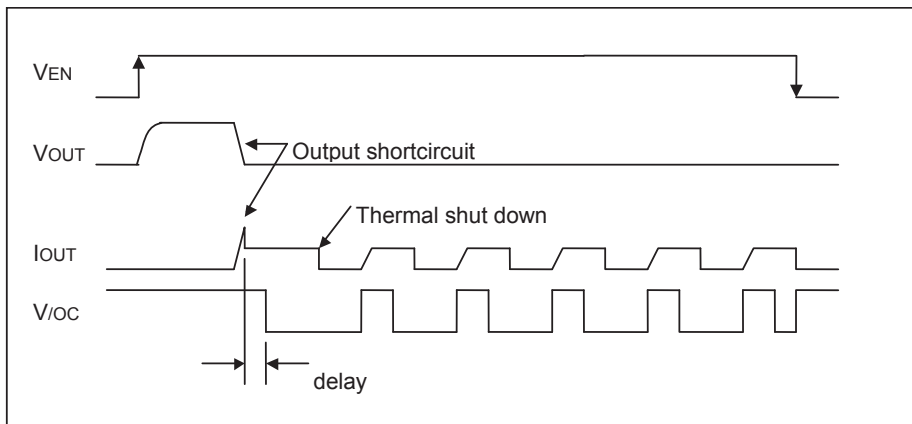
Fig.42 Over-current detection, thermal shutdown timing (BD82065FVJ)
