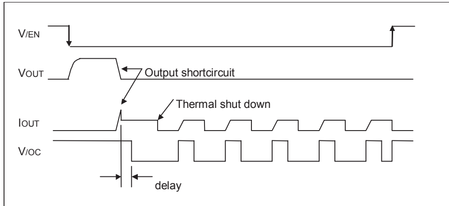
Fig.41 Over-current detection, thermal shutdown timing (BD82000FVJ)
