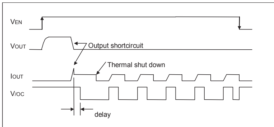
Fig.42 Over-current detection, thermal shutdown timing (BD82001FVJ)
