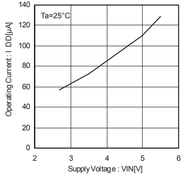
Fig.3 Operating current EN, /EN enable
