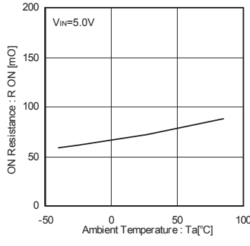
Fig.10 On-resistance
