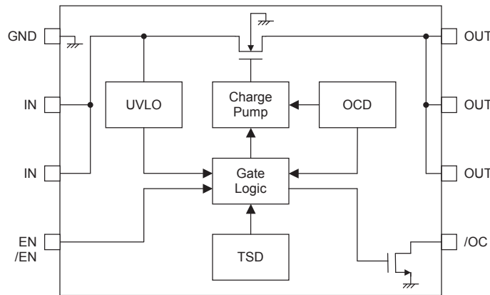
Fig.39 Block diagram
