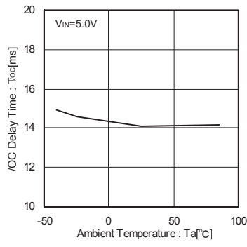
Fig.28 /OC delay time
