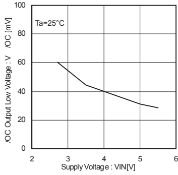
Fig.15 /OC output low voltage
