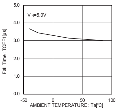
Fig.24 Output fall time
