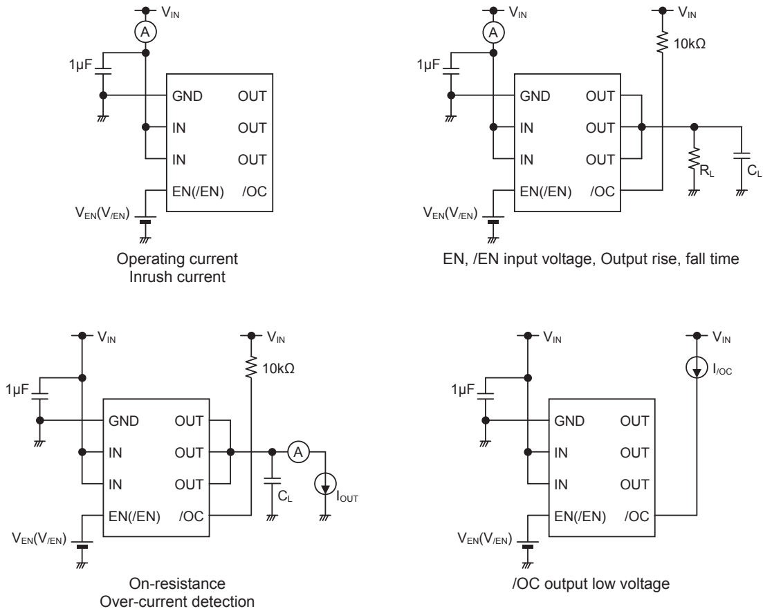
Fig.1 Measurement circuit
