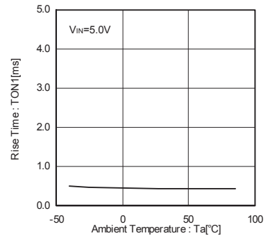
Fig.20 Output rise time
