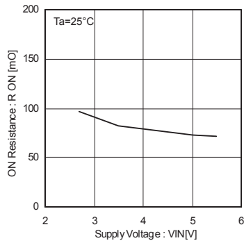
Fig.9 On-resistance
