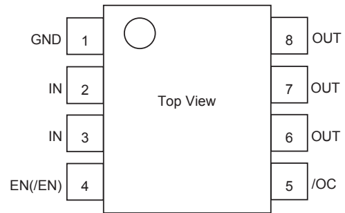
Fig.40 Pin configuration
