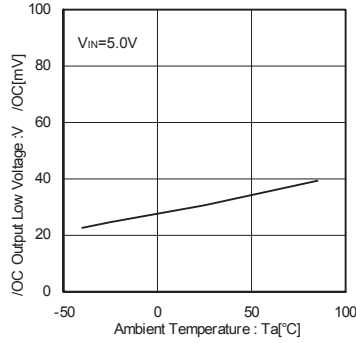
Fig.16 /OC output low voltage
