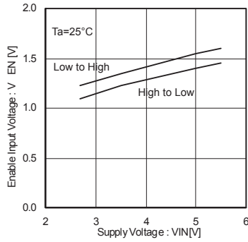
Fig.7 EN, /EN input voltage
