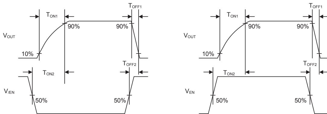
Fig.2 Timing diagram
