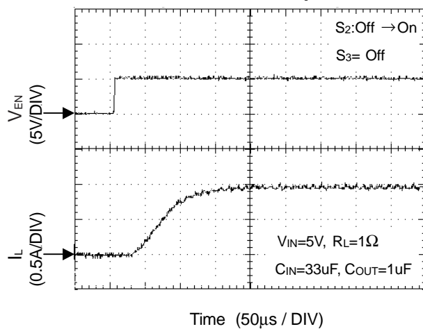
Soft- Start Response ⑤
