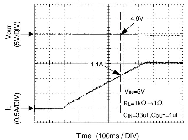
Ramped Load Response ⑤
