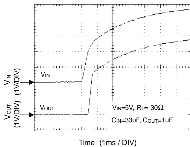
UVLO at Rising ④
