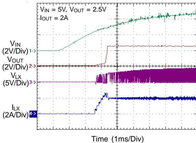
Power On &amp; Inductor Current
