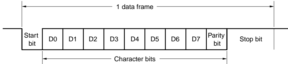
Figure 13-7. Format of Normal UART Transmit/Receive Data
