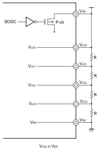
(g) 1/4 bias method (MDSET1, MDSET0 = 0, 0) (example of V_{DD} = 5\text{ V} , V_{LC0} = 5\text{ V} )
