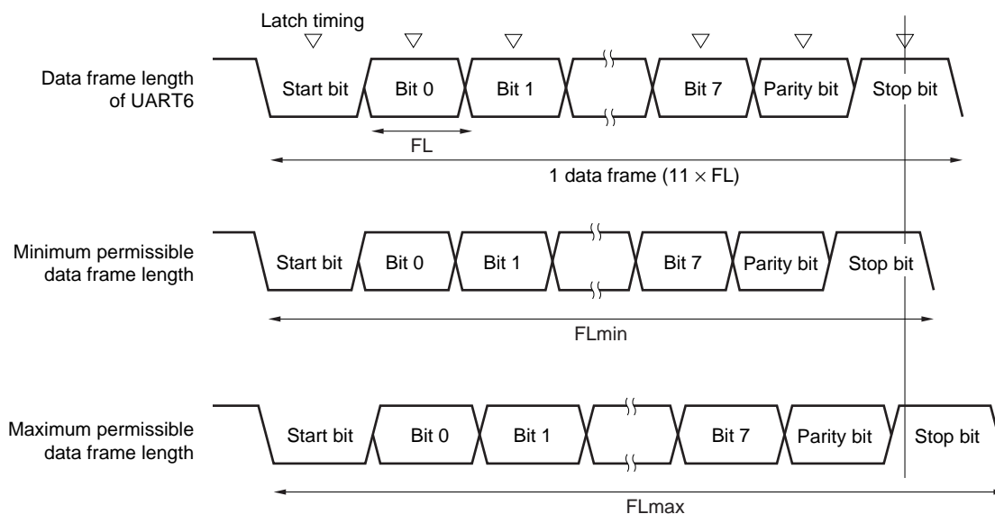
Figure 14-27. Permissible Baud Rate Range During Reception
