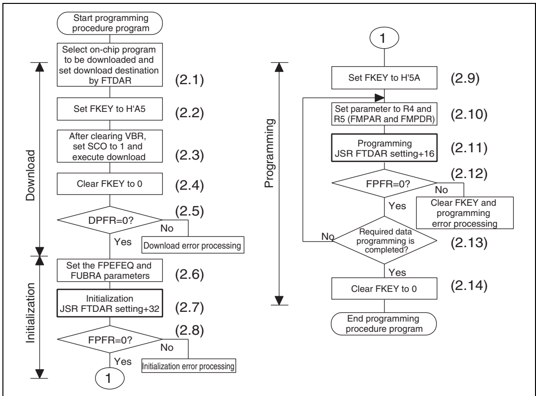
Figure 22.11 Programming Procedure
