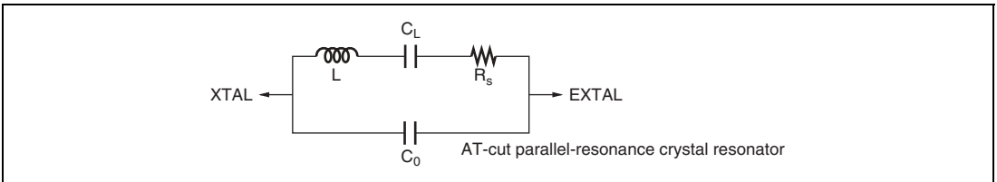
Figure 22.3 Equivalent Circuit of Crystal Resonator
