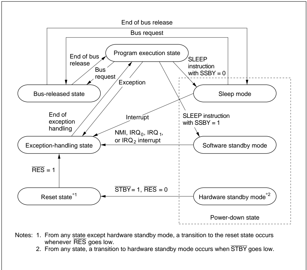
Figure 2-13 State Transitions
