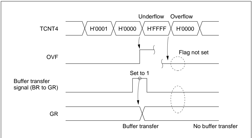
Figure 10-38 Undershoot Timing
