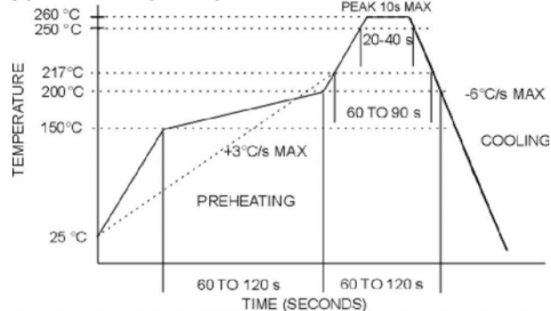
SOLDER REFLOW PROFILE
