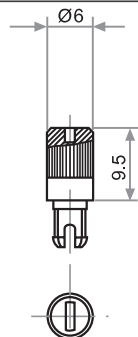
Fig. 28 - Ref. 6055
