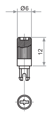
Fig. 4 - Ref. 5371
