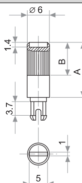
Fig. 18 - Ref. 5271
