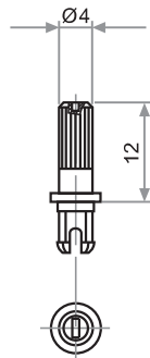
Fig. 21 - Ref. 6031*
