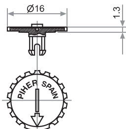
Fig. 4 - Ref. 5371
