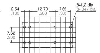
2 coil latching type
