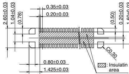
Recommended metal mask pattern Metal mask thickness: When 100μm (Terminal opening ratio: 70%) (Metal-part opening ratio: 100%)
