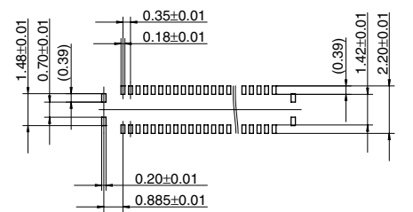
Recommended metal mask pattern Metal mask thickness: When 100μm (Terminal opening ratio: 70%) (Metal-part opening ratio: 100%)
