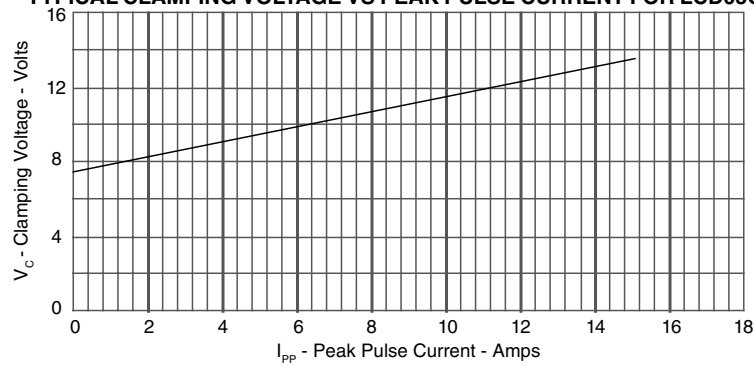
FIGURE 5 TYPICAL CLAMPING VOLTAGE VS PEAK PULSE CURRENT FOR LCD05C
