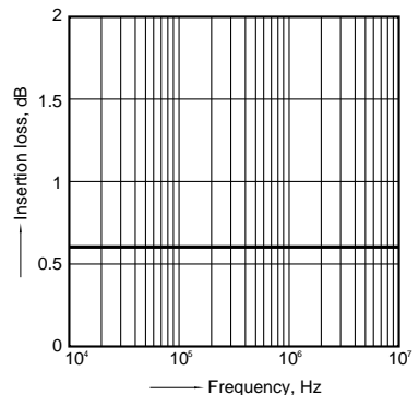
15. Insertion loss vs. frequency characteristics (50Ω impedance)
