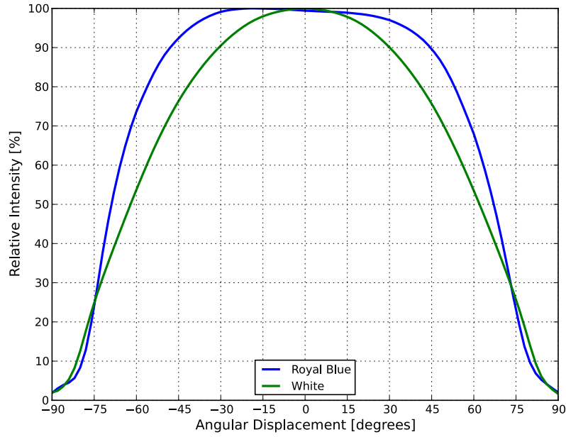
Figure 12. Typical representative spatial radiation pattern.
