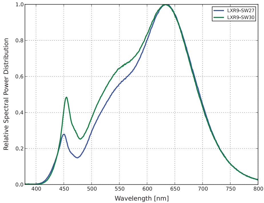
Figure 7. Color spectrum of LXR9-SWxx emitter, integrated measurement.
