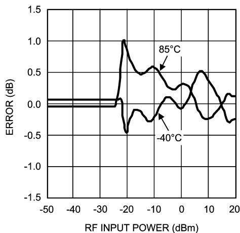
Output Variation vs. RF Input Power Normalized to 25^\circ C @ 1900 MHz (LMV226)
