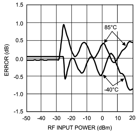
Output Variation vs. RF Input Power Normalized to 25^\circ C @ 1800 MHz (LMV228 in microSMD)
