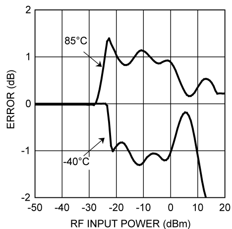
Output Variation vs. RF Input Power Normalized to 25°C @ 1800 MHz (LMV228 in LLP)
