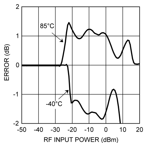
Output Variation vs. RF Input Power Normalized to 25°C @ 2000 MHz (LMV228 in LLP)
