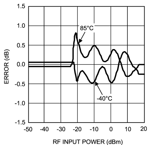
Output Variation vs. RF Input Power Normalized to 25^\circ C @ 1900 MHz (LMV226)
