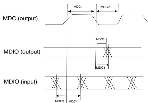
Figure 54. MII/RMII serial management channel timing
