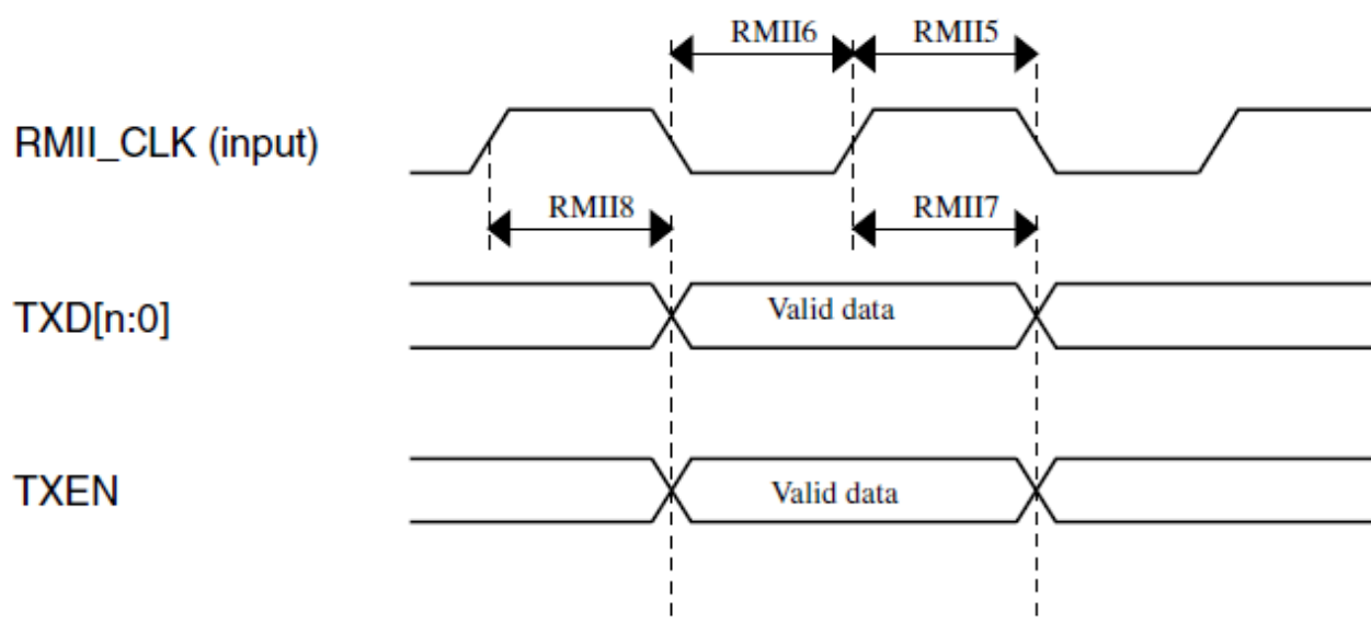
Figure 51. RMI transmit diagram
