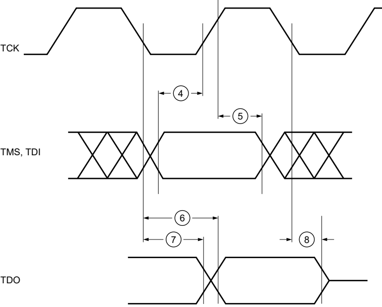
Figure 63. JTAG Test Access Port Timing
