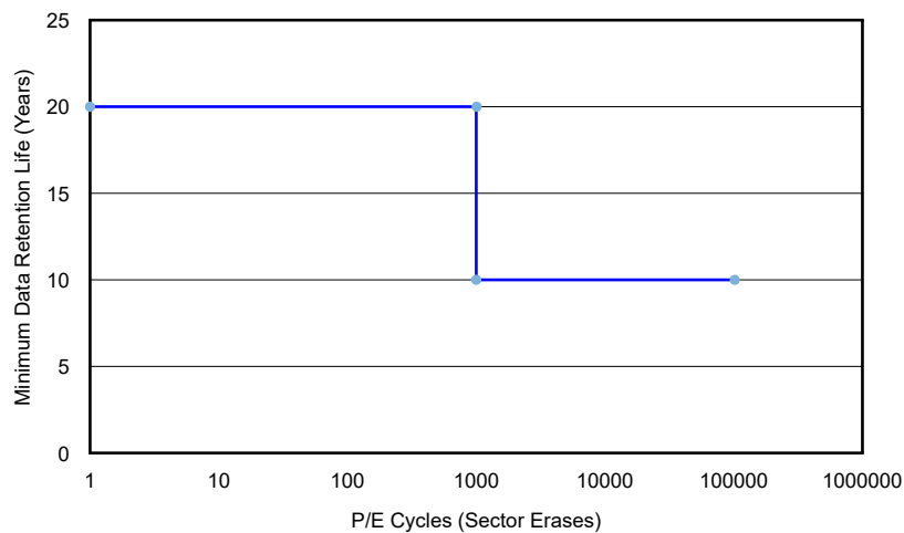
Figure 32. Data retention vs program/erase cycles
