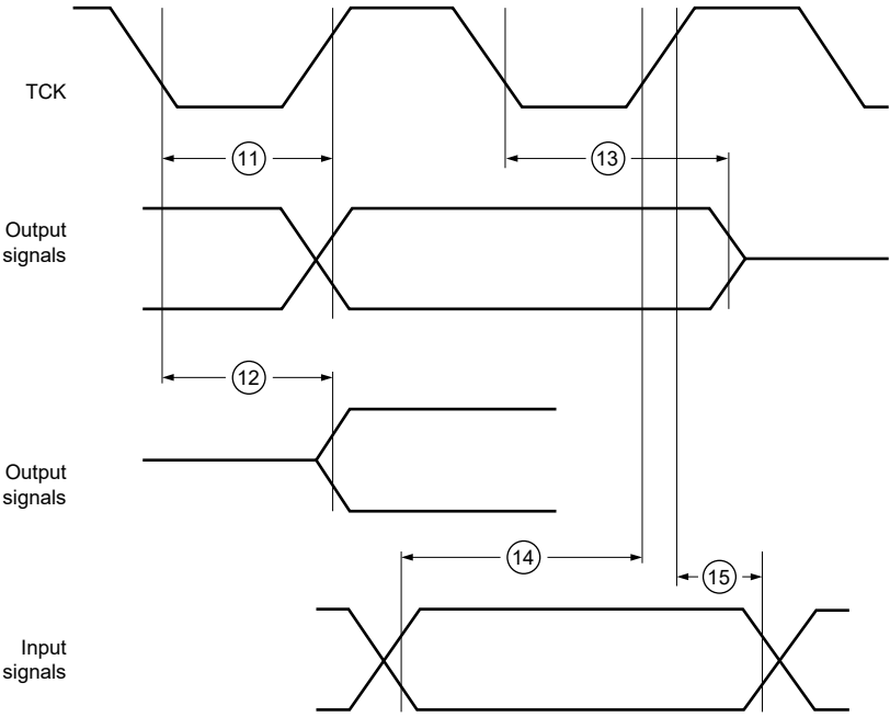
Figure 64. Boundary Scan Timing
