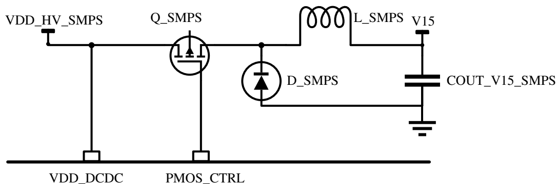
Figure 28. SMPS circuit
