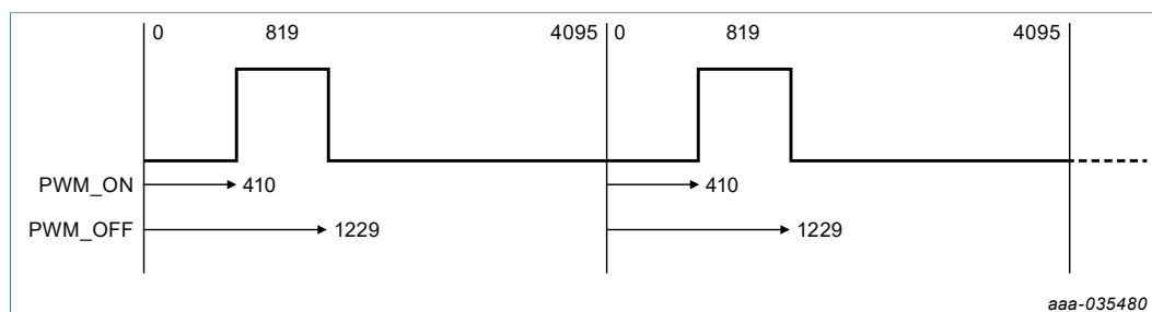
Figure 12. Pulse Width Modulation Example
