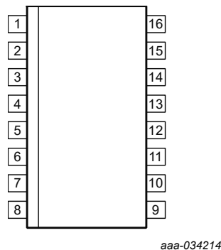
Figure 4. Pin configuration for TSSOP16 package
