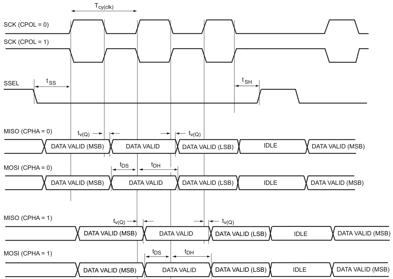
Fig 16. SPI slave interface timings
