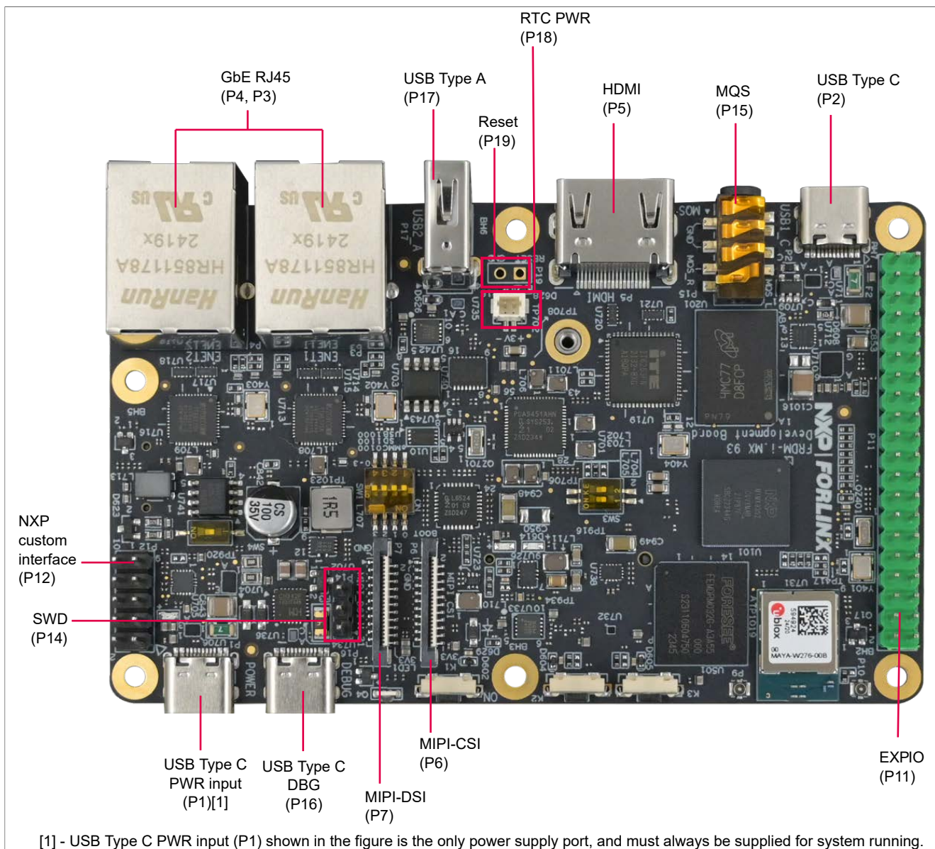
Figure 3. FRDM-IMX93 connectors
