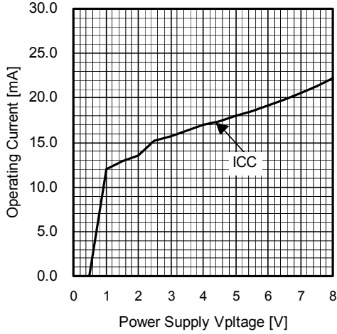
Operating Current vs. Power Supply VpItage Ta=25°C
