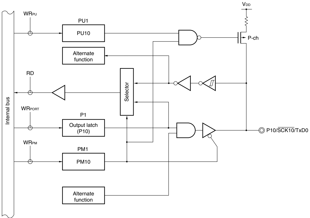
Figure 5-4. Block Diagram of P10
