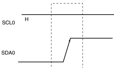
Figure 15-17. Stop Condition
