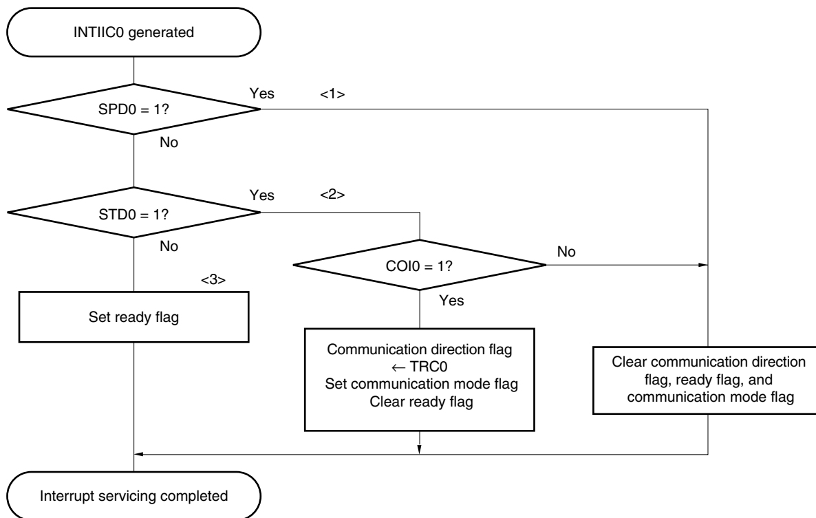
Figure 15-26. Slave Operation Flowchart (2)
