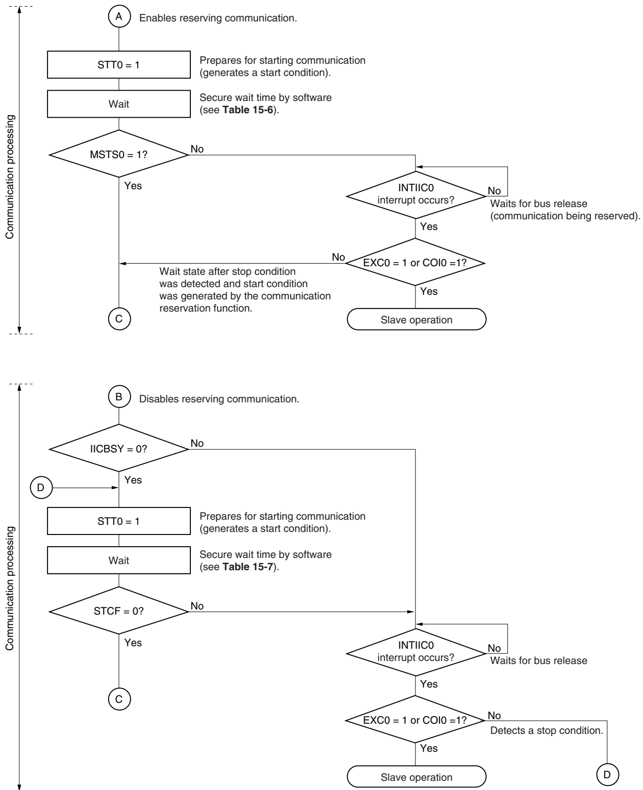
Figure 15-24. Master Operation in Multi-Master System (2/3)
