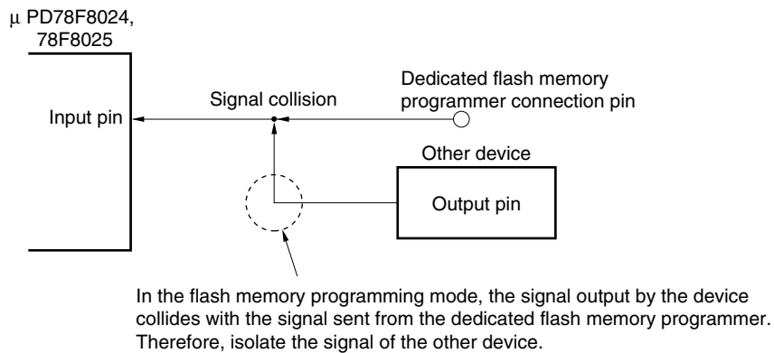
Figure 22-6. Signal Collision (Input Pin of Serial Interface)
