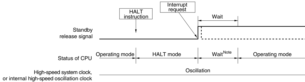
Figure 17-3. HALT Mode Release by Interrupt Request Generation
