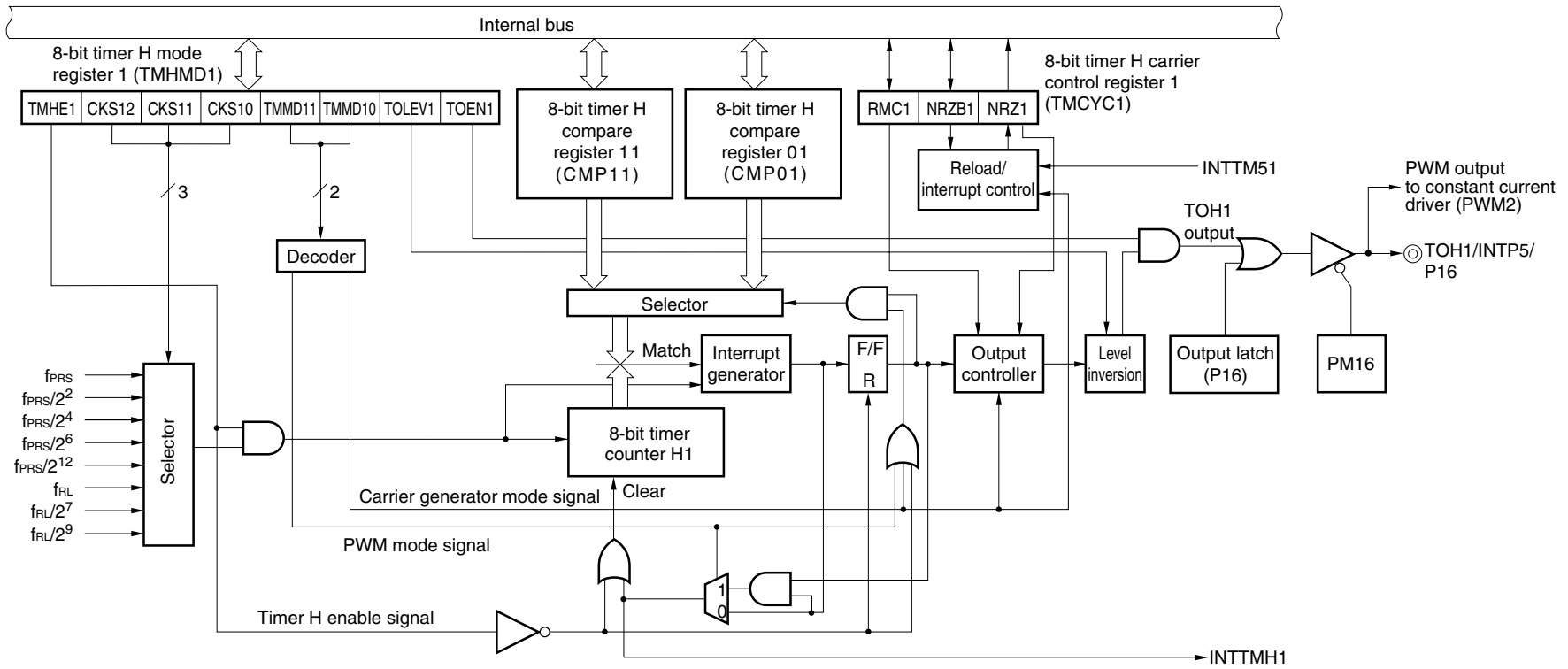
Figure 9-2. Block Diagram of 8-bit Timer H1
