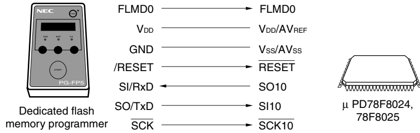
Figure 22-3. Communication with Dedicated Flash Memory Programmer (CSI10)
