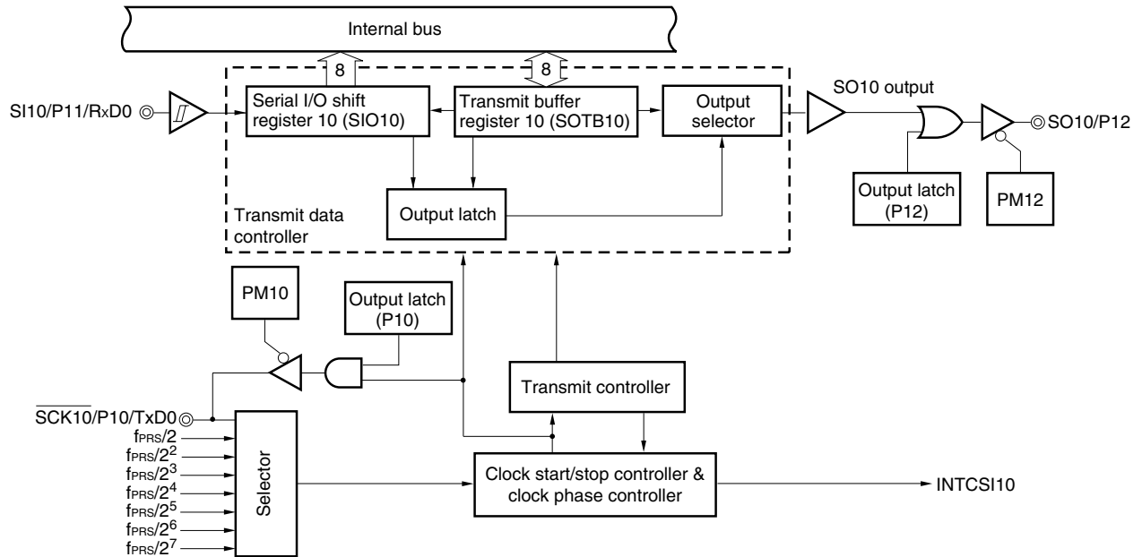
Figure 14-1. Block Diagram of Serial Interface CSI10
