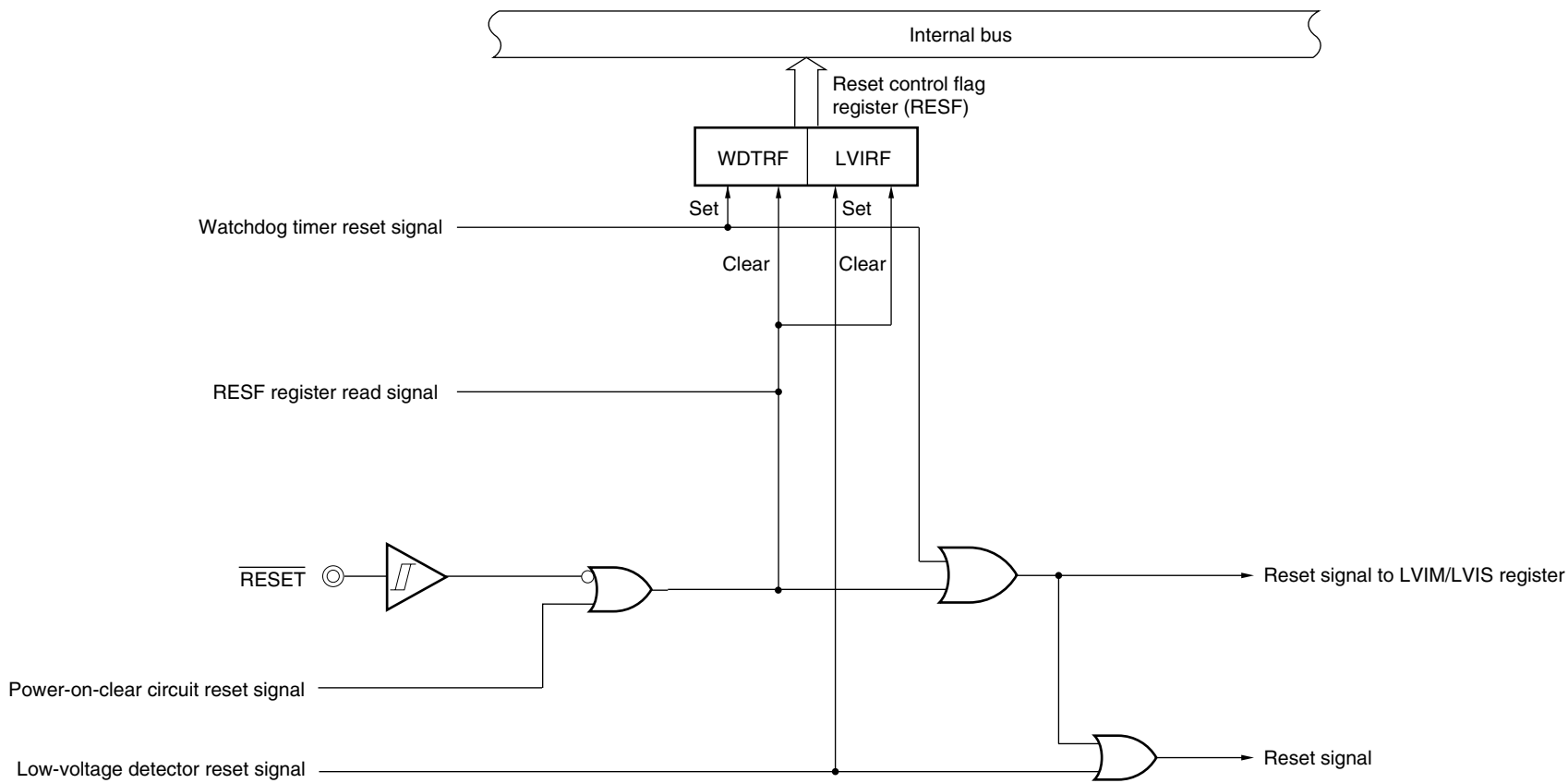
&lt;R&gt; Figure 18-1. Block Diagram of Reset Function
