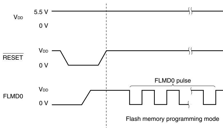
Figure 21-12. Flash Memory Programming Mode
