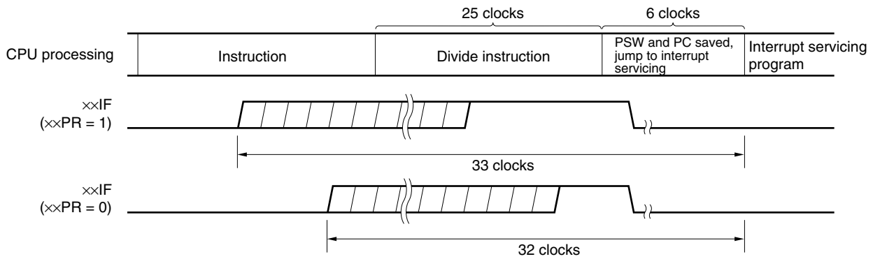
Figure 15-9. Interrupt Request Acknowledgement Timing (Maximum Time)
