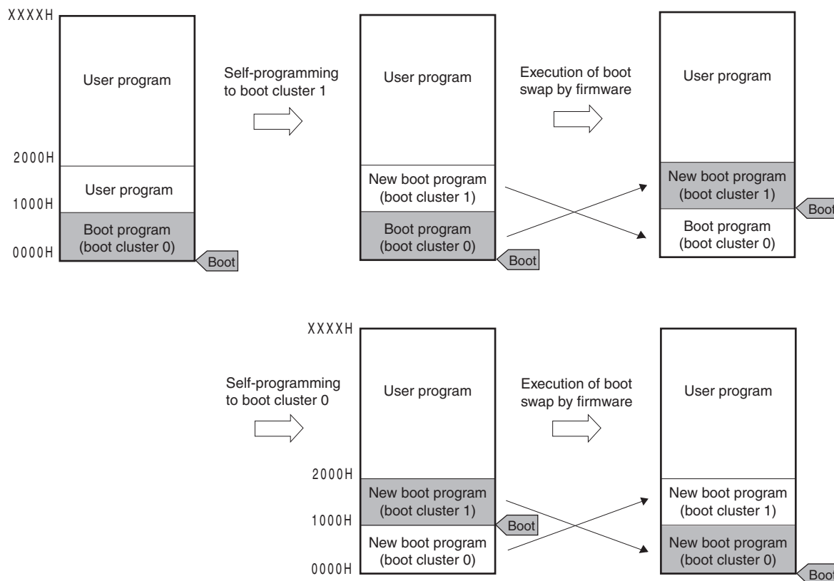
Figure 21-15. Boot Swap Function
