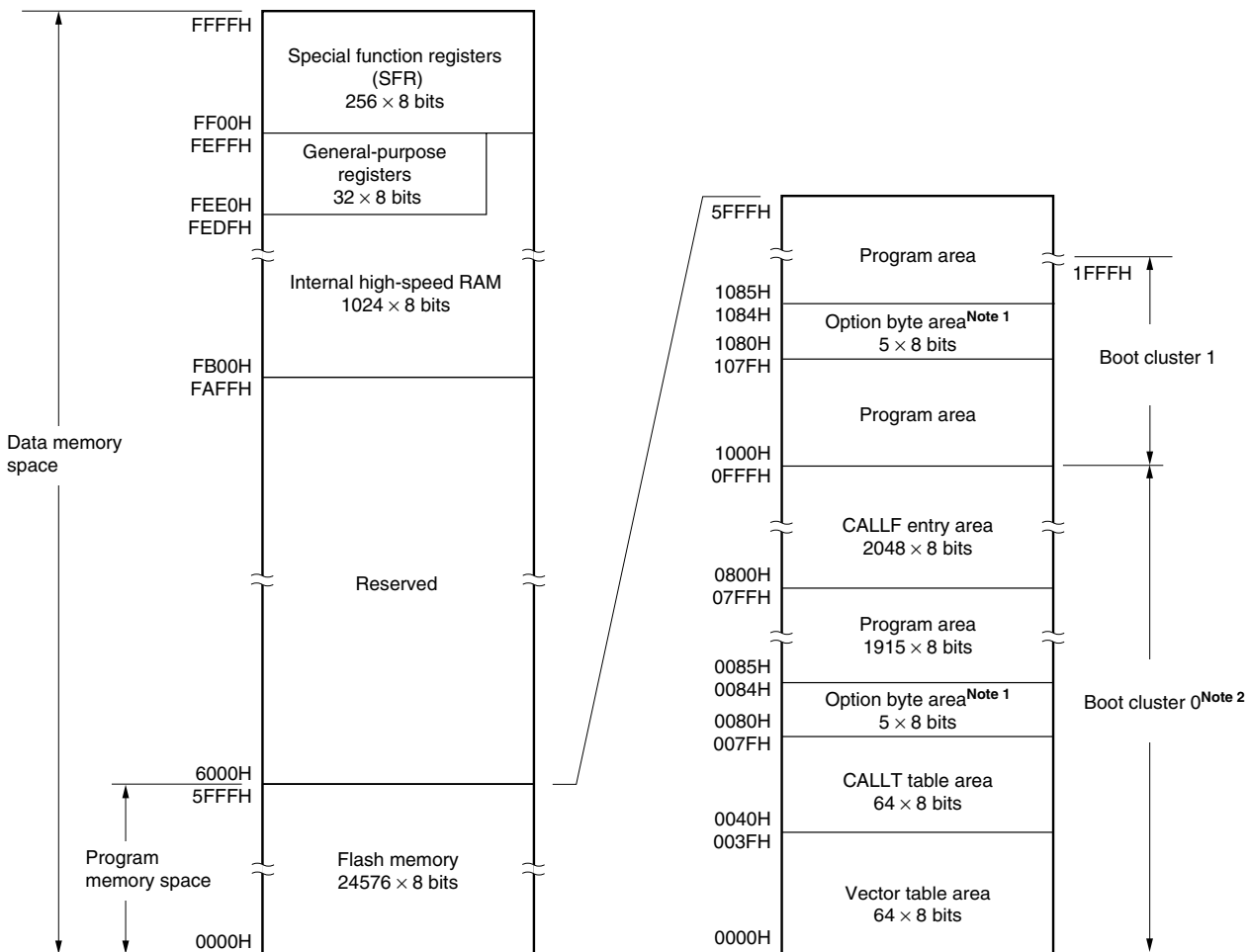
Figure 3-3. Memory Map ( \mu PD78F0502)
