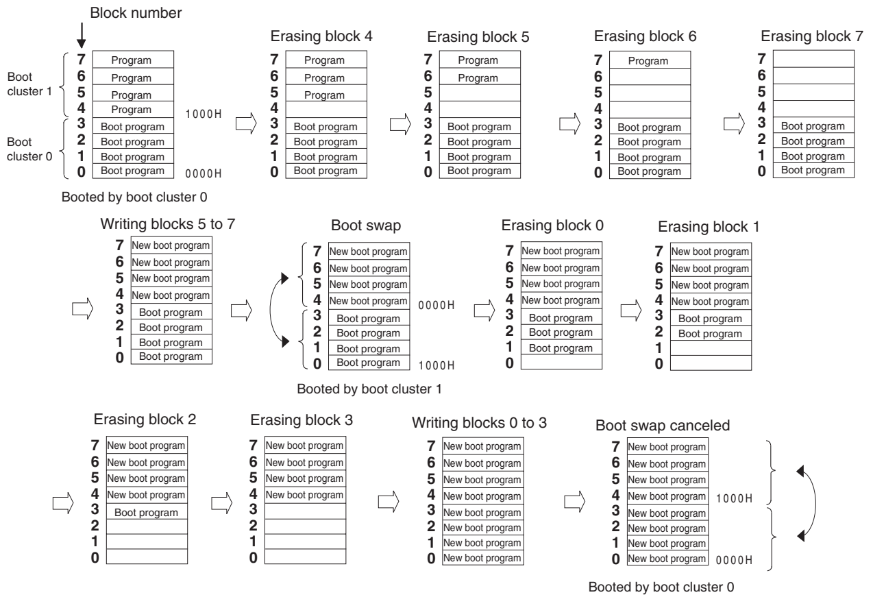
Figure 21-16. Example of Executing Boot Swapping
