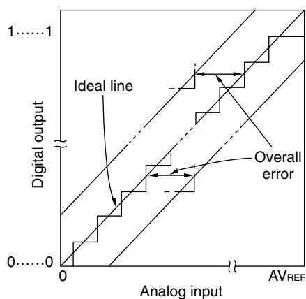
Figure 10-14. Overall Error
