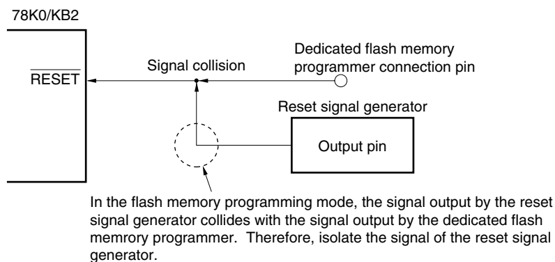
Figure 21-10. Signal Collision ( \overline{\text{RESET}} Pin)
