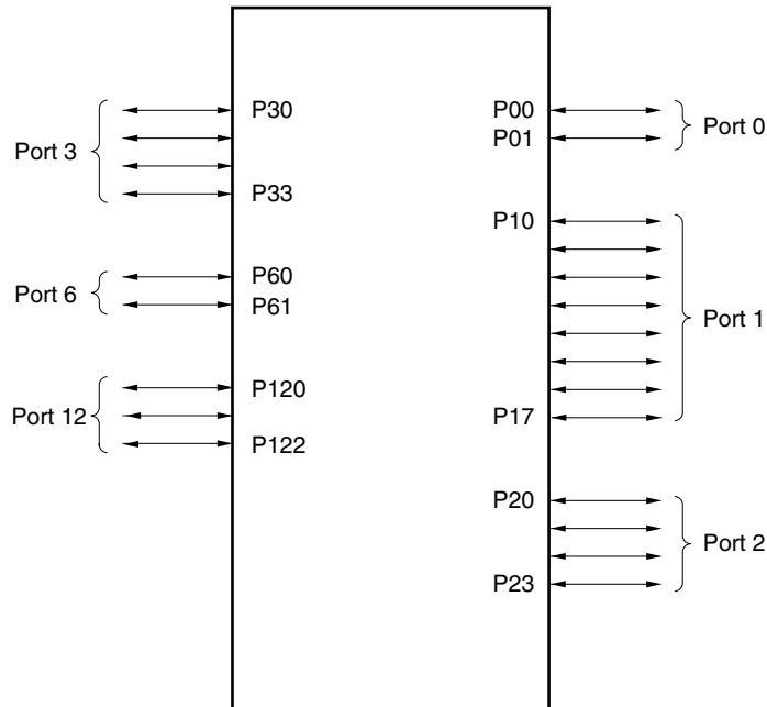
Figure 4-1. Port Types
