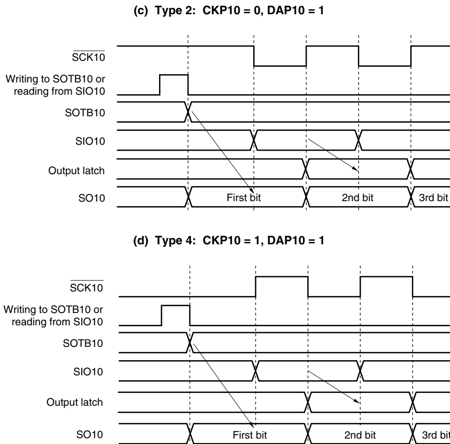
Figure 13-7. Output Operation of First Bit (2/2)
