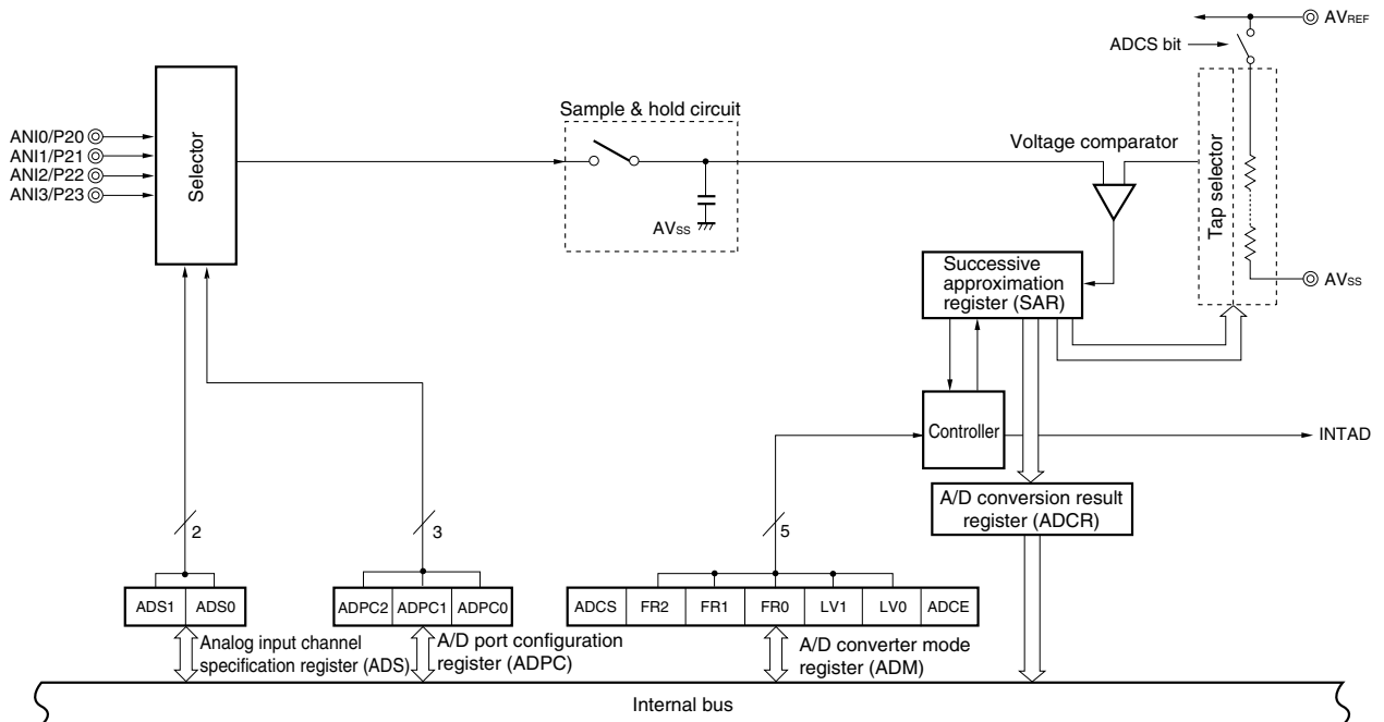
Figure 10-1. Block Diagram of A/D Converter
