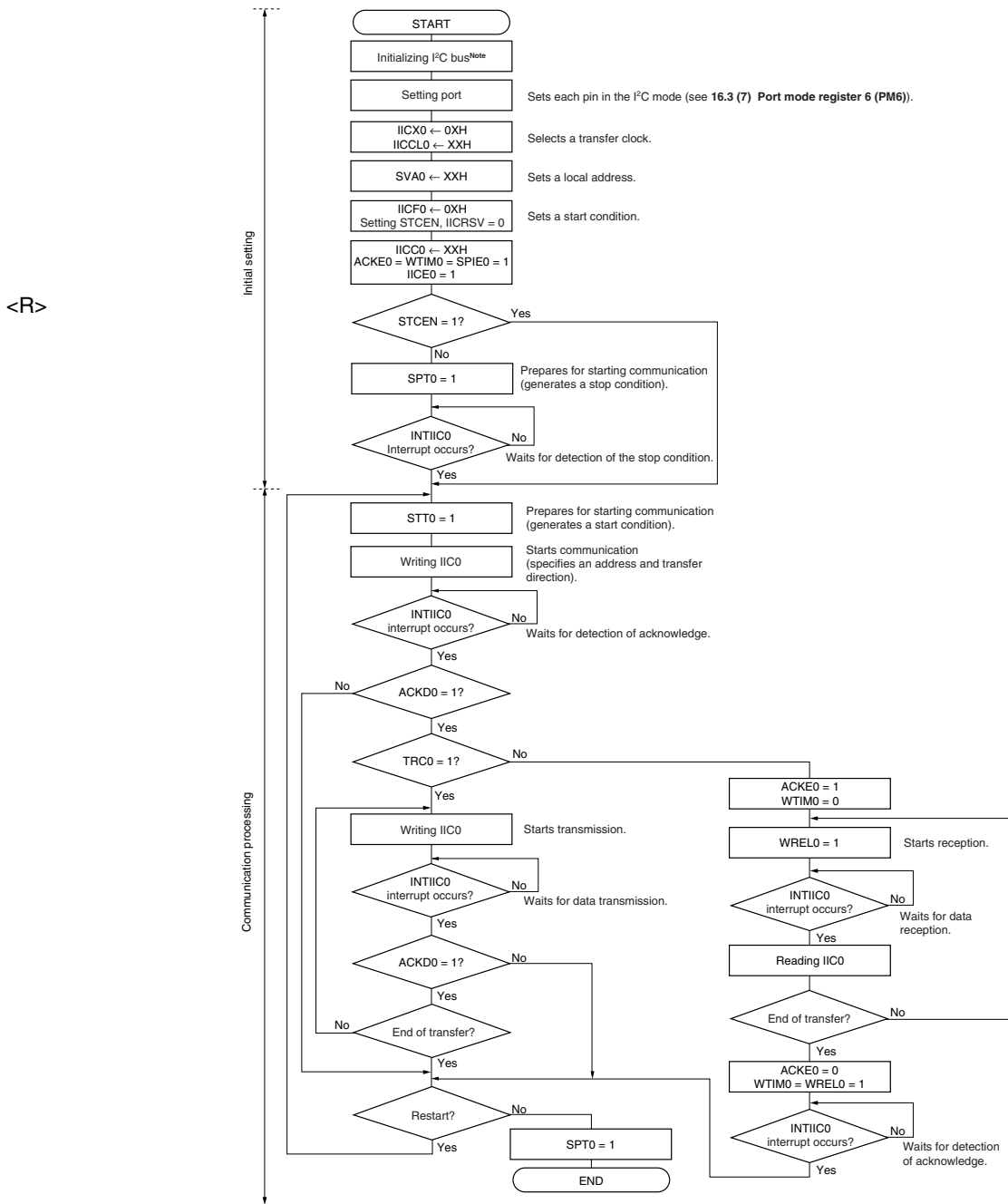
Figure 14-23. Master Operation in Single-Master System
