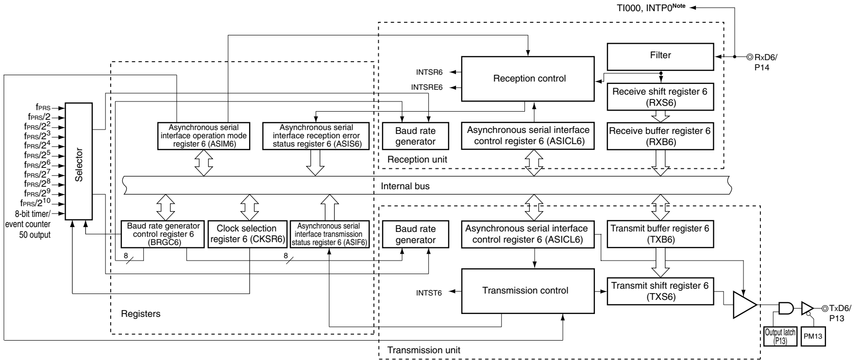
Figure 12-4. Block Diagram of Serial Interface UART6
