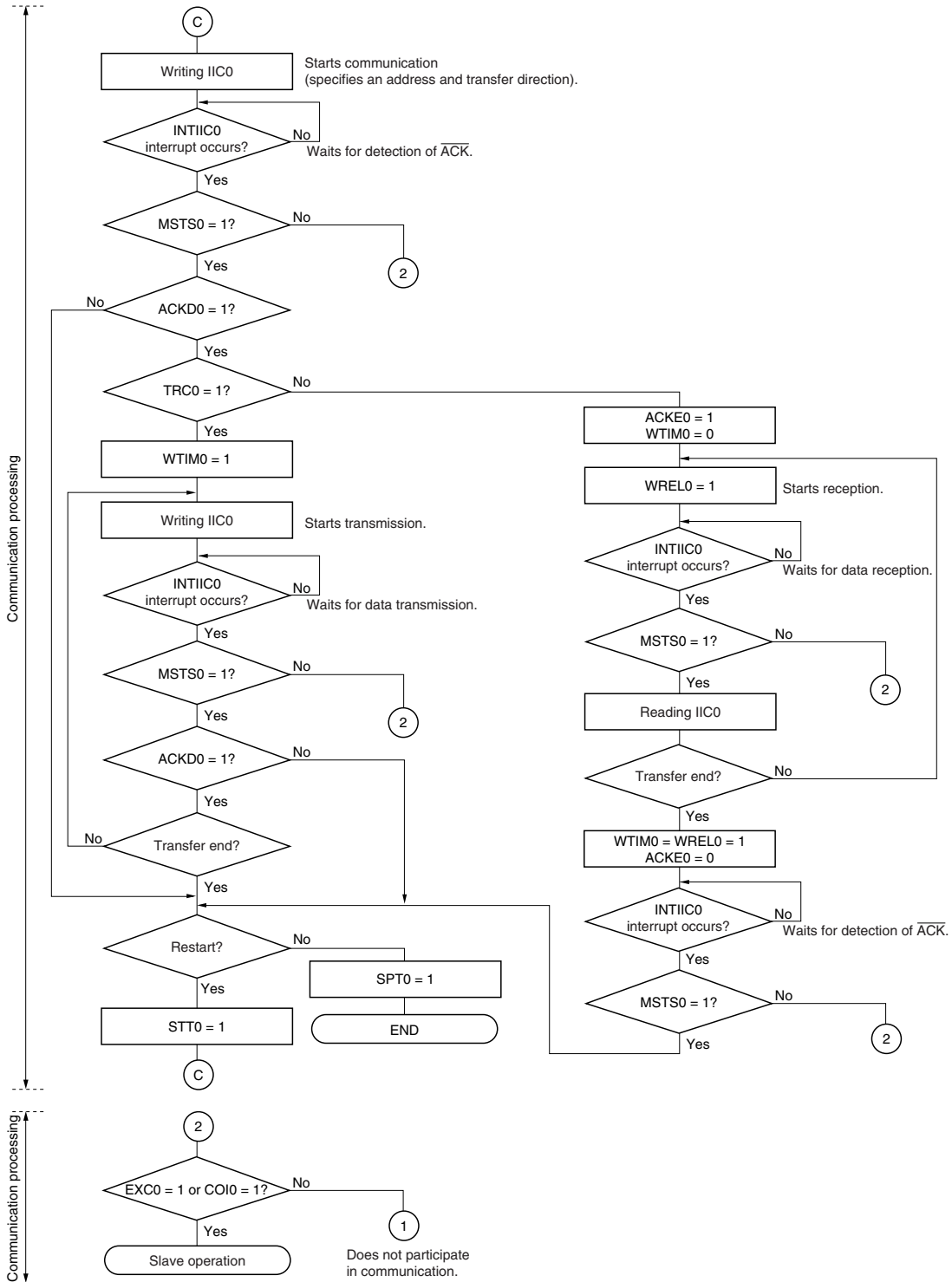
Figure 14-24. Master Operation in Multi-Master System (3/3)
