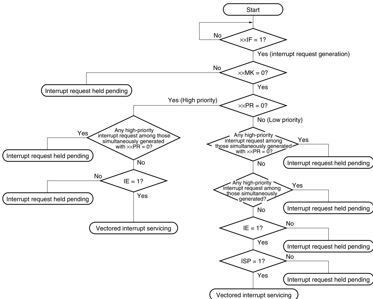
Figure 15-7. Interrupt Request Acknowledgement Processing Algorithm
