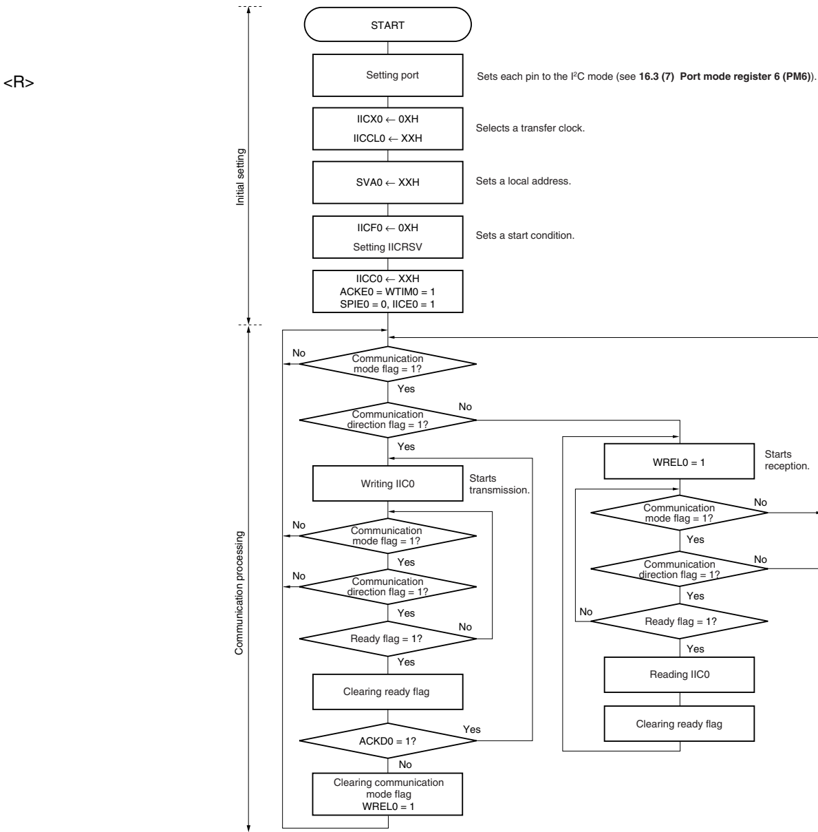
Figure 14-25. Slave Operation Flowchart (1)
