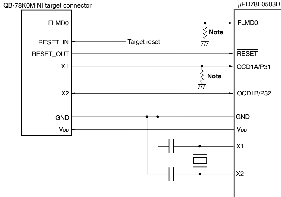
Figure 22-2. Connection Example of QB-78K0MINI and μPD78F0503D (When OCD1A/P31 and OCD1B/P32 Are Used)
