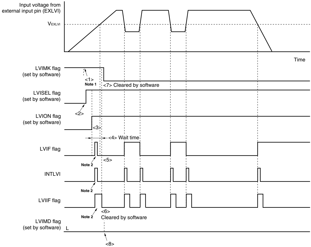
Figure 19-8. Timing of Low-Voltage Detector Interrupt Signal Generation (Detects Level of Input Voltage from External Input Pin (EXLVI))
