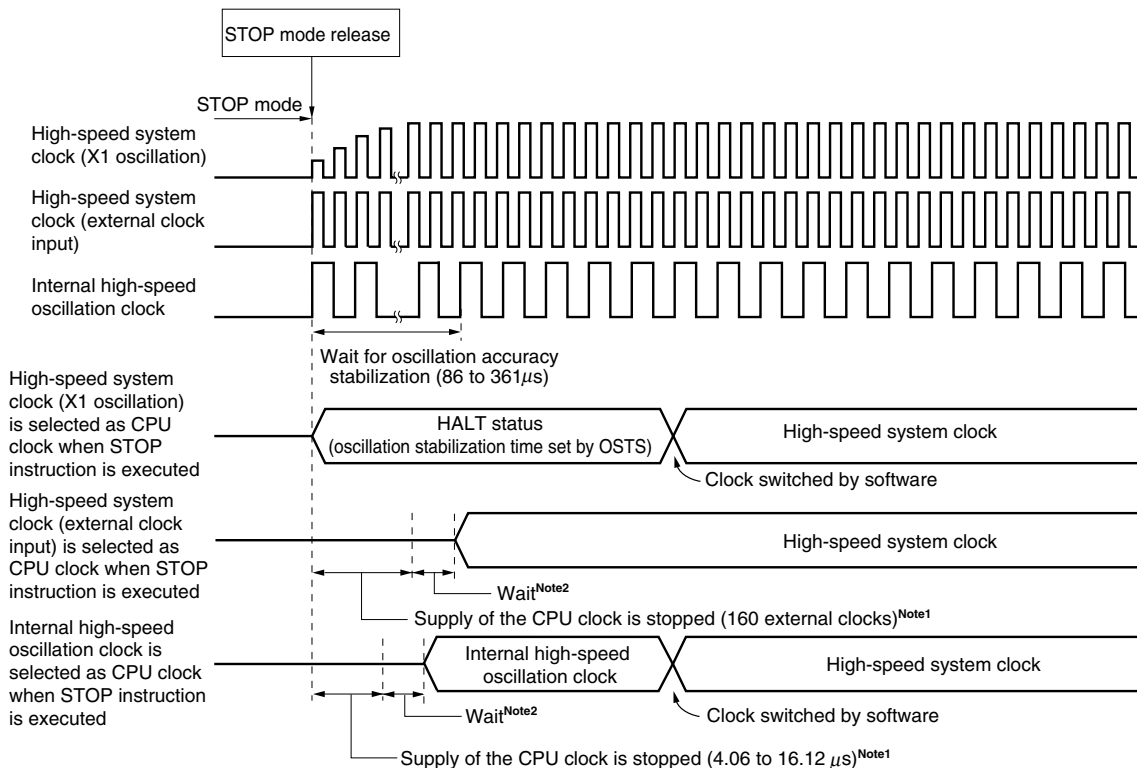
Figure 16-5. Operation Timing When STOP Mode Is Released
