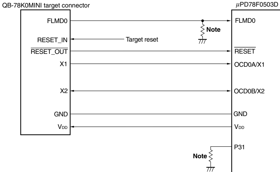
Figure 22-1. Connection Example of QB-78K0MINI and \mu PD78F0503D (When OCD0A/X1 and OCD0B/X2 Are Used)
