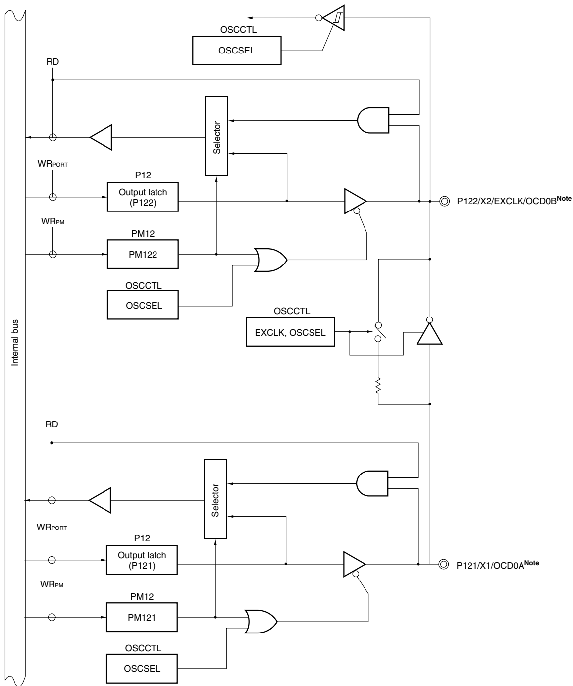
Figure 4-14. Block Diagram of P121 and P122
