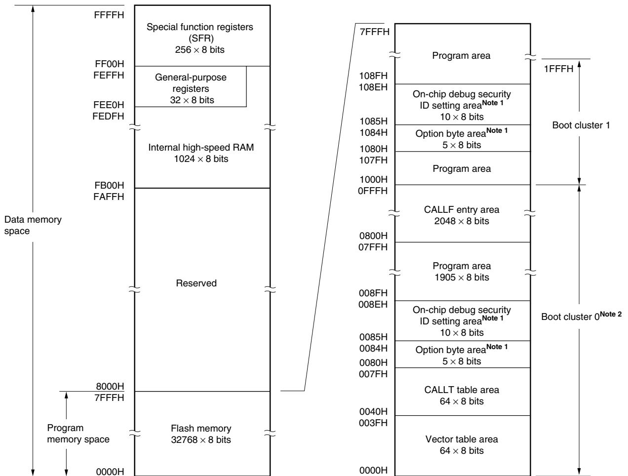
Figure 3-5. Memory Map ( \mu PD78F0503D)
