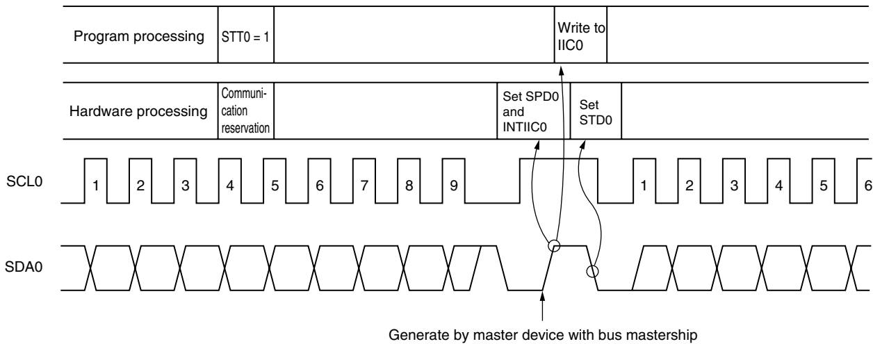
Figure 14-20. Communication Reservation Timing
