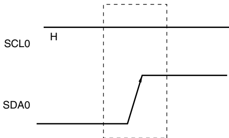
Figure 14-17. Stop Condition
