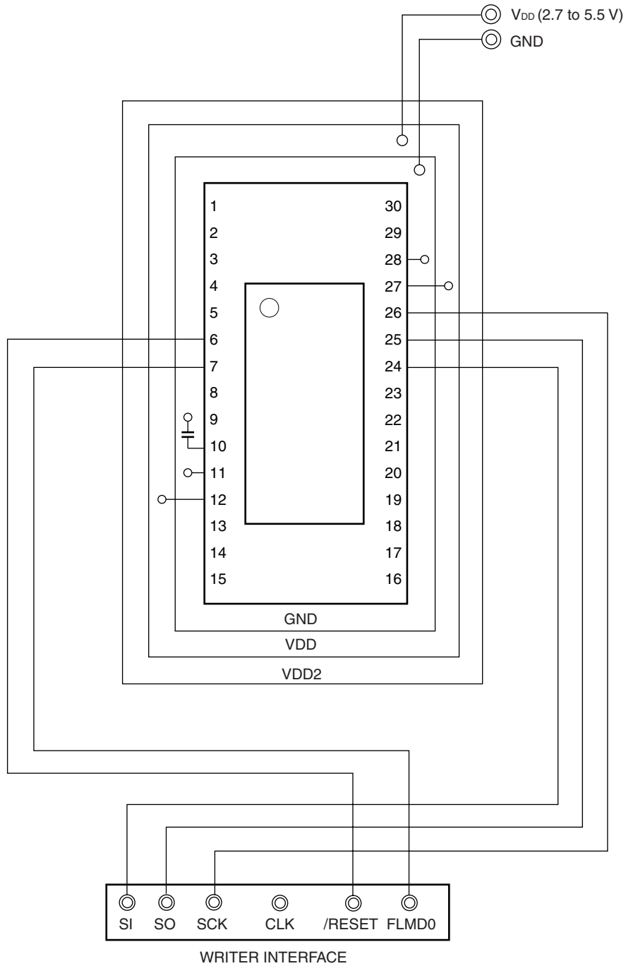
Figure 21-2. Example of Wiring Adapter for Flash Memory Writing in 3-Wire Serial I/O (CSI10) Mode (30-pin Plastic SSOP (MC-5A4 and MC-CAB Types))
