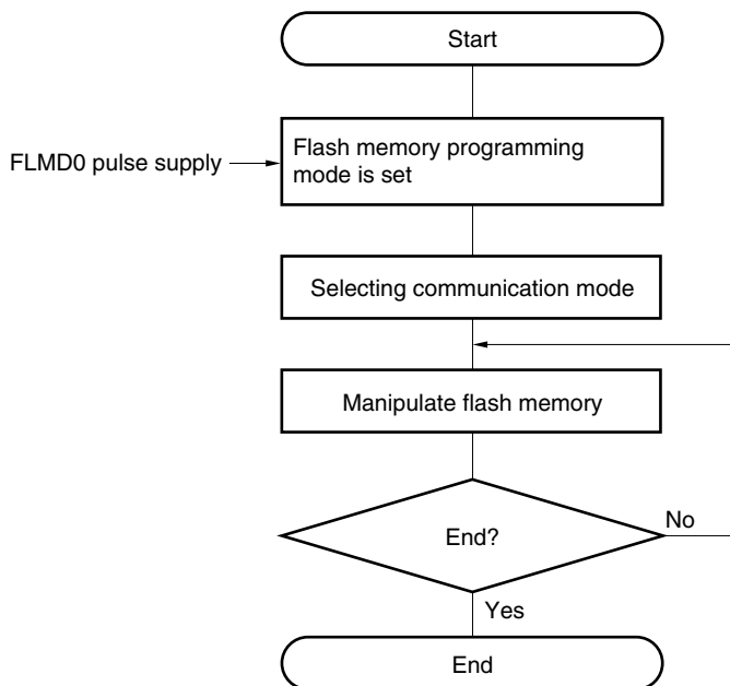
Figure 21-11. Flash Memory Manipulation Procedure
