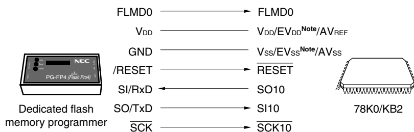
Figure 21-5. Communication with Dedicated Flash Memory Programmer (CSI10)
