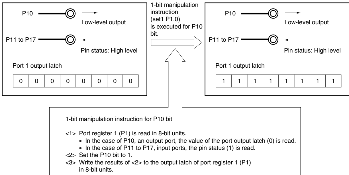
Figure 4-19. Bit Manipulation Instruction (P10)
