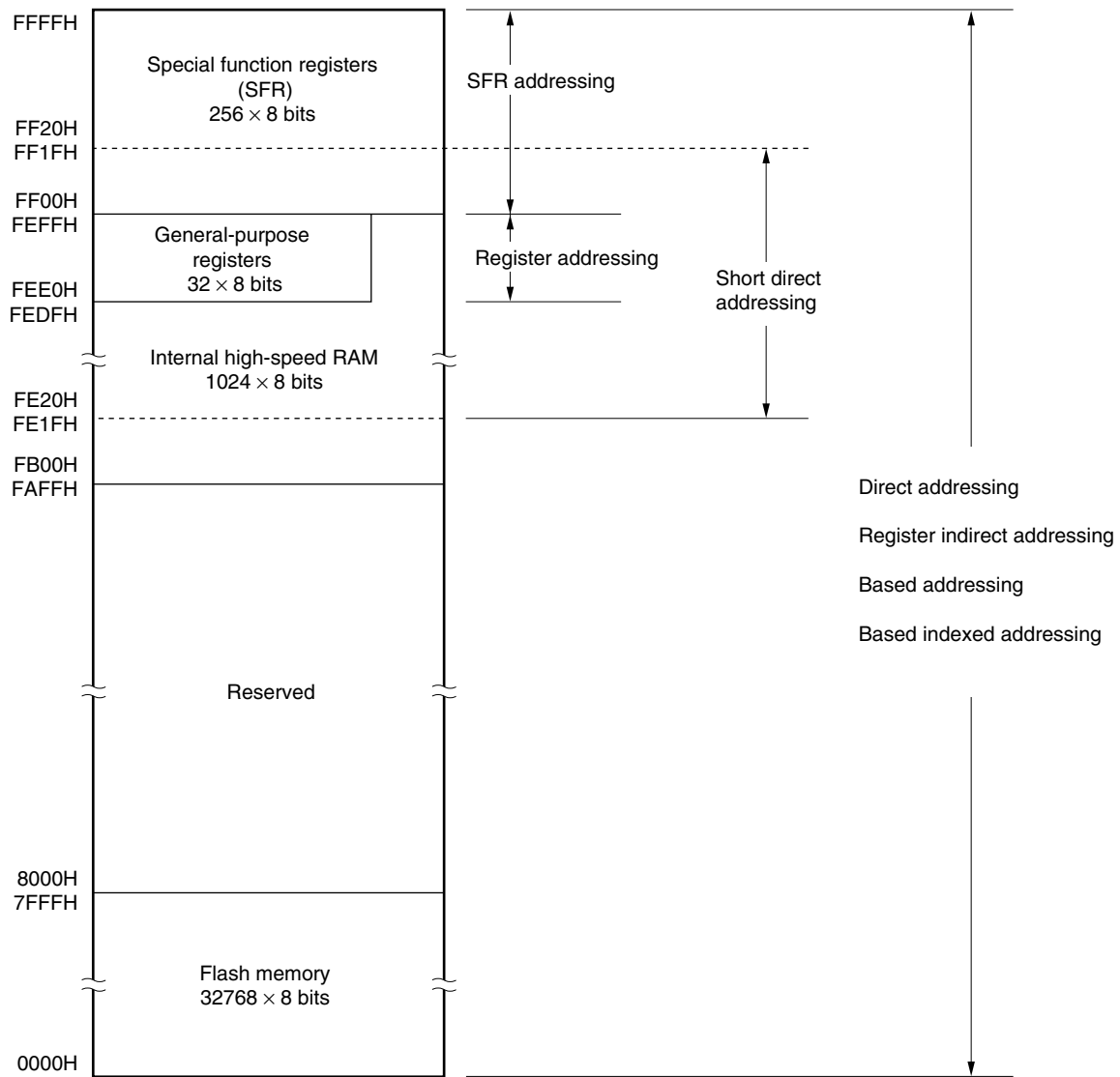
Figure 3-9. Correspondence Between Data Memory and Addressing ( \mu PD78F0503, 78F0503D)
