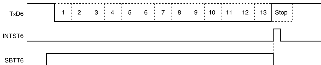
Figure 12-22. SBF Transmission
