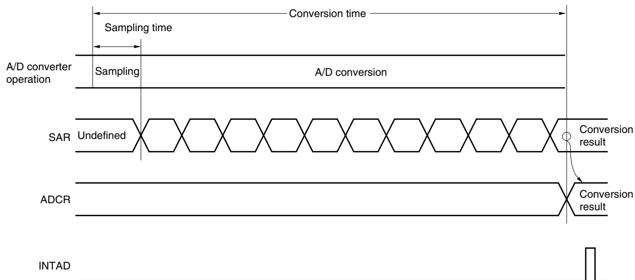
Figure 10-11. Basic Operation of A/D Converter
