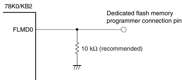
Figure 21-7. FLMD0 Pin Connection Example
