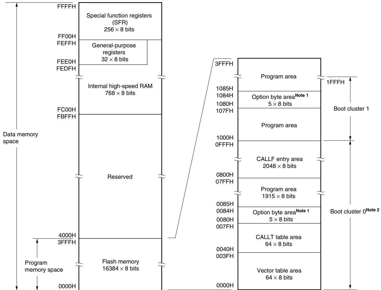
Figure 3-2. Memory Map ( \mu PD78F0501)
