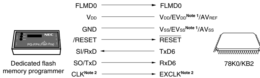
Figure 21-6. Communication with Dedicated Flash Memory Programmer (UART6)
