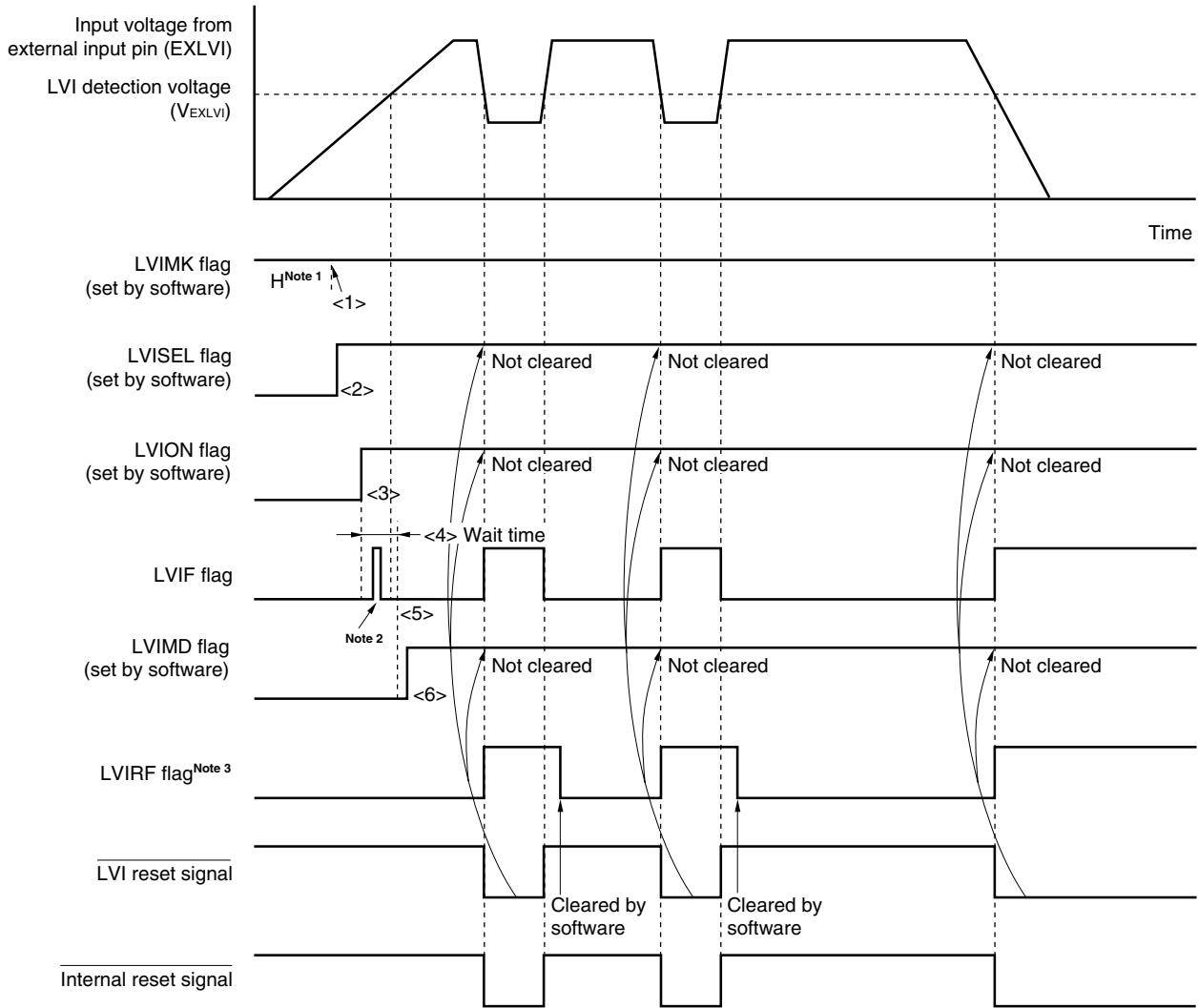
Figure 19-6. Timing of Low-Voltage Detector Internal Reset Signal Generation (Detects Level of Input Voltage from External Input Pin (EXLVI))
