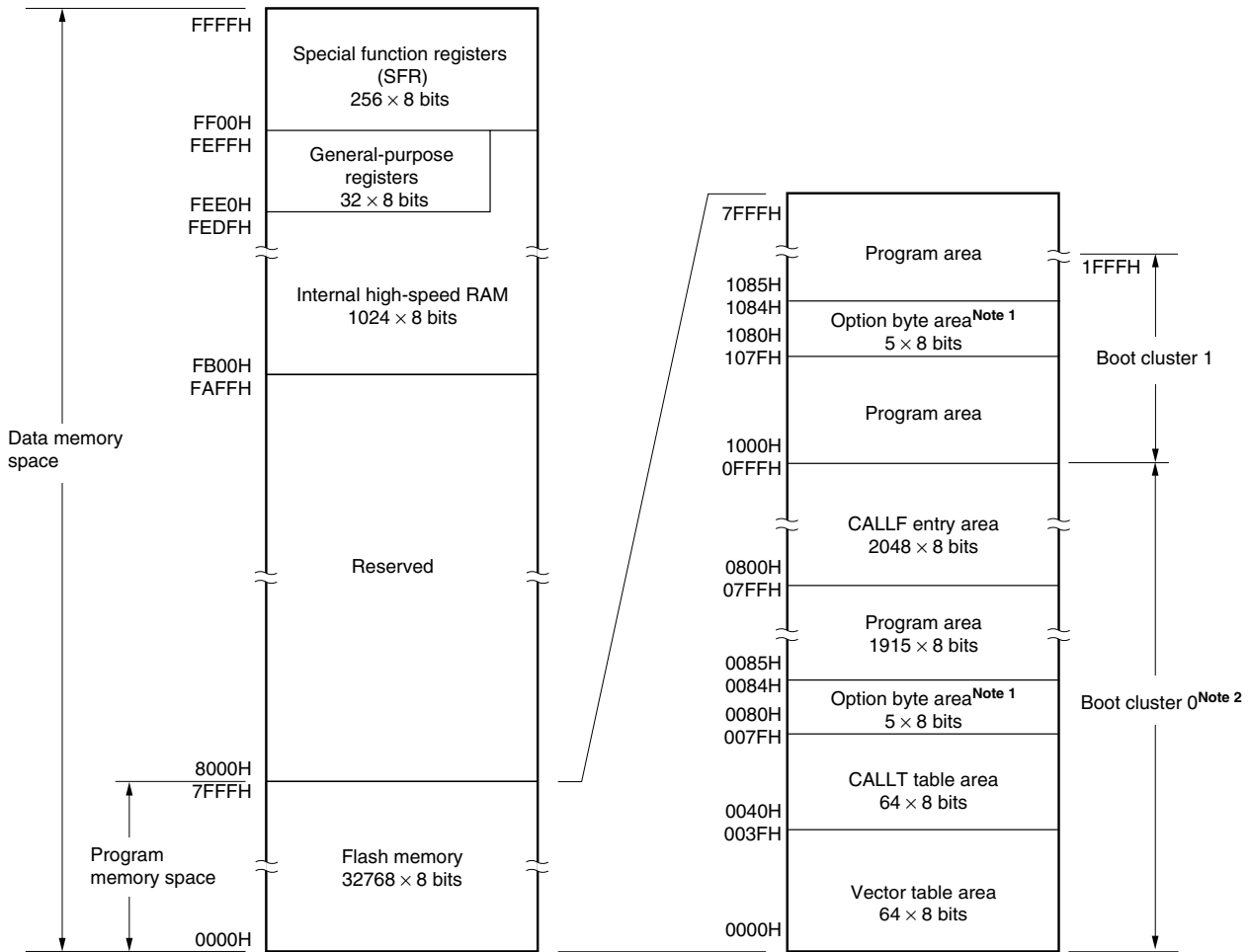
Figure 3-4. Memory Map ( \mu PD78F0503)
