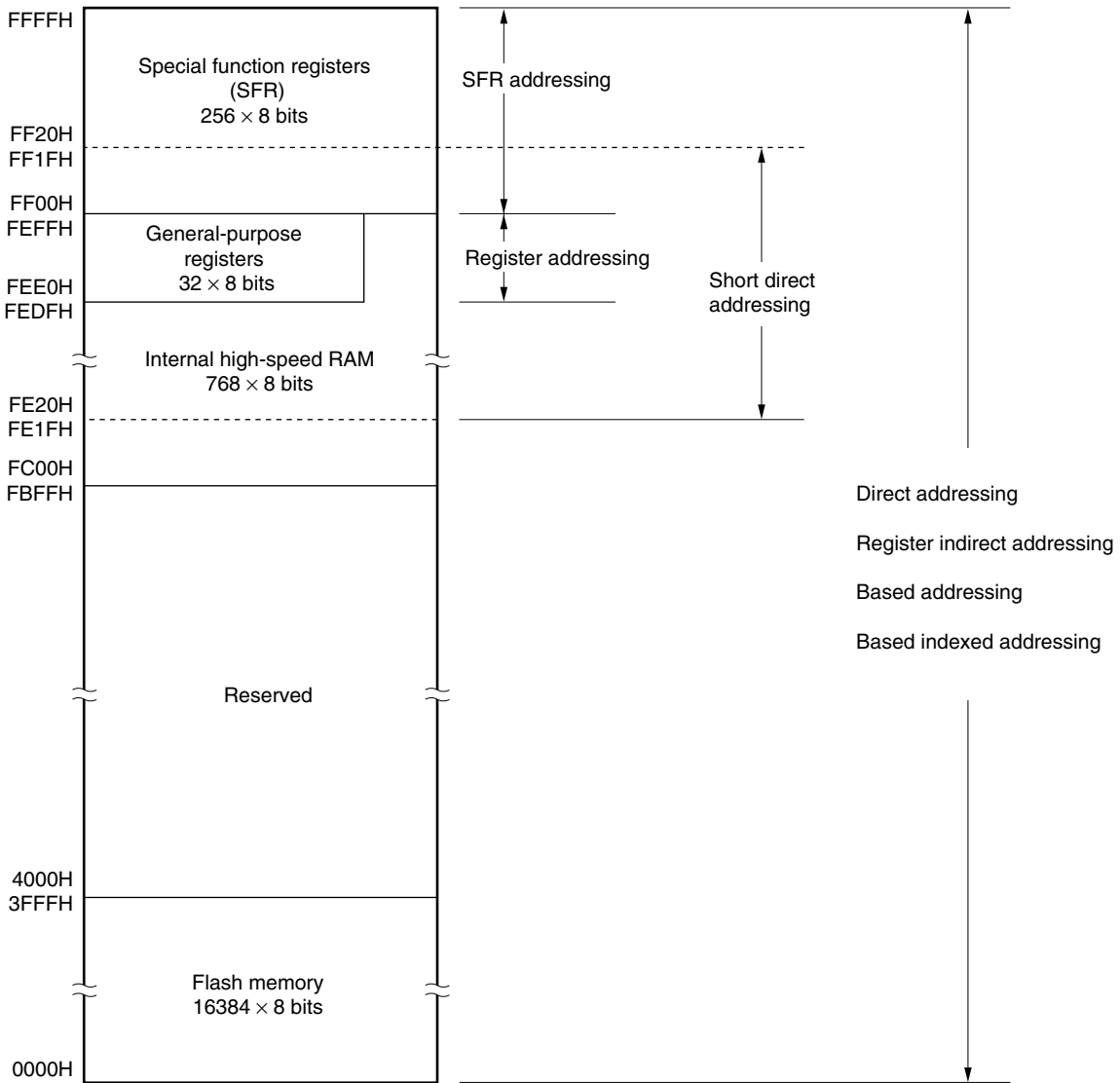
Figure 3-7. Correspondence Between Data Memory and Addressing ( \mu PD78F0501)
