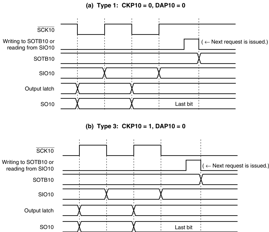
Figure 13-8. Output Value of SO10 Pin (Last Bit) (1/2)
