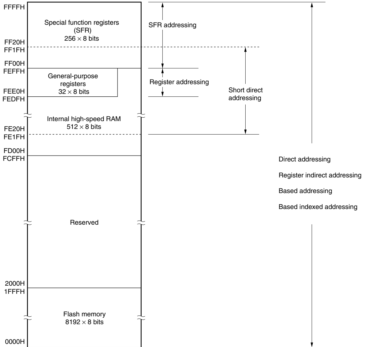
Figure 3-6. Correspondence Between Data Memory and Addressing ( \mu PD78F0500)
