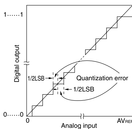
Figure 10-15. Quantization Error
