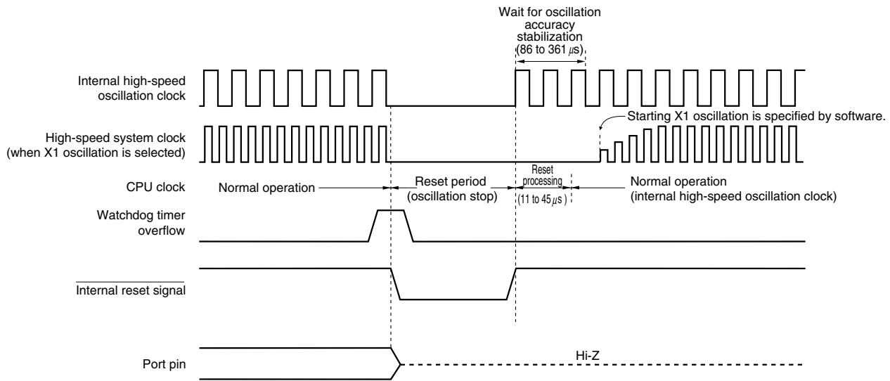
Figure 17-3. Timing of Reset Due to Watchdog Timer Overflow
