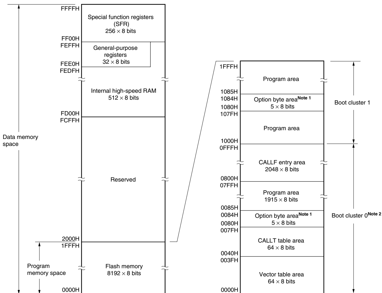
Figure 3-1. Memory Map ( \mu PD78F0500)
