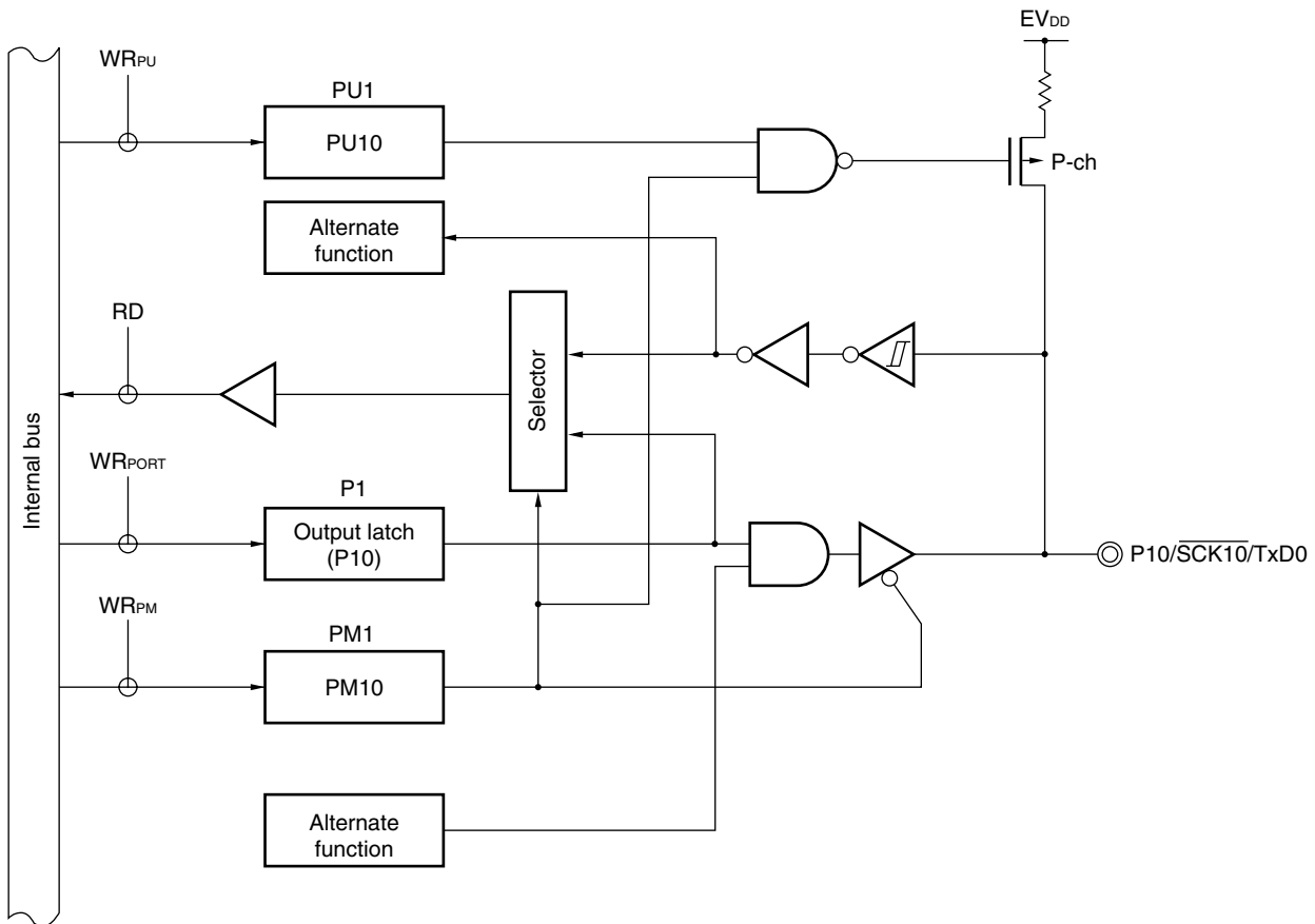
Figur 4-4. Block Diagram of P10
