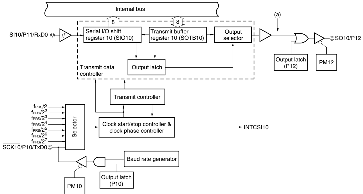
Figure 13-1. Block Diagram of Serial Interface CSI10
