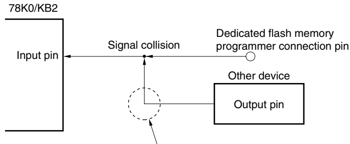
Figure 21-8. Signal Collision (Input Pin of Serial Interface)
