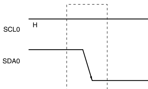
Figure 14-13. Start Conditions
