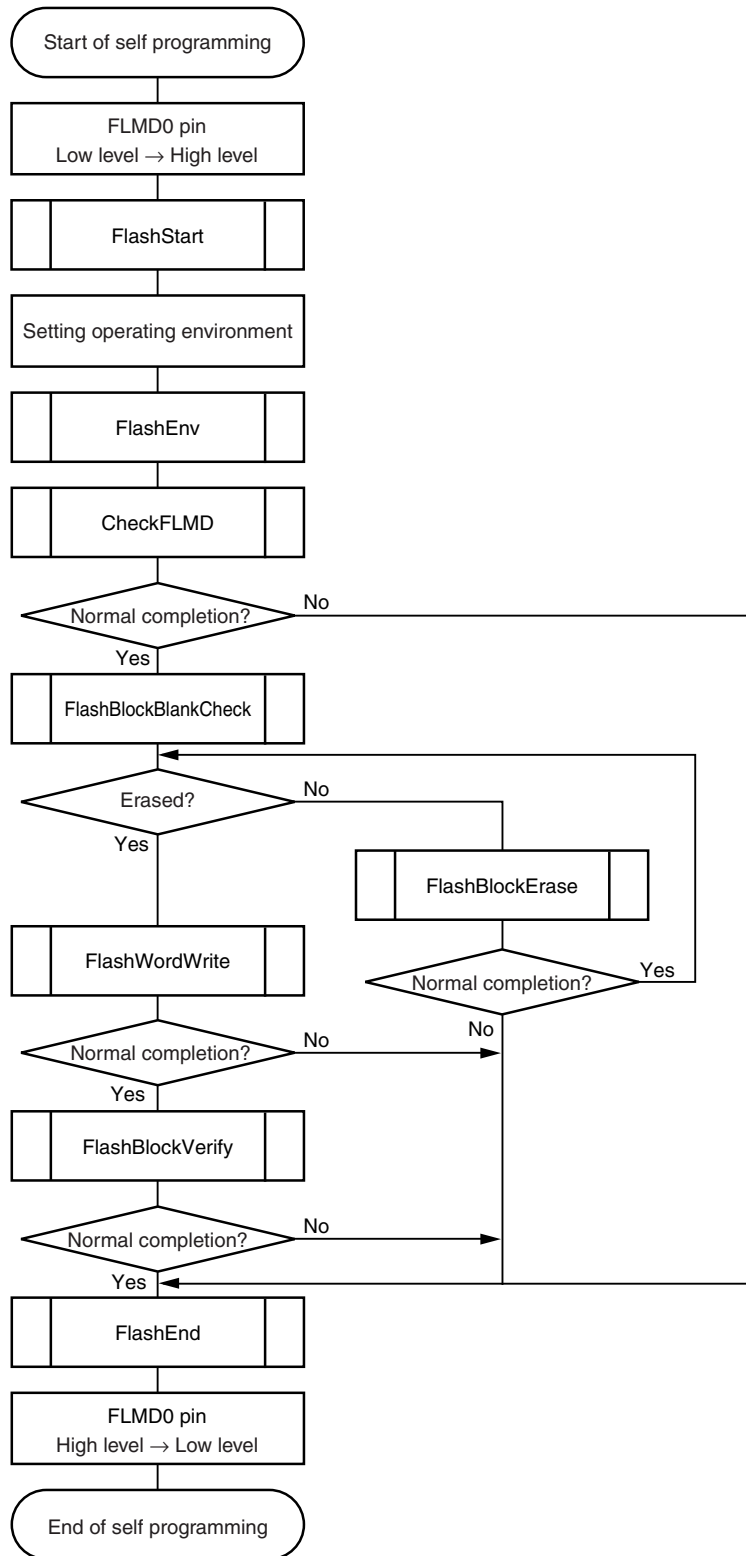
Figure 21-14. Flow of Self Programming (Rewriting Flash Memory)
