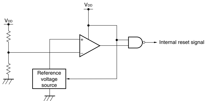
Figure 18-1. Block Diagram of Power-on-Clear Circuit
