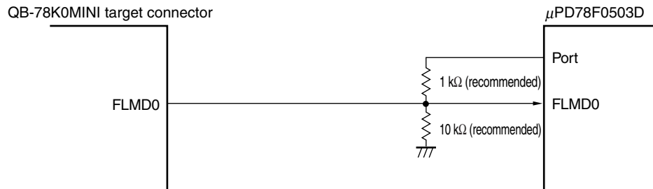
<R> Figure 22-3. Connection of FLMD0 Pin for Self Programming by Means of On-Chip Debugging
