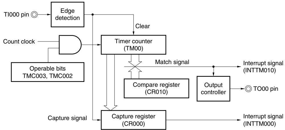
Figure 6-26. Block Diagram of Clear & Start Mode Entered by T1000 Pin Valid Edge Input (CR000: Capture Register, CR010: Compare Register)
