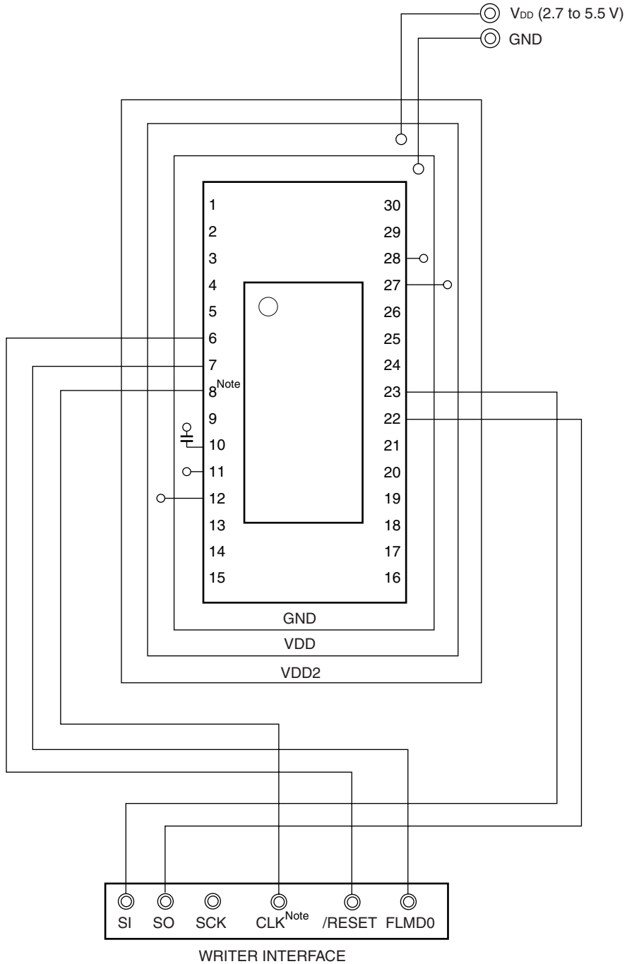
Figure 21-3. Example of Wiring Adapter for Flash Memory Writing in UART (UART6) Mode (30-pin Plastic SSOP (MC-5A4 and MC-CAB Types))
