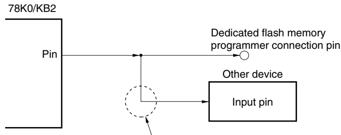
Figure 21-9. Malfunction of Other Device
