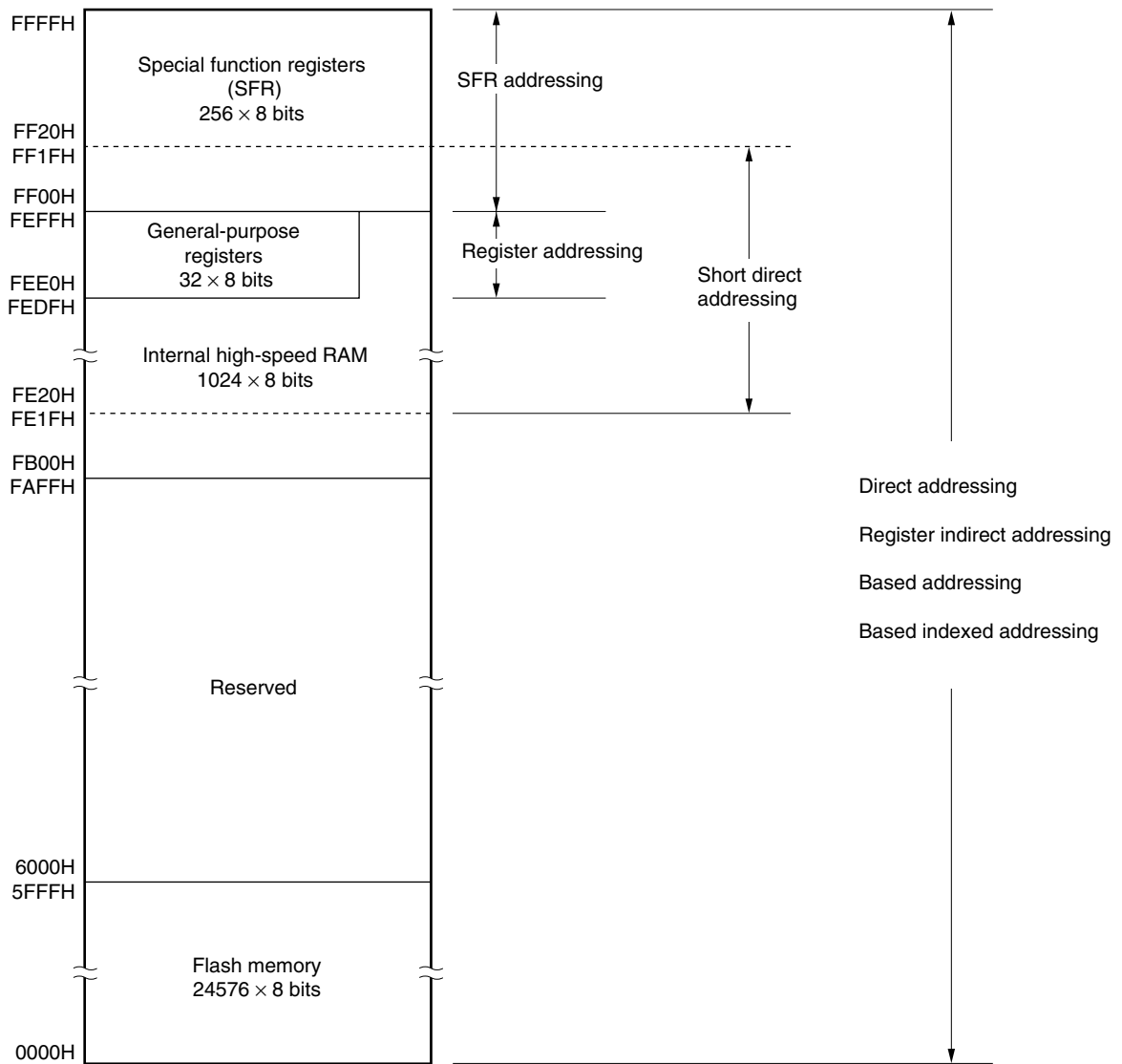
Figure 3-8. Correspondence Between Data Memory and Addressing ( \mu PD78F0502)
