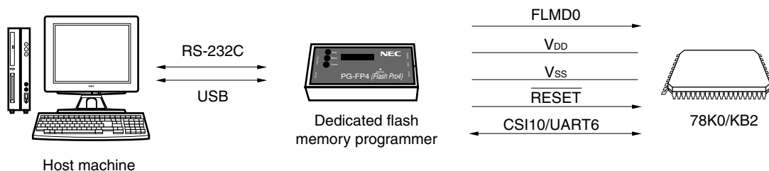
Figure 21-4. Environment for Writing Program to Flash Memory
