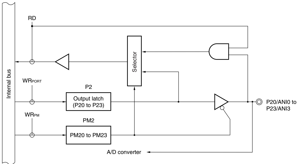
Figure 4-9. Block Diagram of P20 to P23
